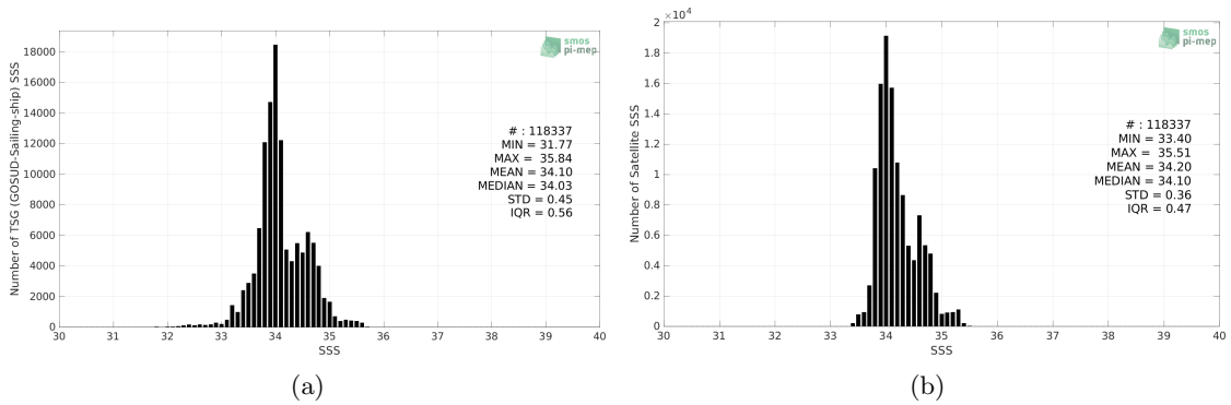
Figure 2: Histograms of SSS from TSG (GOSUD-Sailing-ship) (a) and SMAP SSS L4 OI v1 - Monthly (IPRC) (b) considering all match-up pairs per bins of 0.1 over the Roaring Forties and Furious Fifties Pi-MEP region and for the full satellite product period.
