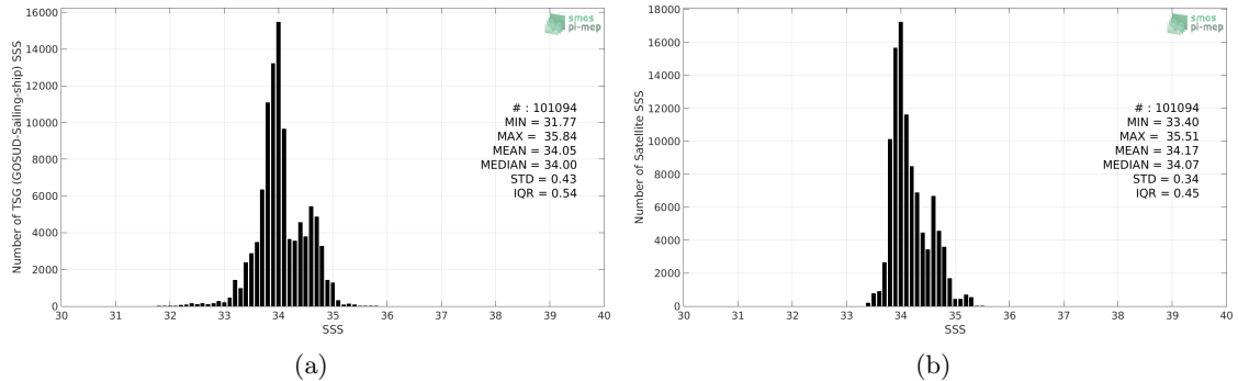
Figure 2: Histograms of SSS from TSG (GOSUD-Sailing-ship) (a) and SMAP SSS L4 OI v1 - Monthly (IPRC) (b) considering all match-up pairs per bins of 0.1 over the Roaring Forties and Furious Fifties Pi-MEP region and for the full satellite product period.
