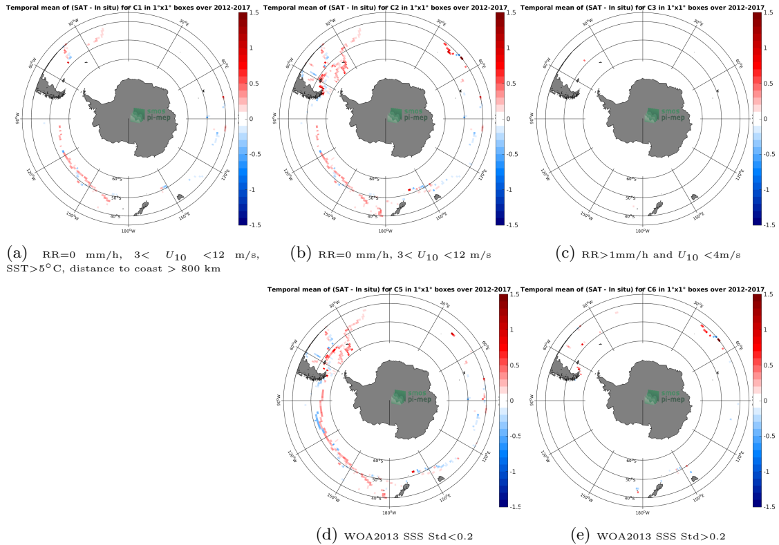
Figure 12: Temporal mean gridded over spatial boxes of size 1°x1° of \Delta SSS (SMAP SSS L4 OI v1 - Monthly (IPRC) - TSG (GOSUD-Sailing-ship)) for 5 different subdatasets corresponding to: RR=0 mm/h, 3 < U_{10} < 12 m/s, SST>5°C, distance to coast > 800 km (a), RR=0 mm/h, 3 < U_{10} < 12 m/s (b), RR>1mm/h and U_{10} < 4 m/s (c), WOA2013 SSS Std<0.2 (d), WOA2013 SSS Std>0.2 (e).
