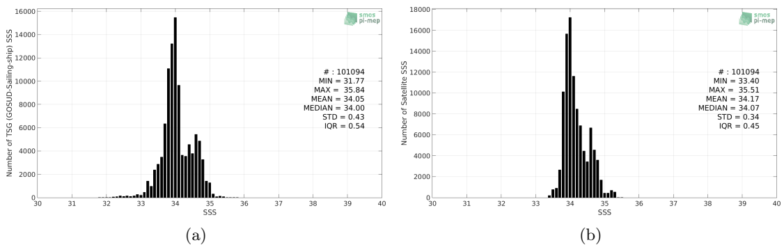
Figure 2: Histograms of SSS from TSG (GOSUD-Sailing-ship) (a) and SMAP SSS L4 OI v1 - Monthly (IPRC) (b) considering all match-up pairs per bins of 0.1 over the Roaring Forties and Furious Fifties Pi-MEP region and for the full satellite product period.
