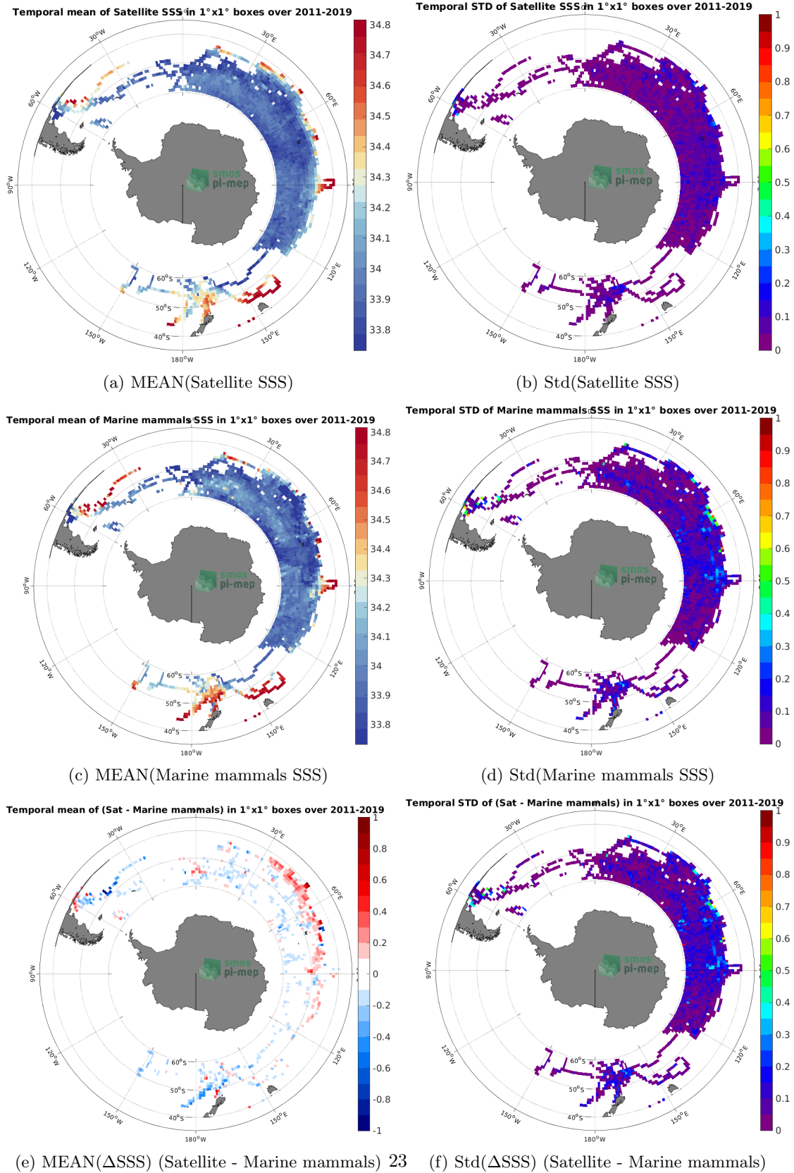
Figure 6: Temporal mean (left) and Std (right) of SSS from SMAP SSS L4 OI v1 - Monthly (IPRC) (top), Marine mammals (middle), and of \Delta SSS (Satellite - Marine mammals). Only match-up pairs are used to generate these maps.
