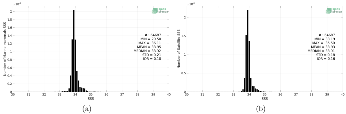
Figure 2: Histograms of SSS from Marine mammals (a) and SMAP SSS L4 OI v1 - Monthly (IPRC) (b) considering all match-up pairs per bins of 0.1 over the Roaring Forties and Furious Fifties Pi-MEP region and for the full satellite product period.
