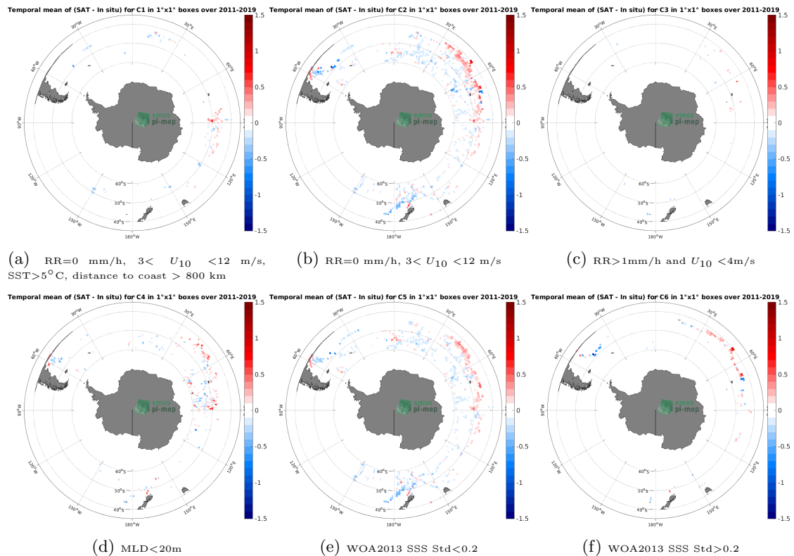
Figure 12: Temporal mean gridded over spatial boxes of size 1^{\circ}\times 1^{\circ} of \Delta\text{SSS} (SMAP SSS L4 OI v1 - Monthly (IPRC) - Marine mammals) for 6 different subdatasets corresponding to:RR=0 mm/h, 3 < U_{10} < 12 m/s, \text{SST} > 5^{\circ}\text{C} , distance to coast > 800 km (a), RR=0 mm/h, 3 < U_{10} < 12 m/s (b), RR > 1\text{mm/h} and U_{10} < 4\text{m/s} (c),MLD < 20\text{m} (d),WOA2013 SSS Std < 0.2 (e),WOA2013 SSS Std > 0.2 (f).
