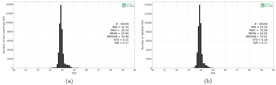
Figure 2: Histograms of SSS from Marine mammals (a) and SMAP SSS L4 OI v1 - Monthly (IPRC) (b) considering all match-up pairs per bins of 0.1 over the Roaring Forties and Furious Fifties Pi-MEP region and for the full satellite product period.
