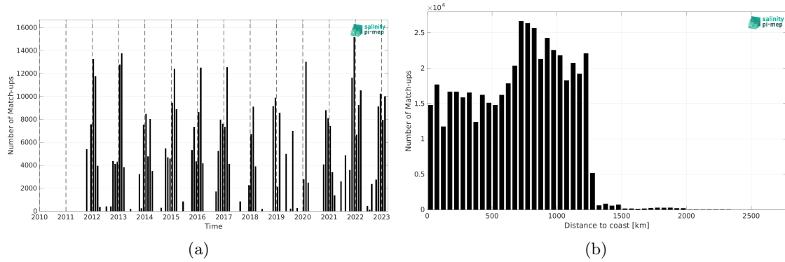
Figure 2: Number of match-ups between TSG (LEGOS-DM) and SMAP SSS L4 OI v3 - Monthly (ESR) SSS as a function of time (a) and as function of the distance to coast (b) over the Roaring Forties and Furious Fifties Pi-MEP region and for the full satellite product period.
