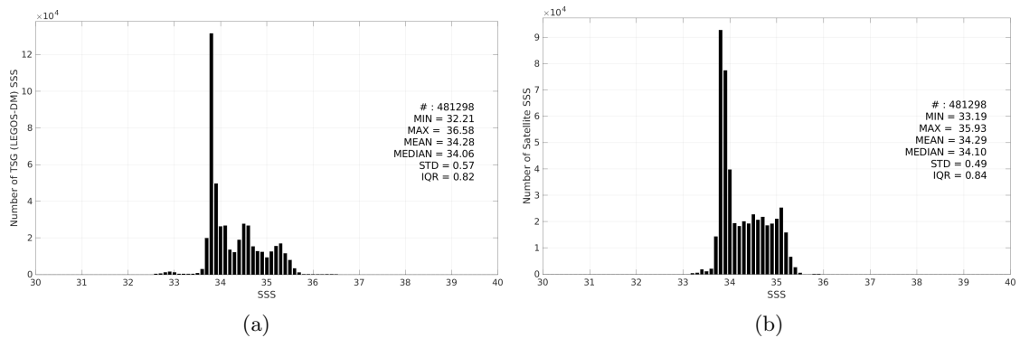
Figure 3: Histograms of SSS from TSG (LEGOS-DM) (a) and SMAP SSS L4 OI v3 - Monthly (ESR) (b) considering all match-up pairs per bins of 0.1 over the Roaring Forties and Furious Fifties Pi-MEP region and for the full satellite product period.
