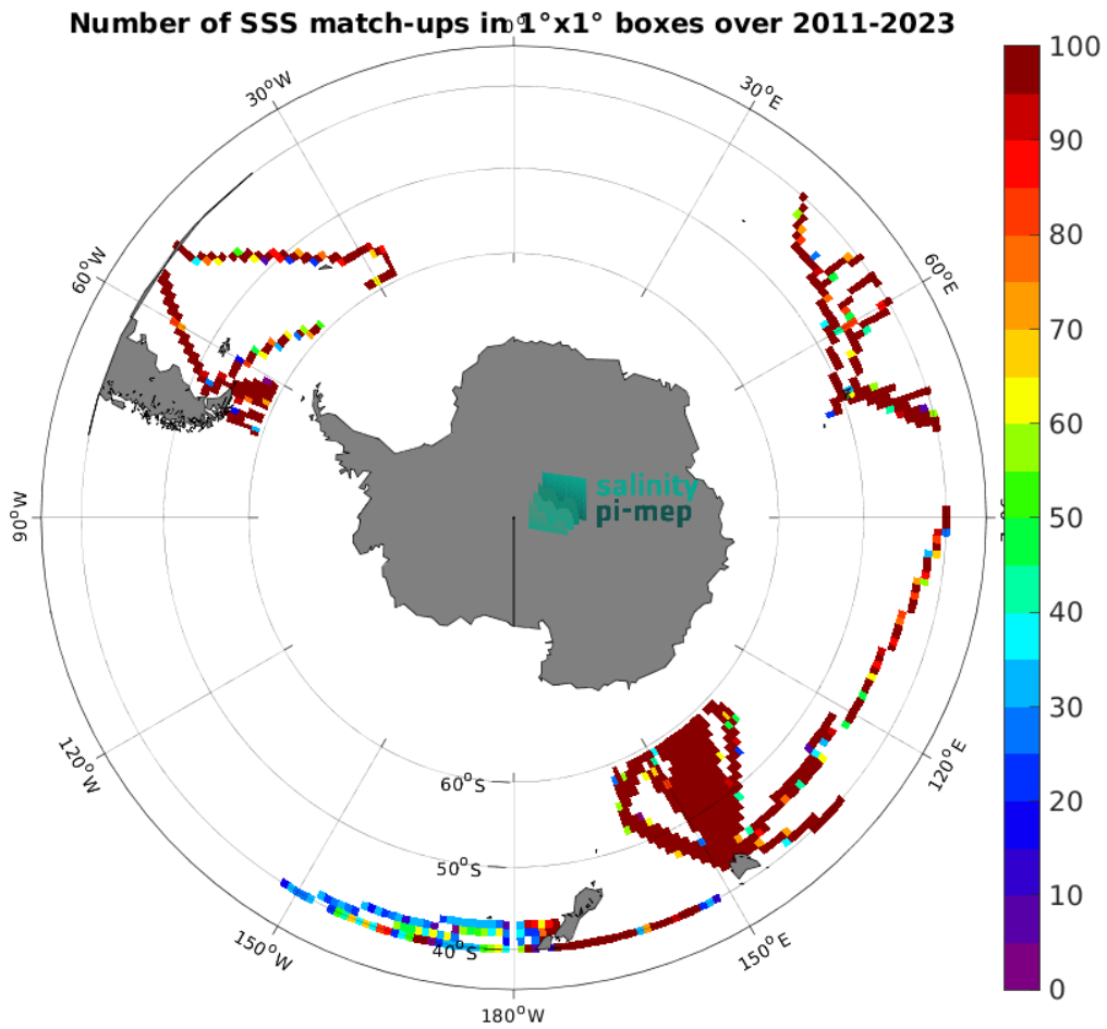
Figure 5: Number of SSS match-ups between TSG (LEGOS-DM) SSS and the SMAP SSS L4 OI v3 - Monthly (ESR) SSS product for the Roaring Forties and Furious Fifties Pi-MEP region over 1^\circ \times 1^\circ boxes and for the full satellite product period.
