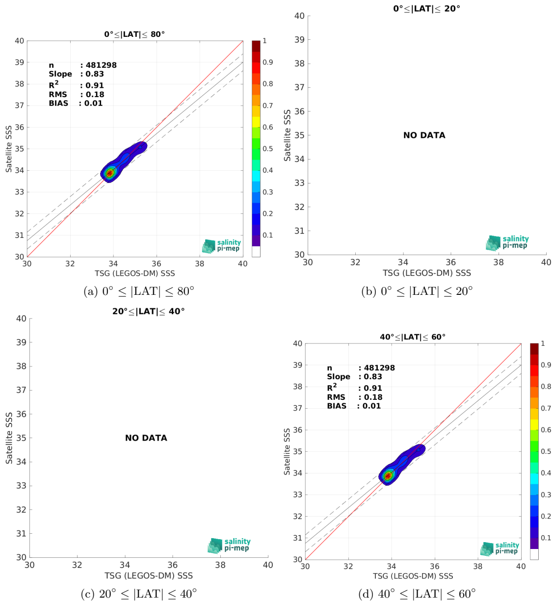
Figure 10: Contour maps of the concentration of SMAP SSS L4 OI v3 - Monthly (ESR) SSS (y-axis) versus TSG (LEGOS-DM) SSS (x-axis) at match-up pairs for different latitude bands. For each plot, the red line shows x=y . The black thin and dashed lines indicate a linear fit through the data cloud and the \pm 95\% confidence levels, respectively. The number match-up pairs n , the slope and R^2 coefficient of the linear fit, the root mean square (RMS) and the mean bias between satellite and in situ data are indicated for each latitude band in each plot.
