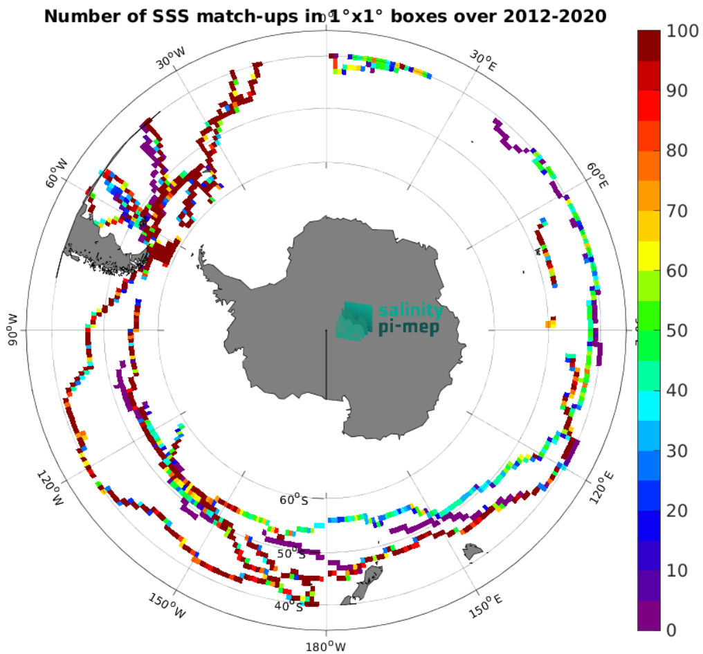
Figure 5: Number of SSS match-ups between TSG (GOSUD-Sailing-ship) SSS and the SMAP SSS L4 OI v3 - Monthly (ESR) SSS product for the Roaring Forties and Furious Fifties Pi-MEP region over 1^{\circ} \times 1^{\circ} boxes and for the full satellite product period.
