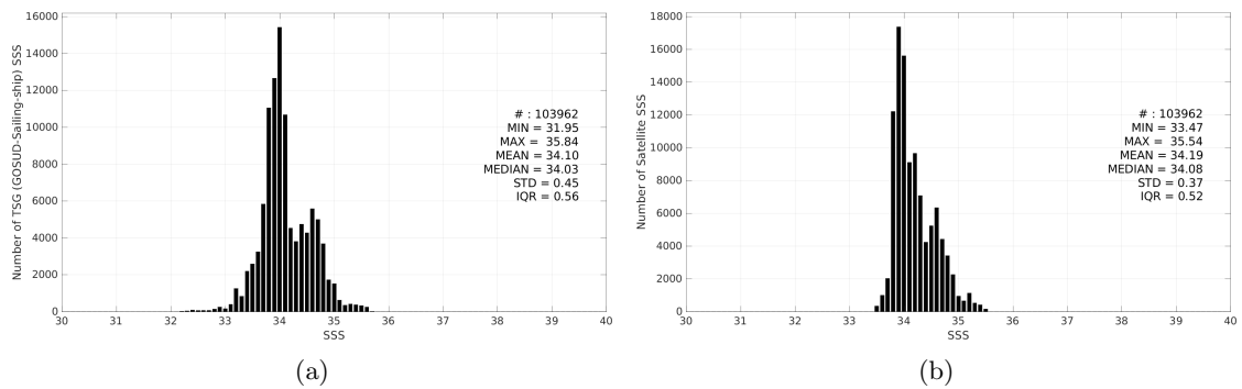
Figure 3: Histograms of SSS from TSG (GOSUD-Sailing-ship) (a) and SMAP SSS L4 OI v3 - Monthly (ESR) (b) considering all match-up pairs per bins of 0.1 over the Roaring Forties and Furious Fifties Pi-MEP region and for the full satellite product period.
