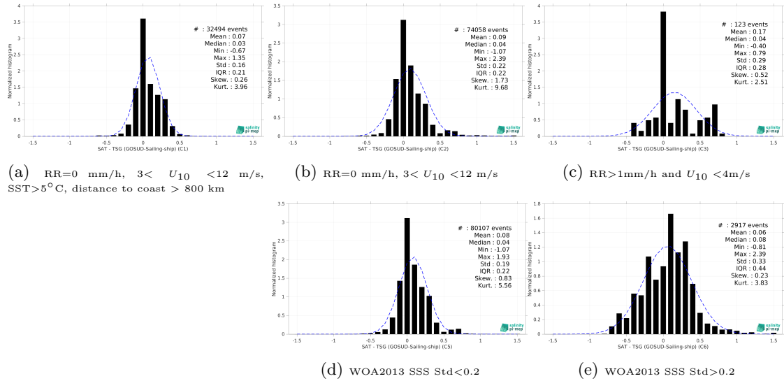
Figure 15: Normalized histogram of \Delta SSS (SMAP SSS L4 OI v3 - Monthly (ESR) - TSG (GOSUD-Sailing-ship)) for 5 different subdatasets corresponding to: RR=0 mm/h, 3 < U_{10} < 12 m/s, SST>5°C, distance to coast > 800 km (a), RR=0 mm/h, 3 < U_{10} < 12 m/s (b), RR>1mm/h and U_{10} < 4 m/s (c), WOA2013 SSS Std<0.2 (d), WOA2013 SSS Std>0.2 (e).
