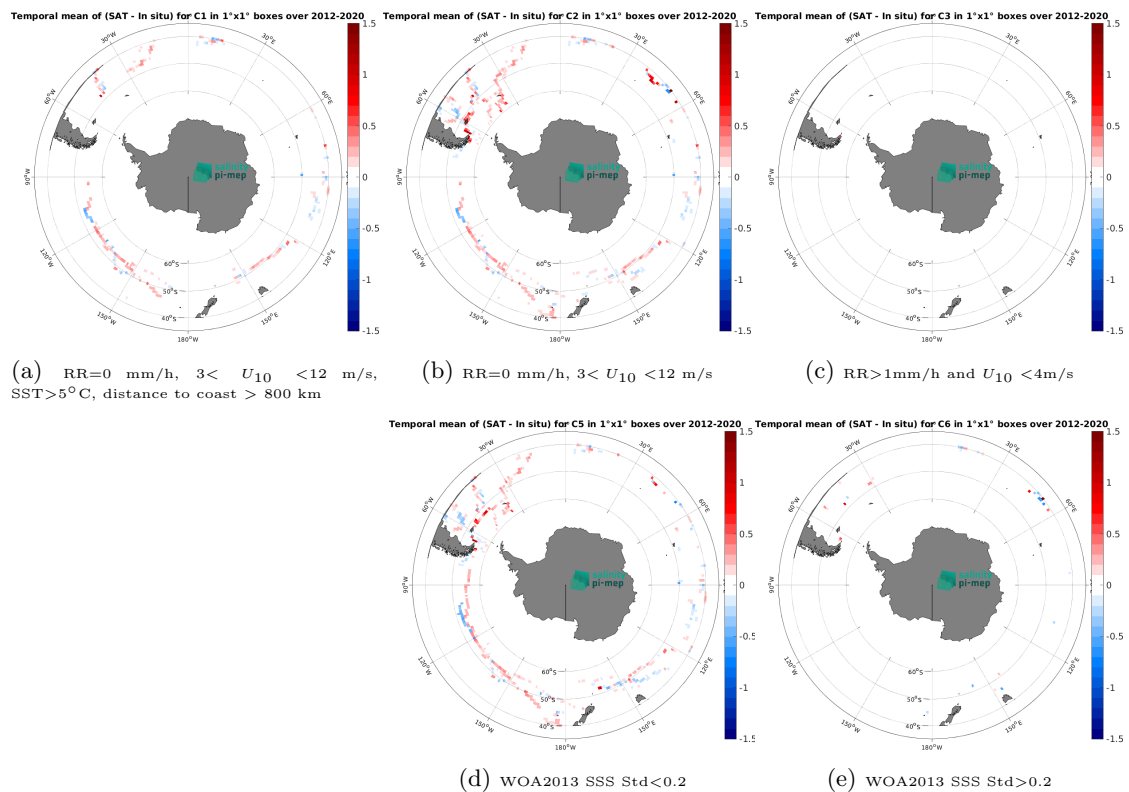
Figure 14: Temporal mean gridded over spatial boxes of size 1^\circ \times 1^\circ of \Delta\text{SSS} (SMAP SSS L4 OI v3 - Monthly (ESR) - TSG (GOSUD-Sailing-ship)) for 5 different subdatasets corresponding to: RR=0 mm/h, 3 < U_{10} < 12 m/s, SST > 5°C, distance to coast > 800 km (a), RR=0 mm/h, 3 < U_{10} < 12 m/s (b), RR > 1mm/h and U_{10} < 4 m/s (c), WOA2013 SSS Std < 0.2 (d), WOA2013 SSS Std > 0.2 (e).
