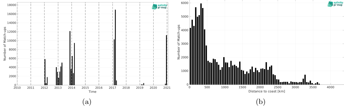
Figure 2: Number of match-ups between TSG (GOSUD-Sailing-ship) and SMAP SSS L4 OI v3 - Monthly (ESR) SSS as a function of time (a) and as function of the distance to coast (b) over the Roaring Forties and Furious Fifties Pi-MEP region and for the full satellite product period.
