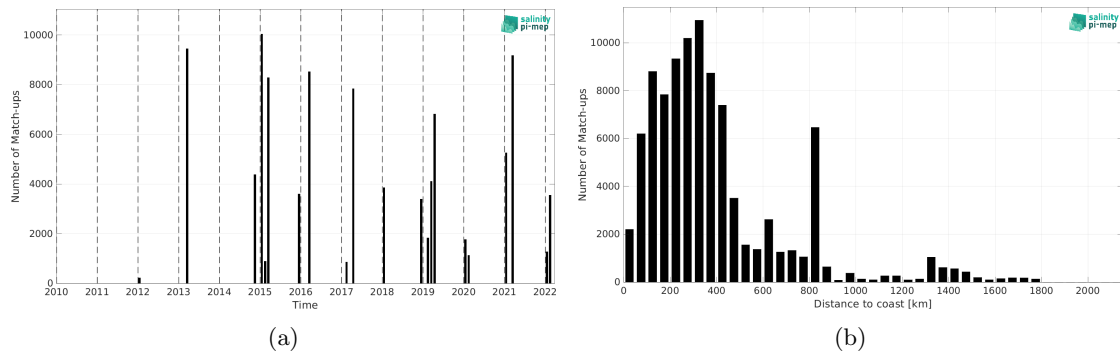
Figure 2: Number of match-ups between TSG (CSIC-UTM) and SMAP SSS L4 OI v3 - Monthly (ESR) SSS as a function of time (a) and as function of the distance to coast (b) over the Roaring Forties and Furious Fifties Pi-MEP region and for the full satellite product period.
