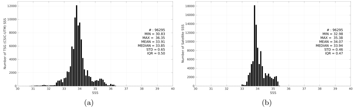
Figure 3: Histograms of SSS from TSG (CSIC-UTM) (a) and SMAP SSS L4 OI v3 - Monthly (ESR) (b) considering all match-up pairs per bins of 0.1 over the Roaring Forties and Furious Fifties Pi-MEP region and for the full satellite product period.
