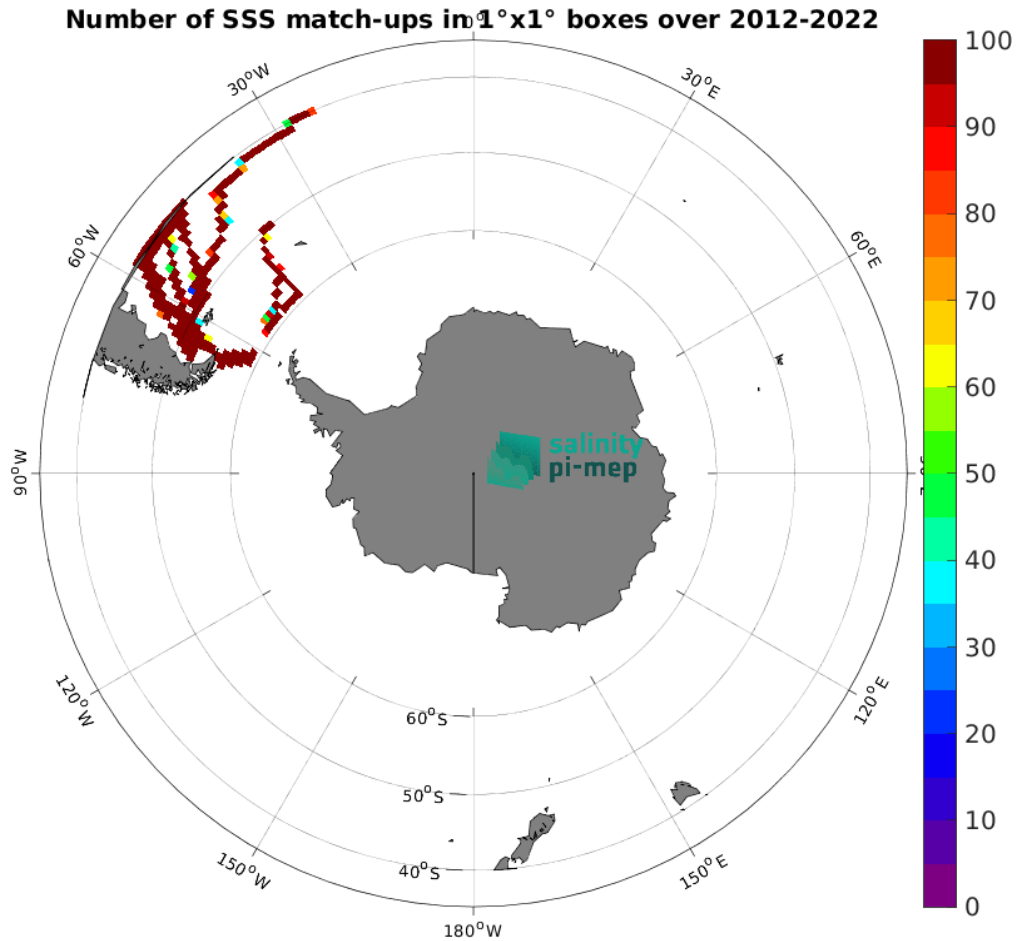
Figure 5: Number of SSS match-ups between TSG (CSIC-UTM) SSS and the SMAP SSS L4 OI v3 - Monthly (ESR) SSS product for the Roaring Forties and Furious Fifties Pi-MEP region over 1^\circ \times 1^\circ boxes and for the full satellite product period.
