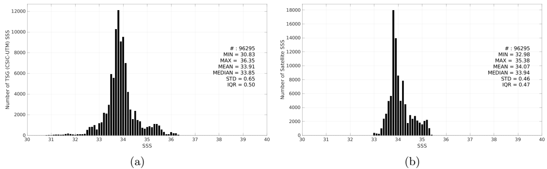
Figure 3: Histograms of SSS from TSG (CSIC-UTM) (a) and SMAP SSS L4 OI v3 - Monthly (ESR) (b) considering all match-up pairs per bins of 0.1 over the Roaring Forties and Furious Fifties Pi-MEP region and for the full satellite product period.
