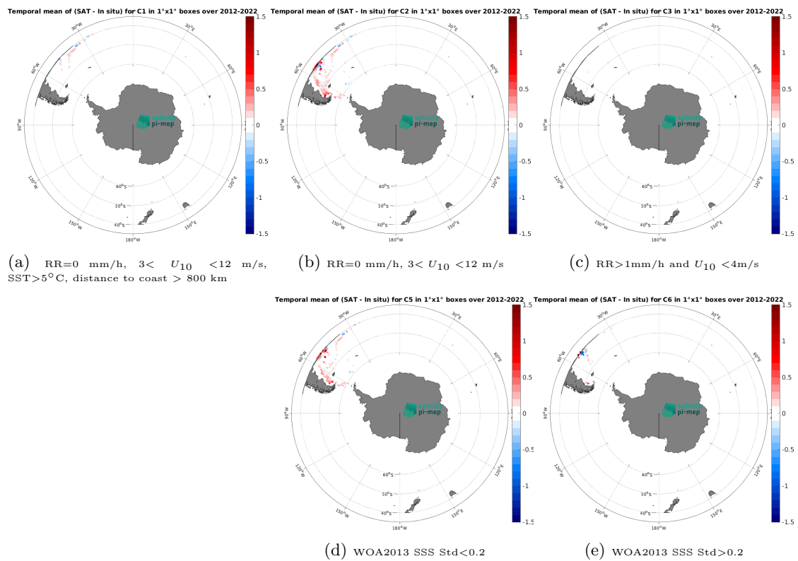
Figure 14: Temporal mean gridded over spatial boxes of size 1^\circ \times 1^\circ of \Delta SSS (SMAP SSS L4 OI v3 - Monthly (ESR) - TSG (CSIC-UTM)) for 5 different subdatasets corresponding to:RR=0 mm/h, 3 < U_{10} < 12 m/s, SST>5°C, distance to coast > 800 km (a), RR=0 mm/h, 3 < U_{10} < 12 m/s (b), RR>1mm/h and U_{10} < 4 m/s (c), WOA2013 SSS Std<0.2 (d), WOA2013 SSS Std>0.2 (e).
