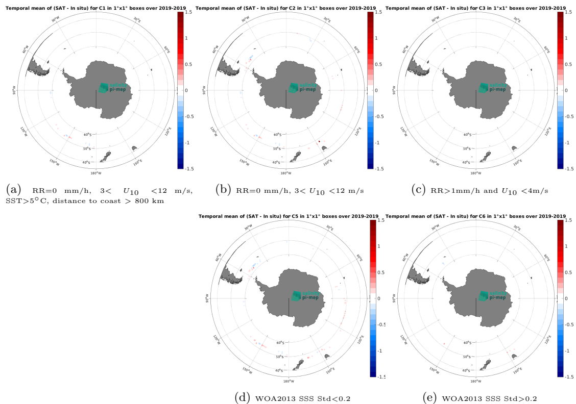
Figure 14: Temporal mean gridded over spatial boxes of size 1^\circ \times 1^\circ of \Delta\text{SSS} (SMAP SSS L4 OI v3 - Monthly (ESR) - Saildrone) for 5 different subdatasets corresponding to:RR=0 mm/h, 3 < U_{10} < 12 m/s, SST>5°C, distance to coast > 800 km (a), RR=0 mm/h, 3 < U_{10} < 12 m/s (b), RR>1mm/h and U_{10} < 4 m/s (c), WOA2013 SSS Std<0.2 (d), WOA2013 SSS Std>0.2 (e).
