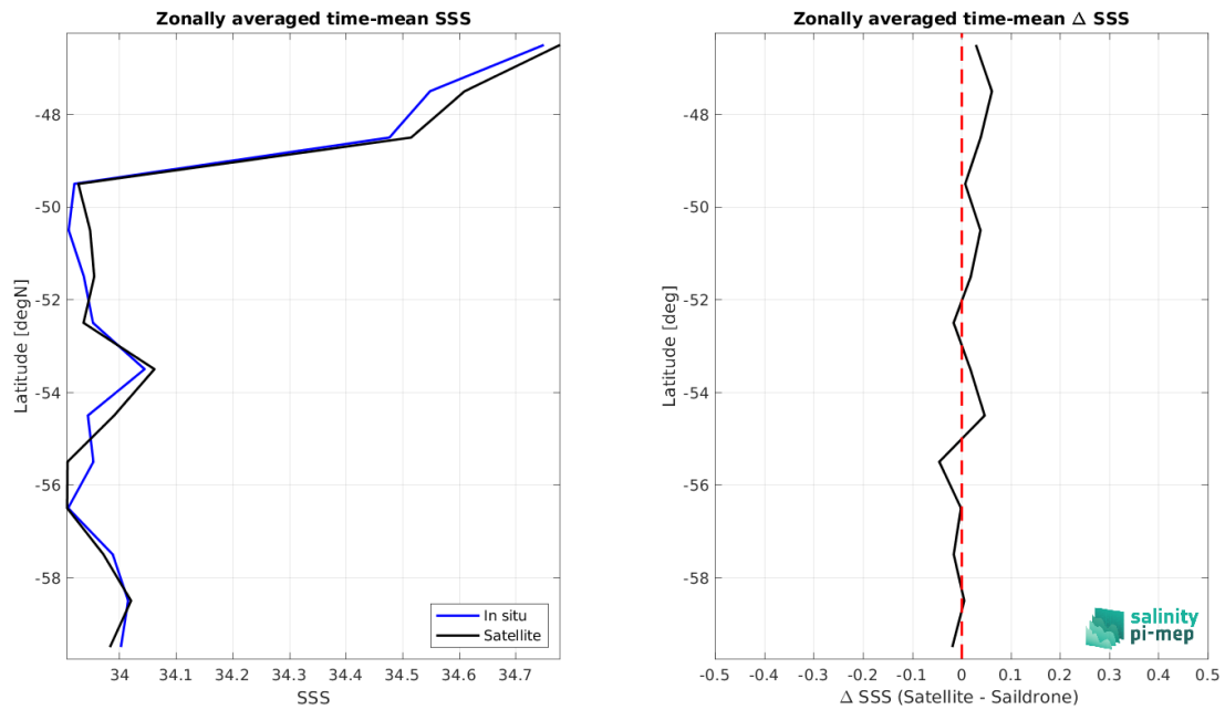
Figure 9: Left panel: Zonal mean SSS from SMAP SSS L4 OI v3 - Monthly (ESR) satellite product (black) and from Sairdronne (blue). Right panel: Zonal mean of \Delta SSS (Satellite - Sairdronne) for all the collected Pi-MEP match-up pairs estimated over the full satellite product period.
