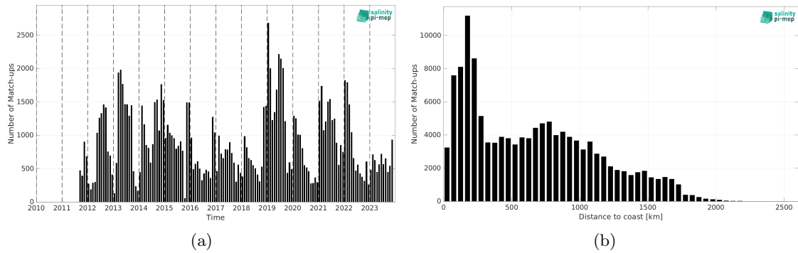
Figure 2: Number of match-ups between Marine mammals and SMAP SSS L4 OI v3 - Monthly (ESR) SSS as a function of time (a) and as function of the distance to coast (b) over the Roaring Forties and Furious Fifties Pi-MEP region and for the full satellite product period.
