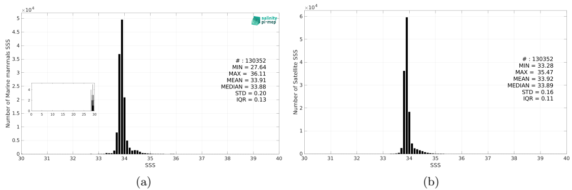
Figure 3: Histograms of SSS from Marine mammals (a) and SMAP SSS L4 OI v3 - Monthly (ESR) (b) considering all match-up pairs per bins of 0.1 over the Roaring Forties and Furious Fifties Pi-MEP region and for the full satellite product period.
