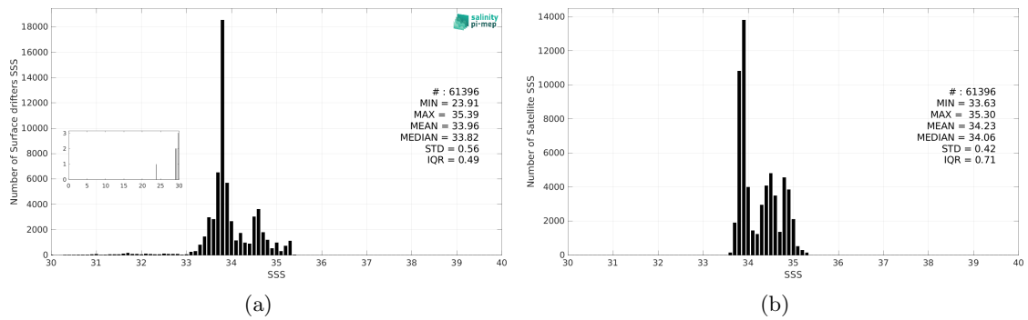
Figure 3: Histograms of SSS from Surface drifters (a) and SMAP SSS L4 OI v3 - Monthly (ESR) (b) considering all match-up pairs per bins of 0.1 over the Roaring Forties and Furious Fifties Pi-MEP region and for the full satellite product period.
