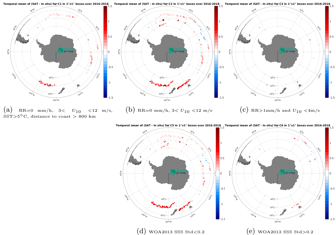
Figure 13: Temporal mean gridded over spatial boxes of size 1^\circ \times 1^\circ of \Delta SSS (SMAP SSS L4 OI v3 - Monthly (ESR) - Surface drifters) for 5 different subdatasets corresponding to:RR=0 mm/h, 3 < U_{10} < 12 m/s, SST >5^\circ C, distance to coast > 800 km (a), RR=0 mm/h, 3 < U_{10} < 12 m/s (b), RR >1 mm/h and U_{10} < 4 m/s (c), WOA2013 SSS Std <0.2 (d), WOA2013 SSS Std >0.2 (e).
