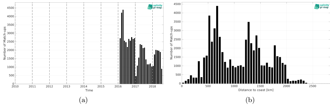
Figure 2: Number of match-ups between Surface drifters and SMAP SSS L4 OI v3 - Monthly (ESR) SSS as a function of time (a) and as function of the distance to coast (b) over the Roaring Forties and Furious Fifties Pi-MEP region and for the full satellite product period.
