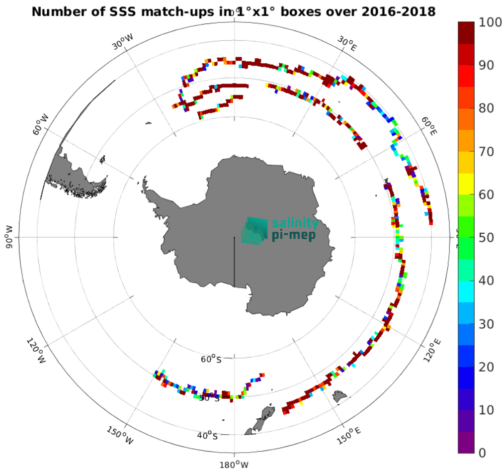
Figure 4: Number of SSS match-ups between Surface drifters SSS and the SMAP SSS L4 OI v3 - Monthly (ESR) SSS product for the Roaring Forties and Furious Fifties Pi-MEP region over 1^\circ \times 1^\circ boxes and for the full satellite product period.
