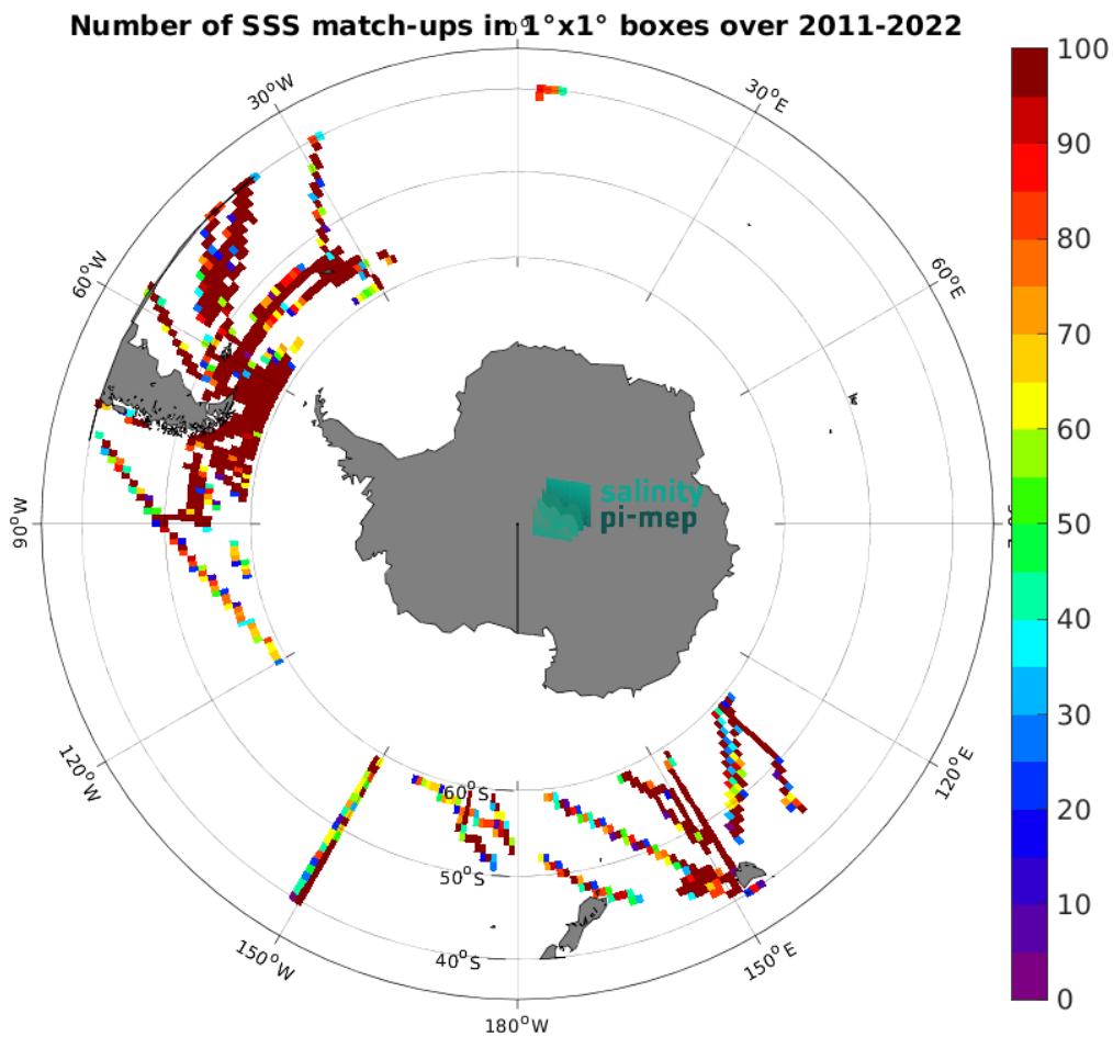
Figure 5: Number of SSS match-ups between TSG (SAMOS) SSS and the SMAP SSS L4 OI v3 - Daily (ESR) SSS product for the Roaring Forties and Furious Fifties Pi-MEP region over 1^\circ \times 1^\circ boxes and for the full satellite product period.
