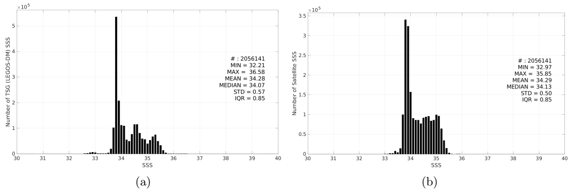
Figure 3: Histograms of SSS from TSG (LEGOS-DM) (a) and SMAP SSS L4 OI v3 - Daily (ESR) (b) considering all match-up pairs per bins of 0.1 over the Roaring Forties and Furious Fifties Pi-MEP region and for the full satellite product period.
