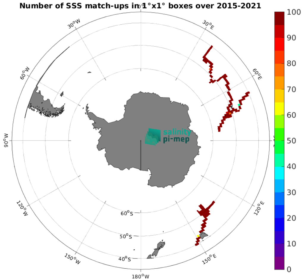
Figure 5: Number of SSS match-ups between TSG (GOSUD-Research-vessel) SSS and the SMAP SSS L4 OI v3 - Daily (ESR) SSS product for the Roaring Forties and Furious Fifties Pi-MEP region over 1^\circ \times 1^\circ boxes and for the full satellite product period.
