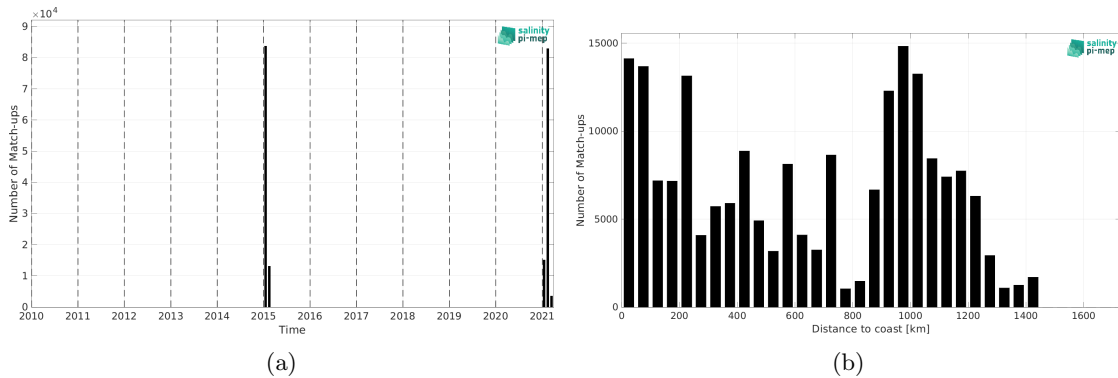
Figure 2: Number of match-ups between TSG (GOSUD-Research-vessel) and SMAP SSS L4 OI v3 - Daily (ESR) SSS as a function of time (a) and as function of the distance to coast (b) over the Roaring Forties and Furious Fifties Pi-MEP region and for the full satellite product period.
