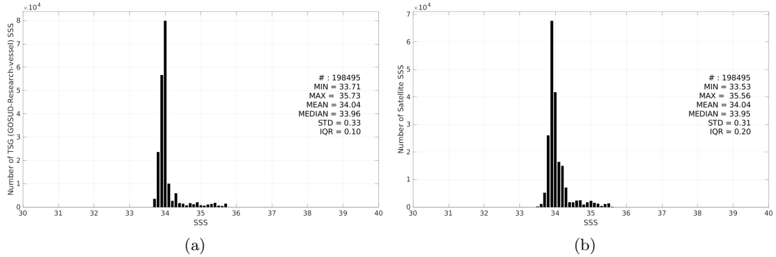
Figure 3: Histograms of SSS from TSG (GOSUD-Research-vessel) (a) and SMAP SSS L4 OI v3 - Daily (ESR) (b) considering all match-up pairs per bins of 0.1 over the Roaring Forties and Furious Fifties Pi-MEP region and for the full satellite product period.
