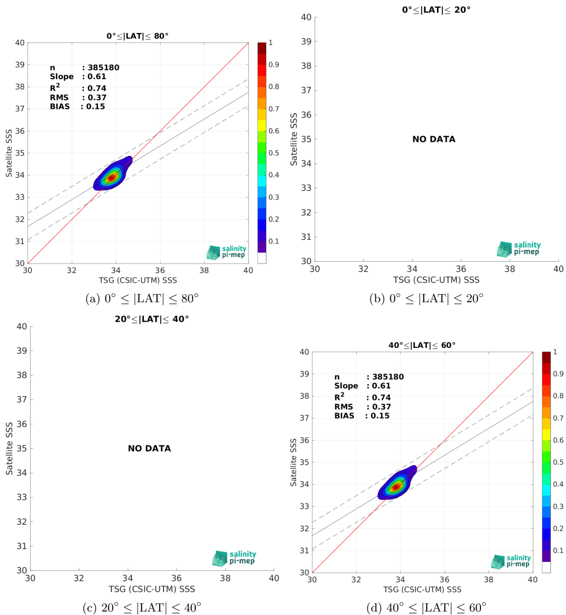
Figure 10: Contour maps of the concentration of SMAP SSS L4 OI v3 - Daily (ESR) SSS (y-axis) versus TSG (CSIC-UTM) SSS (x-axis) at match-up pairs for different latitude bands. For each plot, the red line shows x=y . The black thin and dashed lines indicate a linear fit through the data cloud and the \pm 95\% confidence levels, respectively. The number match-up pairs n , the slope and R^2 coefficient of the linear fit, the root mean square (RMS) and the mean bias between satellite and in situ data are indicated for each latitude band in each plot.
