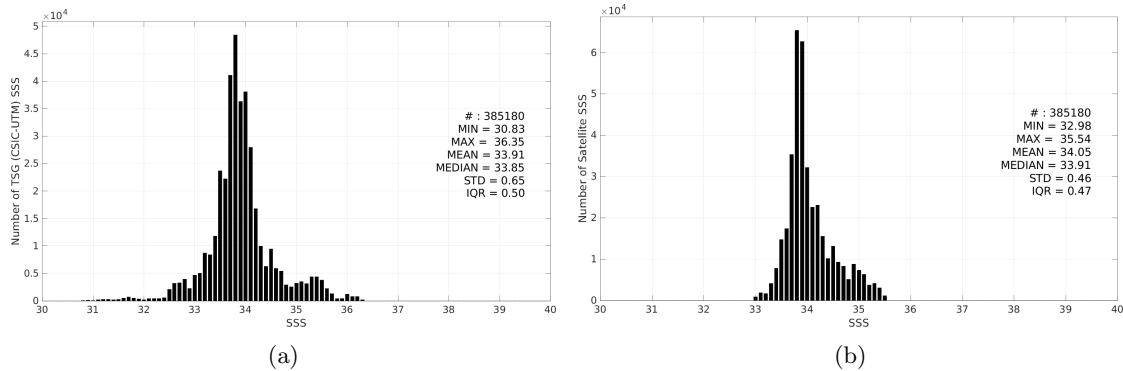
Figure 3: Histograms of SSS from TSG (CSIC-UTM) (a) and SMAP SSS L4 OI v3 - Daily (ESR) (b) considering all match-up pairs per bins of 0.1 over the Roaring Forties and Furious Fifties Pi-MEP region and for the full satellite product period.
