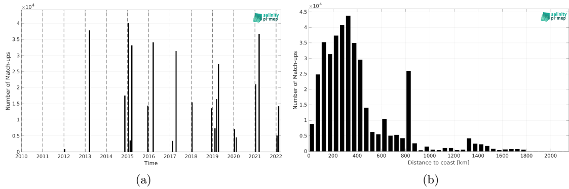
Figure 2: Number of match-ups between TSG (CSIC-UTM) and SMAP SSS L4 OI v3 - Daily (ESR) SSS as a function of time (a) and as function of the distance to coast (b) over the Roaring Forties and Furious Fifties Pi-MEP region and for the full satellite product period.
