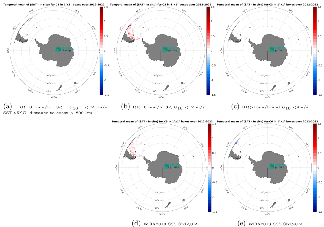
Figure 14: Temporal mean gridded over spatial boxes of size 1^\circ \times 1^\circ of \Delta SSS (SMAP SSS L4 OI v3 - Daily (ESR) - TSG (CSIC-UTM)) for 5 different subdatasets corresponding to:RR=0 mm/h, 3 < U_{10} < 12 m/s, SST>5°C, distance to coast > 800 km (a), RR=0 mm/h, 3 < U_{10} < 12 m/s (b), RR>1mm/h and U_{10} < 4 m/s (c), WOA2013 SSS Std<0.2 (d), WOA2013 SSS Std>0.2 (e).
