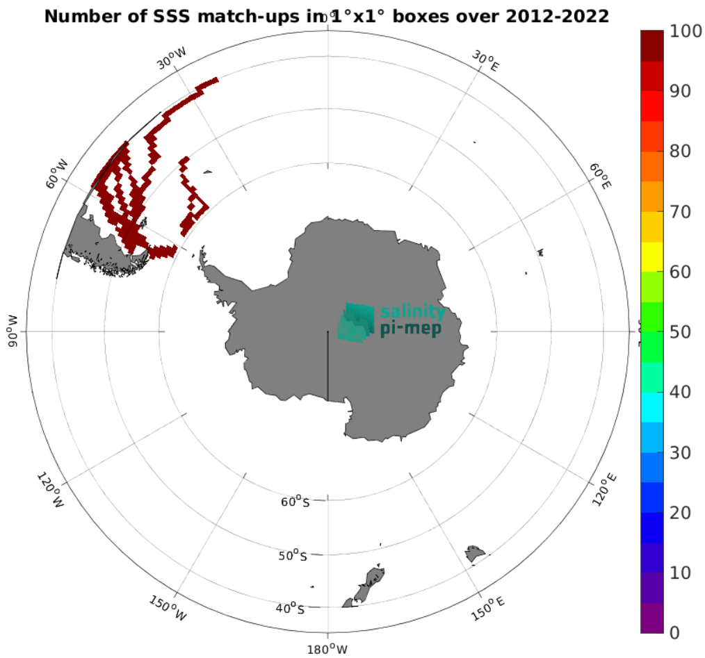
Figure 5: Number of SSS match-ups between TSG (CSIC-UTM) SSS and the SMAP SSS L4 OI v3 - Daily (ESR) SSS product for the Roaring Forties and Furious Fifties Pi-MEP region over 1^\circ \times 1^\circ boxes and for the full satellite product period.
