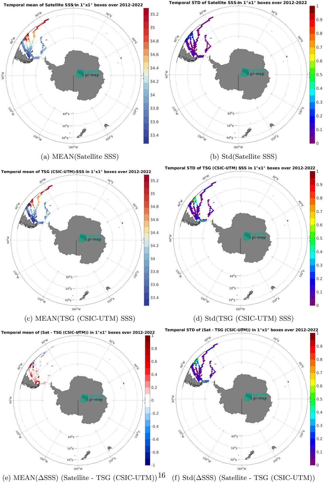
Figure 7: Temporal mean (left) and Std (right) of SSS from SMAP SSS L4 OI v3 - Daily (ESR) (top), TSG (CSIC-UTM) (middle), and of \Delta SSS (Satellite - TSG (CSIC-UTM)). Only match-up pairs are used to generate these maps.
