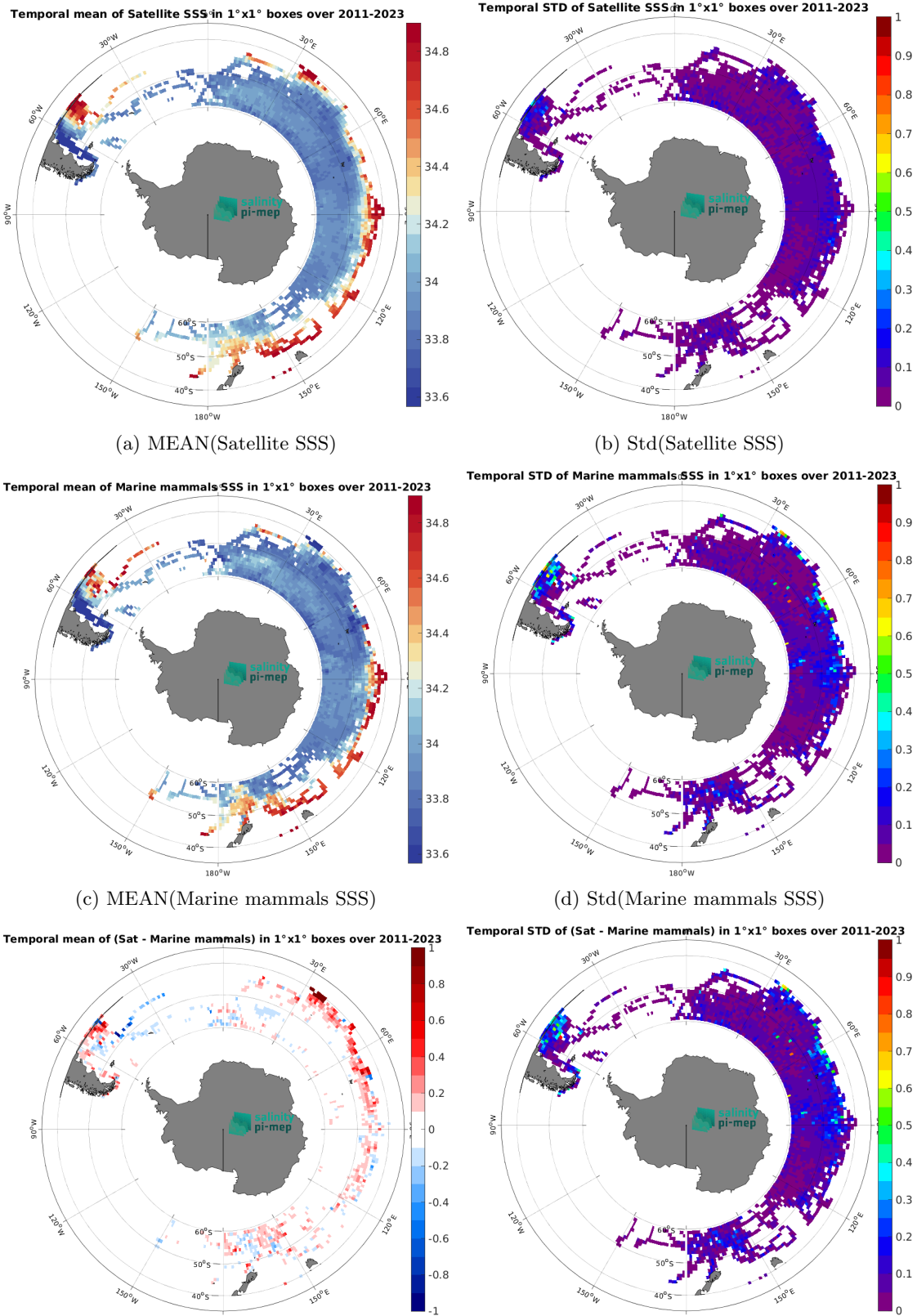
Figure 7: Temporal mean (left) and Std (right) of SSS from SMAP SSS L4 OI v3 - Daily (ESR) (top), Marine mammals (middle), and of \Delta SSS (Satellite - Marine mammals). Only match-up pairs are used to generate these maps.
