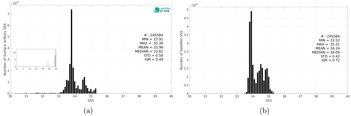
Figure 3: Histograms of SSS from Surface drifters (a) and SMAP SSS L4 OI v3 - Daily (ESR) (b) considering all match-up pairs per bins of 0.1 over the Roaring Forties and Furious Fifties Pi-MEP region and for the full satellite product period.
