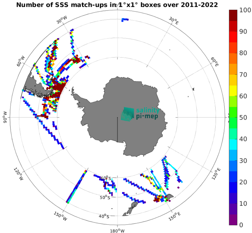
Figure 4: Number of SSS match-ups between TSG (SAMOS) SSS and the SMAP SSS L4 OI v2 - 7 Days (ESR) SSS product for the Roaring Forties and Furious Fifties Pi-MEP region over 1^\circ \times 1^\circ boxes and for the full satellite product period.
