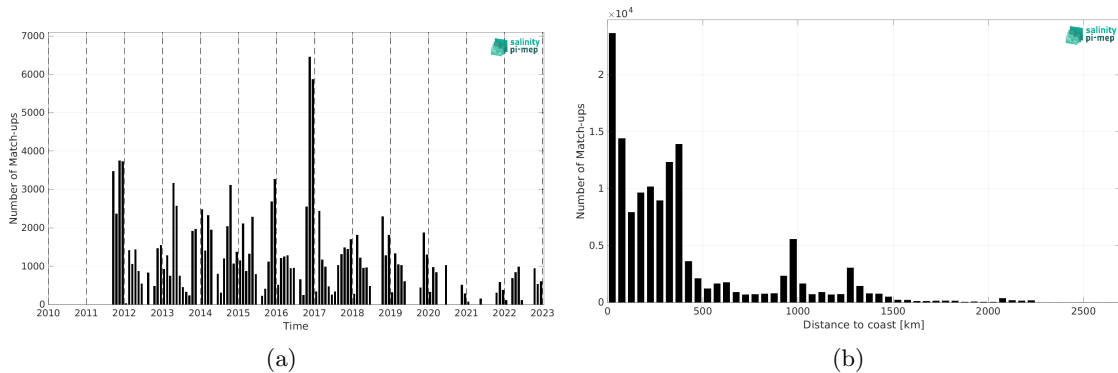
Figure 1: Number of match-ups between TSG (SAMOS) and SMAP SSS L4 OI v2 - 7 Days (ESR) SSS as a function of time (a) and as function of the distance to coast (b) over the Roaring Forties and Furious Fifties Pi-MEP region and for the full satellite product period.
