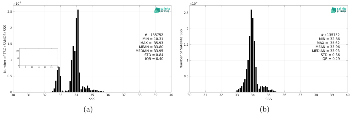
Figure 2: Histograms of SSS from TSG (SAMOS) (a) and SMAP SSS L4 OI v2 - 7 Days (ESR) (b) considering all match-up pairs per bins of 0.1 over the Roaring Forties and Furious Fifties Pi-MEP region and for the full satellite product period.
