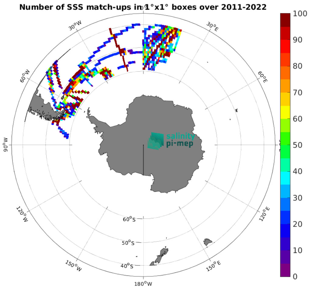
Figure 4: Number of SSS match-ups between TSG (Polarstern) SSS and the SMAP SSS L4 OI v2 - 7 Days (ESR) SSS product for the Roaring Forties and Furious Fifties Pi-MEP region over 1^\circ \times 1^\circ boxes and for the full satellite product period.
