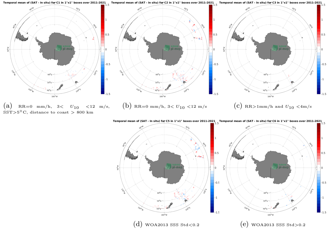
Figure 12: Temporal mean gridded over spatial boxes of size 1^{\circ}\times 1^{\circ} of \Delta\text{SSS} (SMAP SSS L4 OI v2 - 7 Days (ESR) - TSG (LEGOS-DM)) for 5 different subdatasets corresponding to:RR=0 mm/h, 3 < U_{10} < 12 m/s, SST >5^{\circ}\text{C} , distance to coast > 800 km (a), RR=0 mm/h, 3 < U_{10} < 12 m/s (b), RR >1 mm/h and U_{10} < 4 m/s (c), WOA2013 SSS Std <0.2 (d), WOA2013 SSS Std >0.2 (e).
