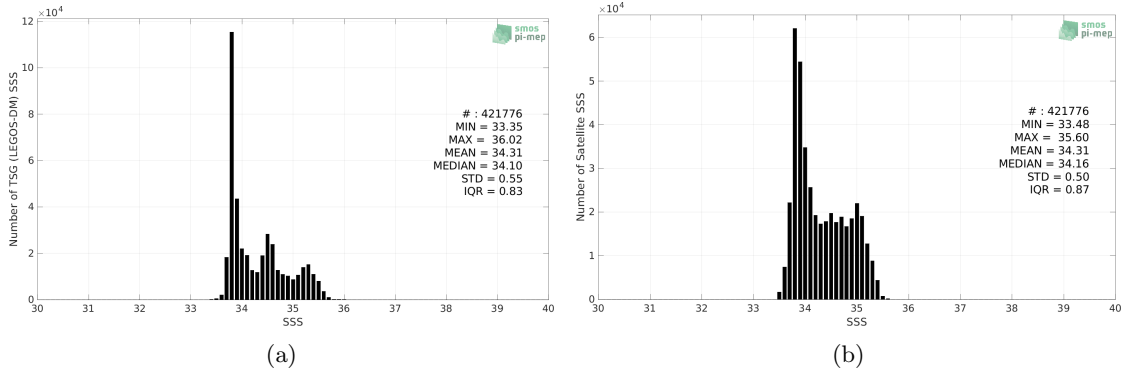
Figure 2: Histograms of SSS from TSG (LEGOS-DM) (a) and SMAP SSS L4 OI v2 - 7 Days (ESR) (b) considering all match-up pairs per bins of 0.1 over the Roaring Forties and Furious Fifties Pi-MEP region and for the full satellite product period.
