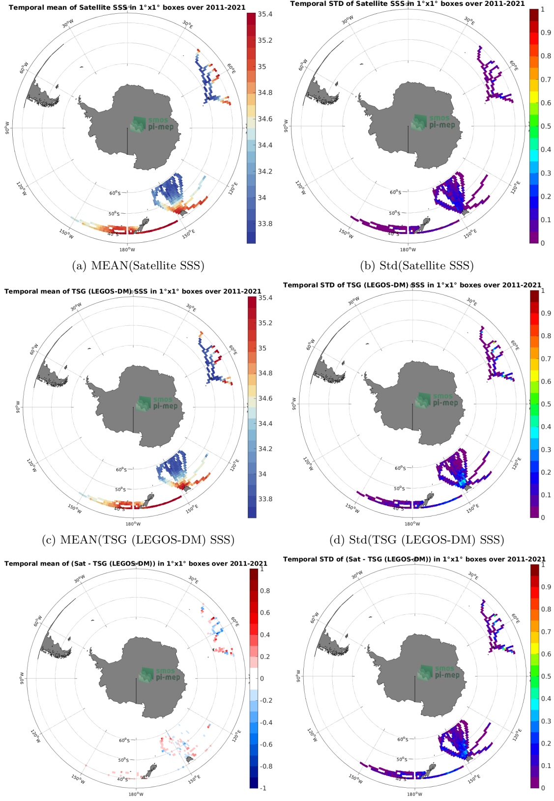
Figure 6: Temporal mean (left) and Std (right) of SSS from SMAP SSS L4 OI v2 - 7 Days (ESR) (top), TSG (LEGOS-DM) (middle), and of \Delta SSS (Satellite - TSG (LEGOS-DM)). Only match-up pairs are used to generate these maps.
