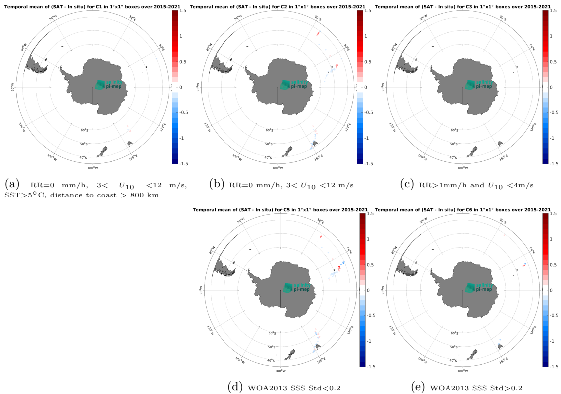
Figure 12: Temporal mean gridded over spatial boxes of size 1°×1° of \Delta SSS (SMAP SSS L4 OI v2 - 7 Days (ESR) - TSG (GOSUD-Research-vessel)) for 5 different subdatasets corresponding to:RR=0 mm/h, 3 < U_{10} < 12 m/s, SST>5°C, distance to coast > 800 km (a), RR=0 mm/h, 3 < U_{10} < 12 m/s (b), RR>1mm/h and U_{10} < 4 m/s (c), WOA2013 SSS Std<0.2 (d), WOA2013 SSS Std>0.2 (e).
