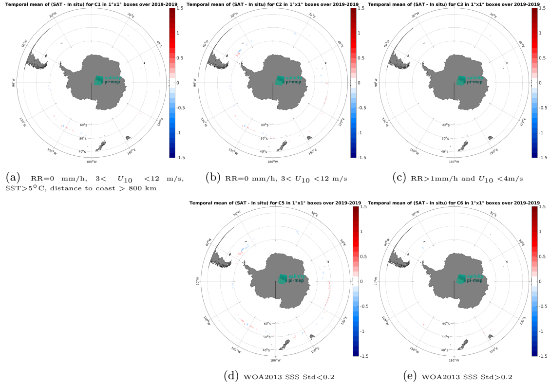
Figure 12: Temporal mean gridded over spatial boxes of size 1^{\circ}\times 1^{\circ} of \Delta\text{SSS} (SMAP SSS L4 OI v2 - 7 Days (ESR) - Saildrone) for 5 different subdatasets corresponding to: \text{RR}=0 mm/h, 3 < U_{10} < 12 m/s, \text{SST}>5^{\circ}\text{C} , distance to coast > 800 km (a), \text{RR}=0 mm/h, 3 < U_{10} < 12 m/s (b), \text{RR}>1 mm/h and U_{10} < 4 m/s (c), WOA2013 SSS Std <0.2 (d), WOA2013 SSS Std >0.2 (e).
