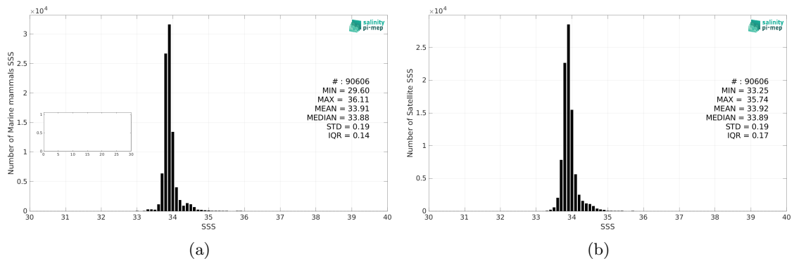
Figure 2: Histograms of SSS from Marine mammals (a) and SMAP SSS L4 OI v2 - 7 Days (ESR) (b) considering all match-up pairs per bins of 0.1 over the Roaring Forties and Furious Fifties Pi-MEP region and for the full satellite product period.
