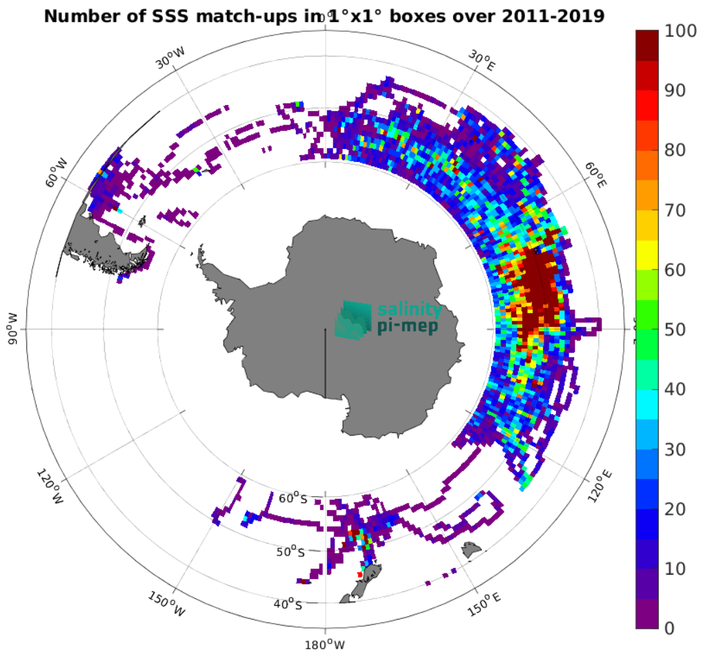
Figure 4: Number of SSS match-ups between Marine mammals SSS and the SMAP SSS L4 OI v2 - 7 Days (ESR) SSS product for the Roaring Forties and Furious Fifties Pi-MEP region over 1^\circ \times 1^\circ boxes and for the full satellite product period.
