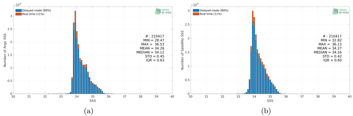
Figure 2: Histograms of SSS from Argo (a) and SMAP SSS L4 OI v2 - 7 Days (ESR) (b) considering all match-up pairs per bins of 0.1 over the Roaring Forties and Furious Fifties Pi-MEP region and for the full satellite product period.
