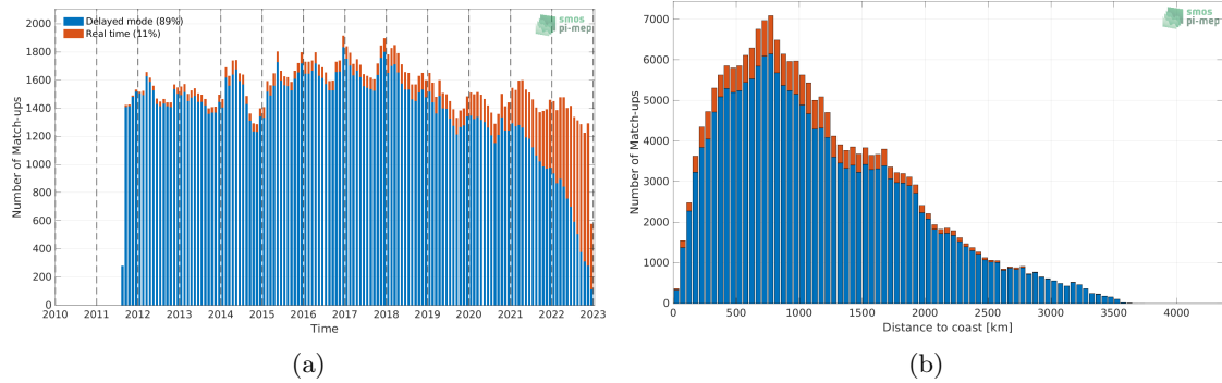
Figure 1: Number of match-ups between Argo and SMAP SSS L4 OI v2 - 7 Days (ESR) SSS as a function of time (a) and as function of the distance to coast (b) over the Roaring Forties and Furious Fifties Pi-MEP region and for the full satellite product period.
