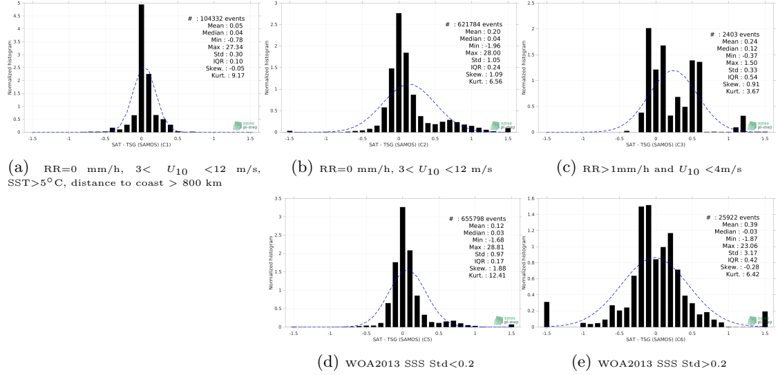
Figure 13: Normalized histogram of \Delta SSS (SMAP SSS L4 OI v2 - Monthly (IPRC) - TSG (SAMOS)) for 5 different subdatasets corresponding to: RR=0 mm/h, 3 < U_{10} < 12 m/s, SST>5°C, distance to coast > 800 km (a), RR=0 mm/h, 3 < U_{10} < 12 m/s (b), RR>1mm/h and U_{10} < 4 m/s (c), WOA2013 SSS Std<0.2 (d), WOA2013 SSS Std>0.2 (e).
