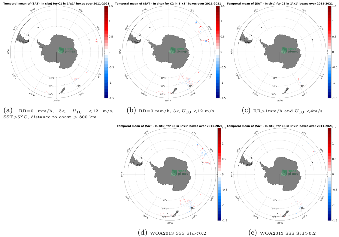
Figure 12: Temporal mean gridded over spatial boxes of size 1^{\circ}\times 1^{\circ} of \Delta\text{SSS} (SMAP SSS L4 OI v2 - Monthly (IPRC) - TSG (LEGOS-DM)) for 5 different subdatasets corresponding to:RR=0 mm/h, 3 < U_{10} < 12 m/s, SST >5^{\circ}\text{C} , distance to coast > 800 km (a), RR=0 mm/h, 3 < U_{10} < 12 m/s (b), RR >1 mm/h and U_{10} < 4 m/s (c), WOA2013 SSS Std <0.2 (d), WOA2013 SSS Std >0.2 (e).
