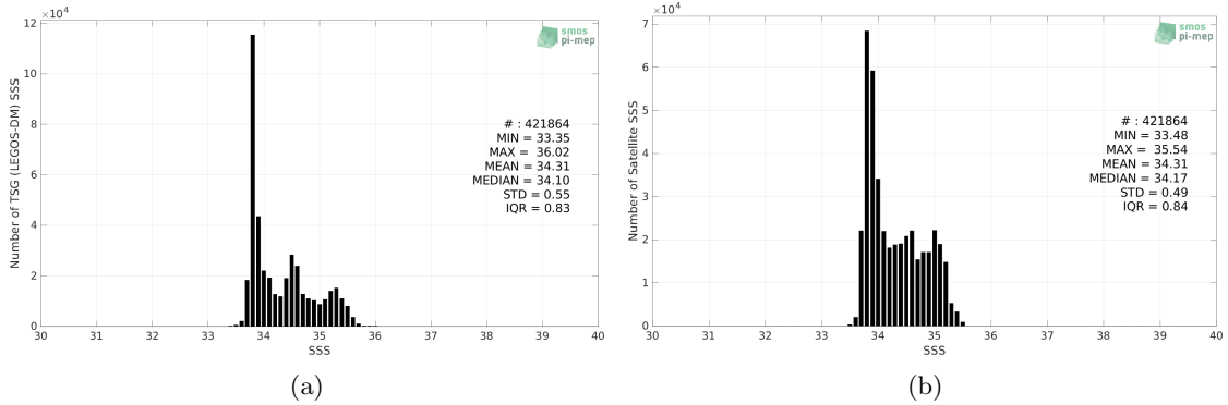
Figure 2: Histograms of SSS from TSG (LEGOS-DM) (a) and SMAP SSS L4 OI v2 - Monthly (IPRC) (b) considering all match-up pairs per bins of 0.1 over the Roaring Forties and Furious Fifties Pi-MEP region and for the full satellite product period.
