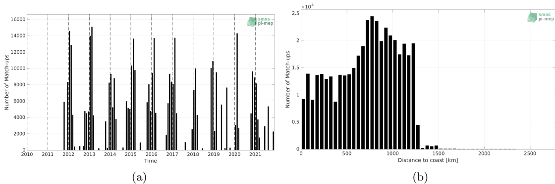
Figure 1: Number of match-ups between TSG (LEGOS-DM) and SMAP SSS L4 OI v2 - Monthly (IPRC) SSS as a function of time (a) and as function of the distance to coast (b) over the Roaring Forties and Furious Fifties Pi-MEP region and for the full satellite product period.
