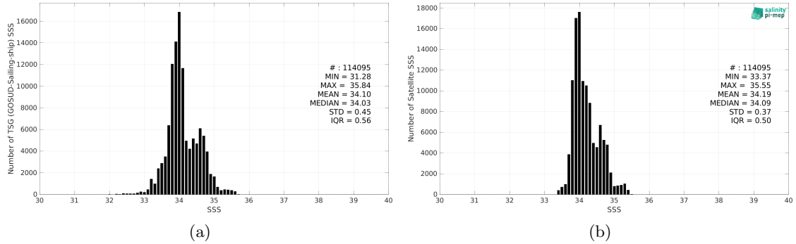
Figure 2: Histograms of SSS from TSG (GOSUD-Sailing-ship) (a) and SMAP SSS L4 OI v2 - Monthly (IPRC) (b) considering all match-up pairs per bins of 0.1 over the Roaring Forties and Furious Fifties Pi-MEP region and for the full satellite product period.
