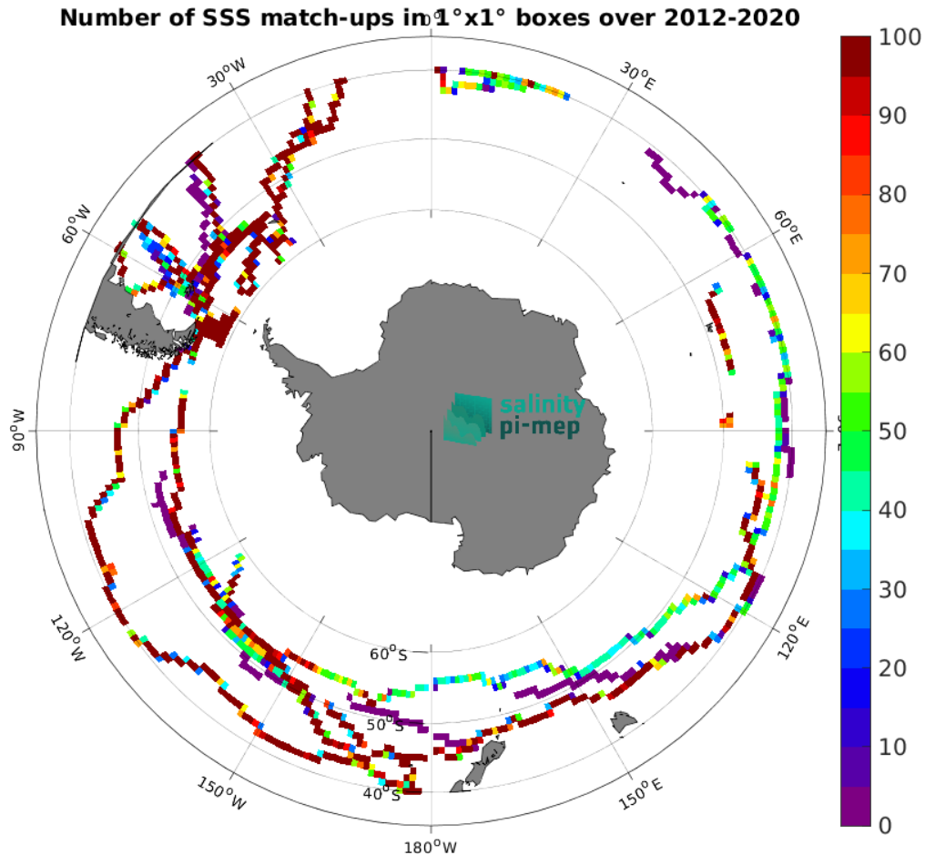
Figure 4: Number of SSS match-ups between TSG (GOSUD-Sailing-ship) SSS and the SMAP SSS L4 OI v2 - Monthly (IPRC) SSS product for the Roaring Forties and Furious Fifties Pi-MEP region over 1^\circ \times 1^\circ boxes and for the full satellite product period.
