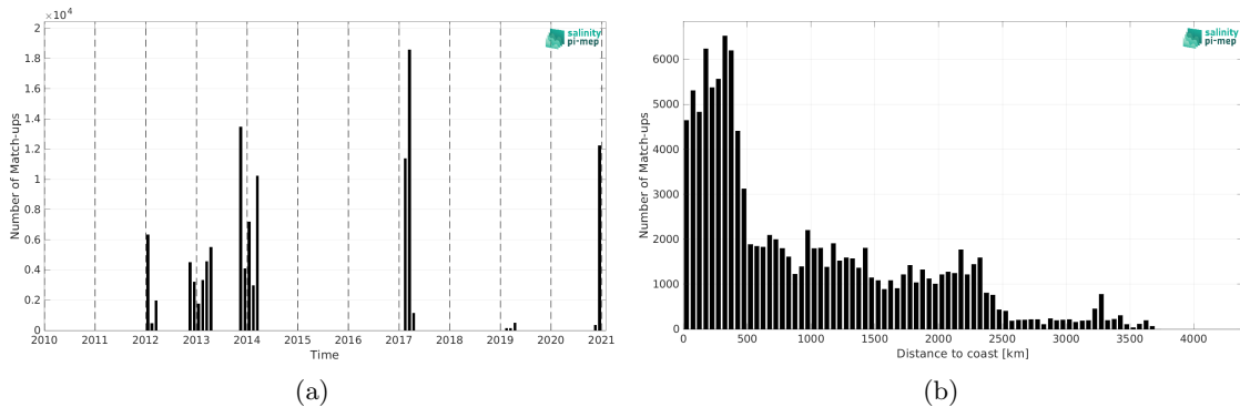
Figure 1: Number of match-ups between TSG (GOSUD-Sailing-ship) and SMAP SSS L4 OI v2 - Monthly (IPRC) SSS as a function of time (a) and as function of the distance to coast (b) over the Roaring Forties and Furious Fifties Pi-MEP region and for the full satellite product period.
