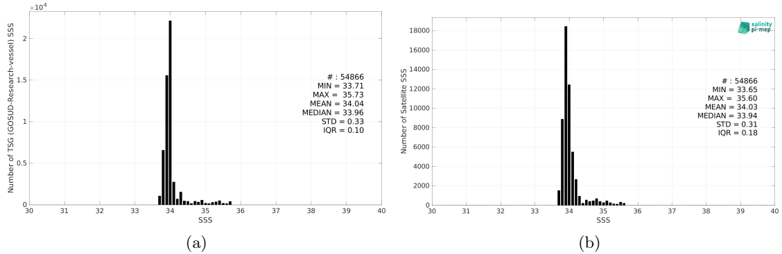
Figure 2: Histograms of SSS from TSG (GOSUD-Research-vessel) (a) and SMAP SSS L4 OI v2 - Monthly (IPRC) (b) considering all match-up pairs per bins of 0.1 over the Roaring Forties and Furious Fifties Pi-MEP region and for the full satellite product period.
