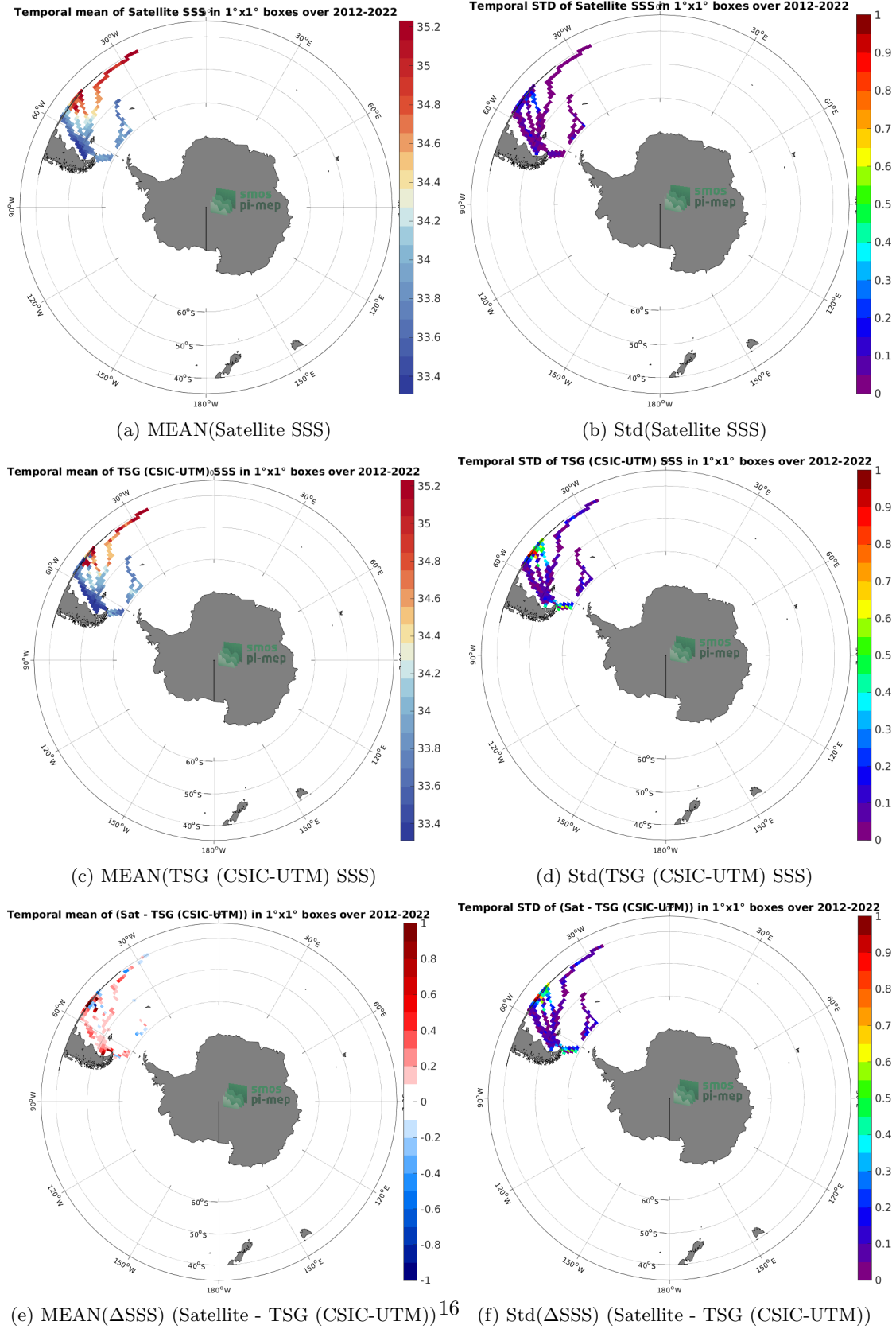
Figure 6: Temporal mean (left) and Std (right) of SSS from SMAP SSS L4 OI v2 - Monthly (IPRC) (top), TSG (CSIC-UTM) (middle), and of \Delta SSS (Satellite - TSG (CSIC-UTM)). Only match-up pairs are used to generate these maps.
