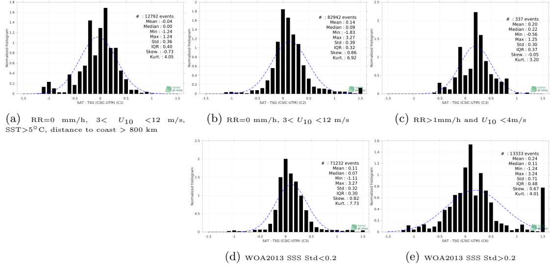
Figure 13: Normalized histogram of \Delta SSS (SMAP SSS L4 OI v2 - Monthly (IPRC) - TSG (CSIC-UTM)) for 5 different subdatasets corresponding to: RR=0 mm/h, 3 < U_{10} < 12 m/s, SST > 5°C, distance to coast > 800 km (a), RR=0 mm/h, 3 < U_{10} < 12 m/s (b), RR > 1mm/h and U_{10} < 4 m/s (c), WOA2013 SSS Std < 0.2 (d), WOA2013 SSS Std > 0.2 (e).
