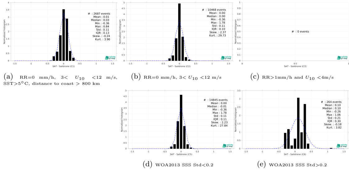
Figure 13: Normalized histogram of \Delta SSS (SMAP SSS L4 OI v2 - Monthly (IPRC) - Salsdrone) for 5 different subdatasets corresponding to: RR=0 mm/h, 3 < U_{10} < 12 m/s, SST > 5°C, distance to coast > 800 km (a), RR=0 mm/h, 3 < U_{10} < 12 m/s (b), RR > 1mm/h and U_{10} < 4 m/s (c), WOA2013 SSS Std < 0.2 (d), WOA2013 SSS Std > 0.2 (e).
