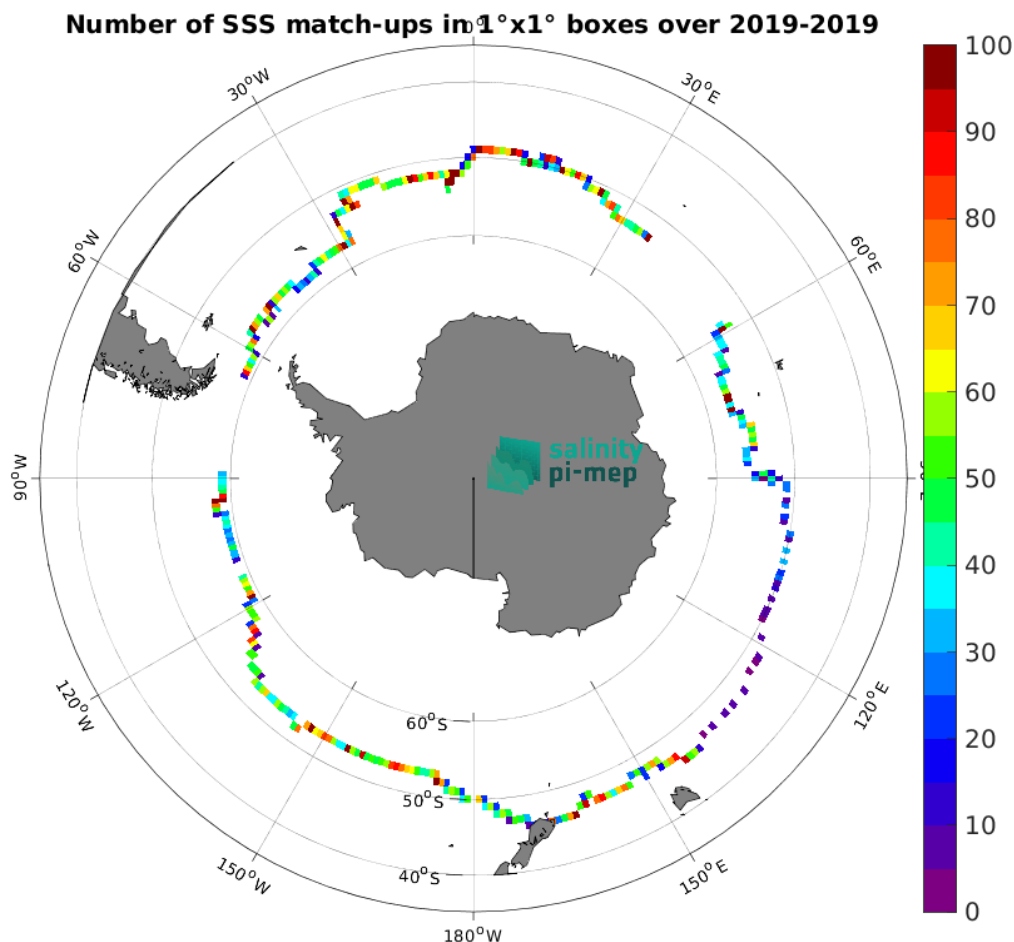
Figure 4: Number of SSS match-ups between Saildrone SSS and the SMAP SSS L4 OI v2 - Monthly (IPRC) SSS product for the Roaring Forties and Furious Fifties Pi-MEP region over 1^\circ \times 1^\circ boxes and for the full satellite product period.
