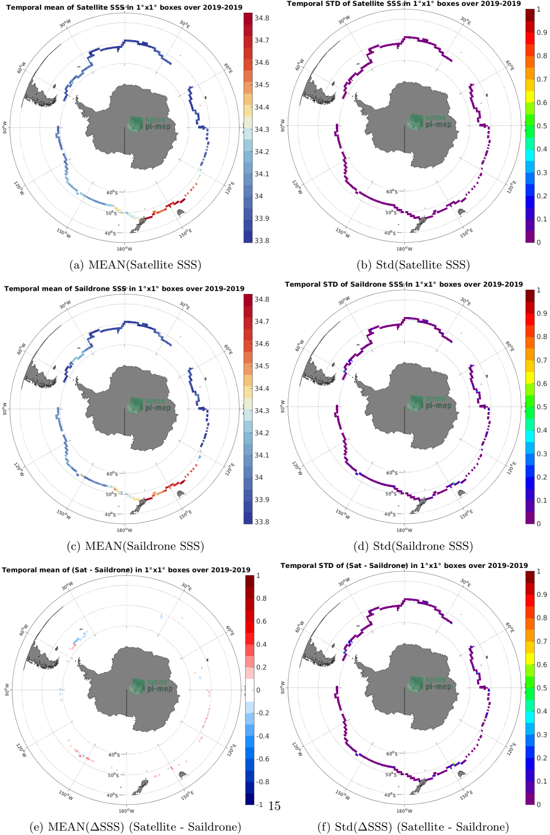
Figure 6: Temporal mean (left) and Std (right) of SSS from SMAP SSS L4 OI v2 - Monthly (IPRC) (top), Saildrone (middle), and of \Delta SSS (Satellite - Saildrone). Only match-up pairs are used to generate these maps.
