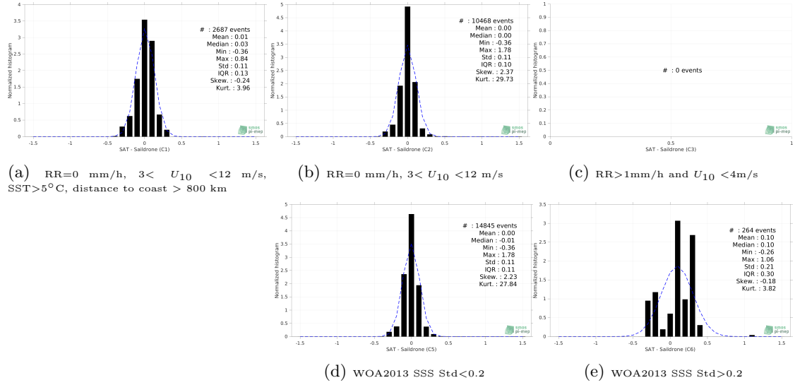
Figure 13: Normalized histogram of \Delta SSS (SMAP SSS L4 OI v2 - Monthly (IPRC) - Sairdrone) for 5 different subdatasets corresponding to: RR=0 mm/h, 3 < U_{10} < 12 m/s, SST > 5°C, distance to coast > 800 km (a), RR=0 mm/h, 3 < U_{10} < 12 m/s (b), RR > 1mm/h and U_{10} < 4 m/s (c), WOA2013 SSS Std < 0.2 (d), WOA2013 SSS Std > 0.2 (e).
