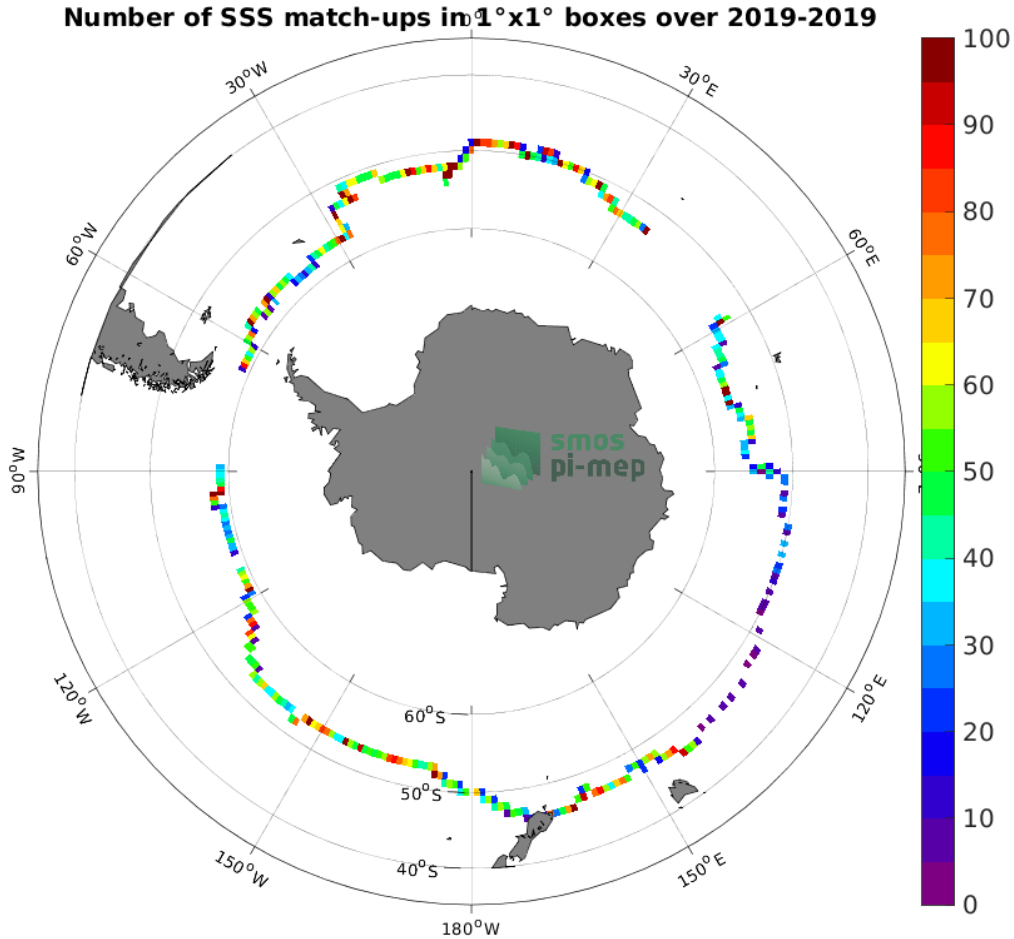
Figure 4: Number of SSS match-ups between Saildrone SSS and the SMAP SSS L4 OI v2 - Monthly (IPRC) SSS product for the Roaring Forties and Furious Fifties Pi-MEP region over 1^\circ \times 1^\circ boxes and for the full satellite product period.
