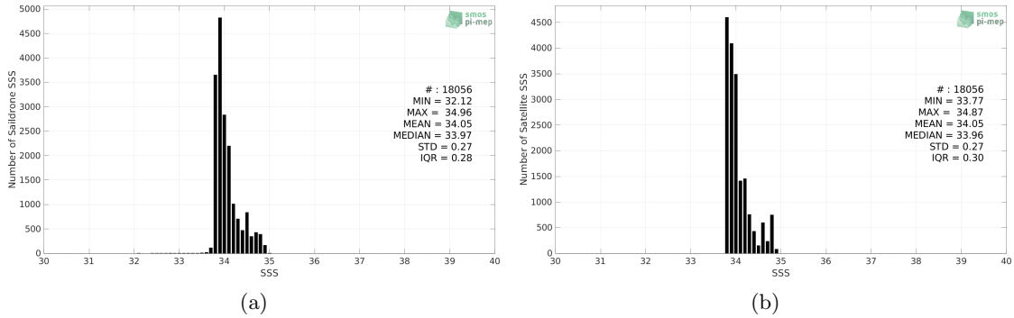
Figure 2: Histograms of SSS from Saildrone (a) and SMAP SSS L4 OI v2 - Monthly (IPRC) (b) considering all match-up pairs per bins of 0.1 over the Roaring Forties and Furious Fifties Pi-MEP region and for the full satellite product period.
