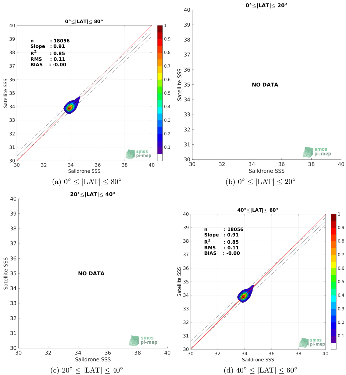
Figure 9: Contour maps of the concentration of SMAP SSS L4 OI v2 - Monthly (IPRC) SSS (y-axis) versus Saildrone SSS (x-axis) at match-up pairs for different latitude bands. For each plot, the red line shows x=y . The black thin and dashed lines indicate a linear fit through the data cloud and the \pm 95\% confidence levels, respectively. The number match-up pairs n , the slope and R^2 coefficient of the linear fit, the root mean square (RMS) and the mean bias between satellite and in situ data are indicated for each latitude band in each plots.
