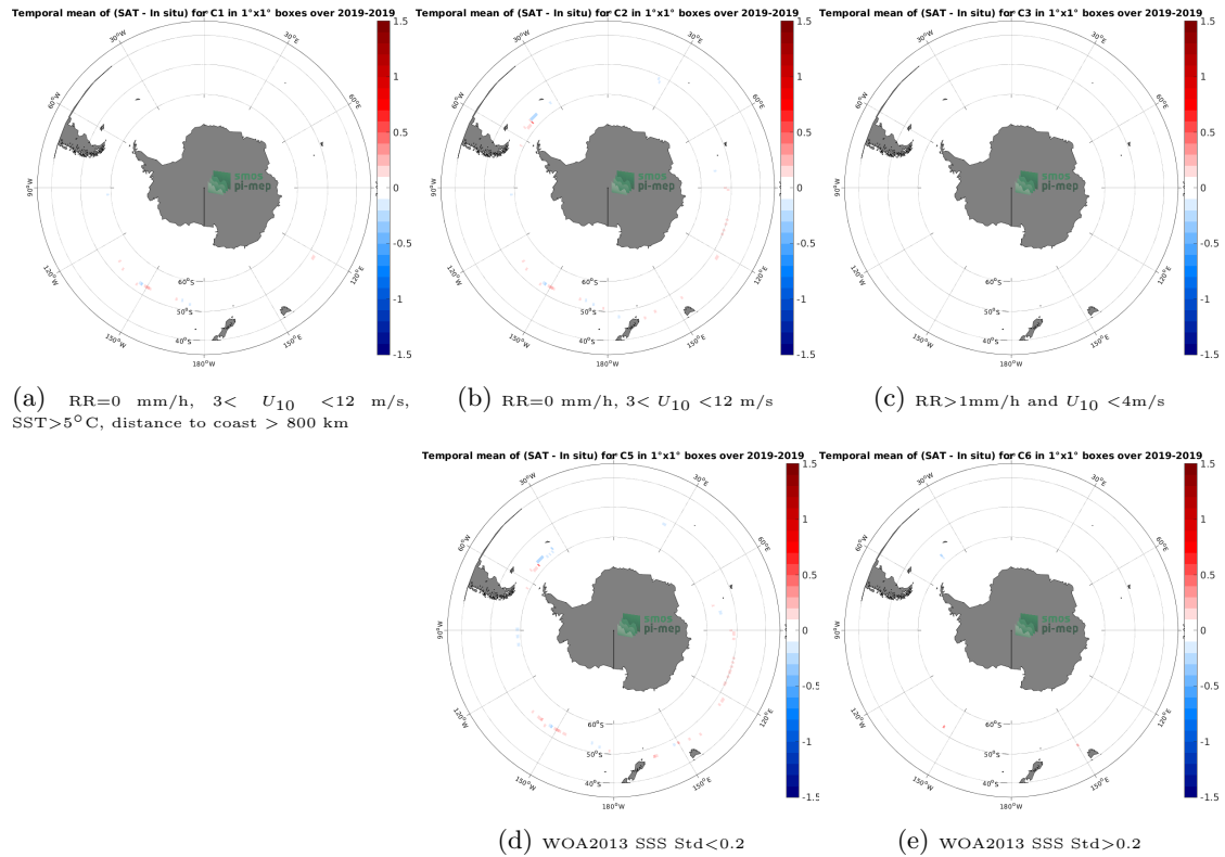
Figure 12: Temporal mean gridded over spatial boxes of size 1^{\circ}\times 1^{\circ} of \Delta\text{SSS} (SMAP SSS L4 OI v2 - Monthly (IPRC) - Saildrone) for 5 different subdatasets corresponding to:RR=0 mm/h, 3 < U_{10} < 12 m/s, SST >5^{\circ}\text{C} , distance to coast > 800 km (a), RR=0 mm/h, 3 < U_{10} < 12 m/s (b), RR >1 mm/h and U_{10} < 4 m/s (c), WOA2013 SSS Std <0.2 (d), WOA2013 SSS Std >0.2 (e).
