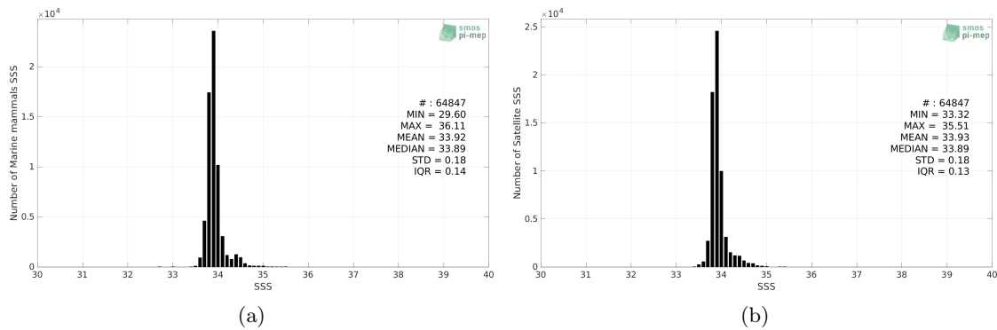
Figure 2: Histograms of SSS from Marine mammals (a) and SMAP SSS L4 OI v2 - Monthly (IPRC) (b) considering all match-up pairs per bins of 0.1 over the Roaring Forties and Furious Fifties Pi-MEP region and for the full satellite product period.
