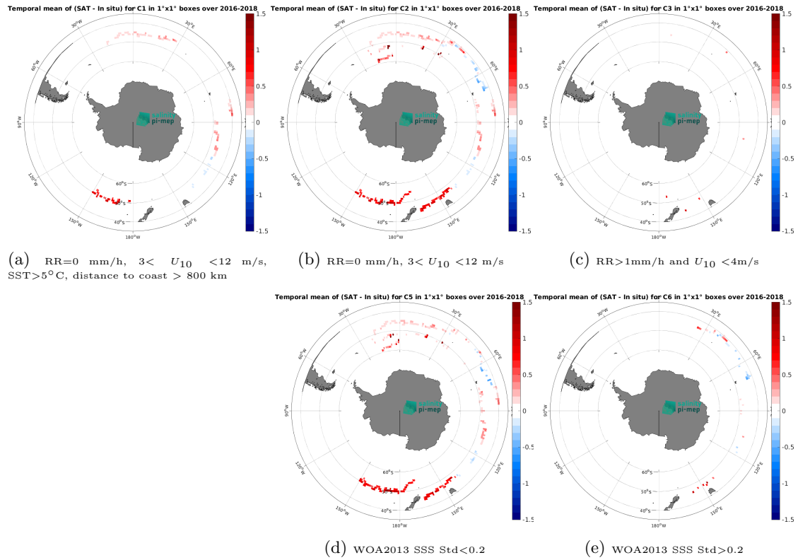
Figure 11: Temporal mean gridded over spatial boxes of size 1^{\circ}\times 1^{\circ} of \Delta\text{SSS} (SMAP SSS L4 OI v2 - Monthly (IPRC) - Surface drifters) for 5 different subdatasets corresponding to:RR=0 mm/h, 3 < U_{10} < 12 m/s, SST >5^{\circ}\text{C} , distance to coast > 800 km (a), RR=0 mm/h, 3 < U_{10} < 12 m/s (b), RR >1 mm/h and U_{10} < 4 m/s (c), WOA2013 SSS Std <0.2 (d), WOA2013 SSS Std >0.2 (e).
