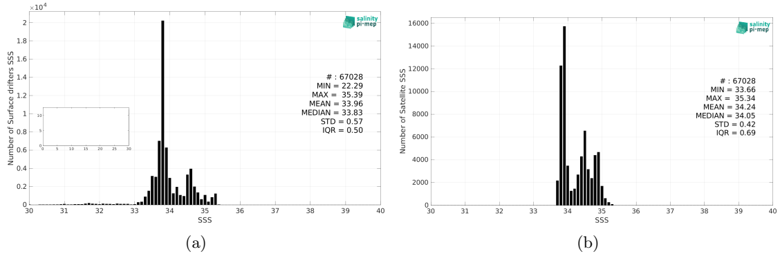
Figure 2: Histograms of SSS from Surface drifters (a) and SMAP SSS L4 OI v2 - Monthly (IPRC) (b) considering all match-up pairs per bins of 0.1 over the Roaring Forties and Furious Fifties Pi-MEP region and for the full satellite product period.
