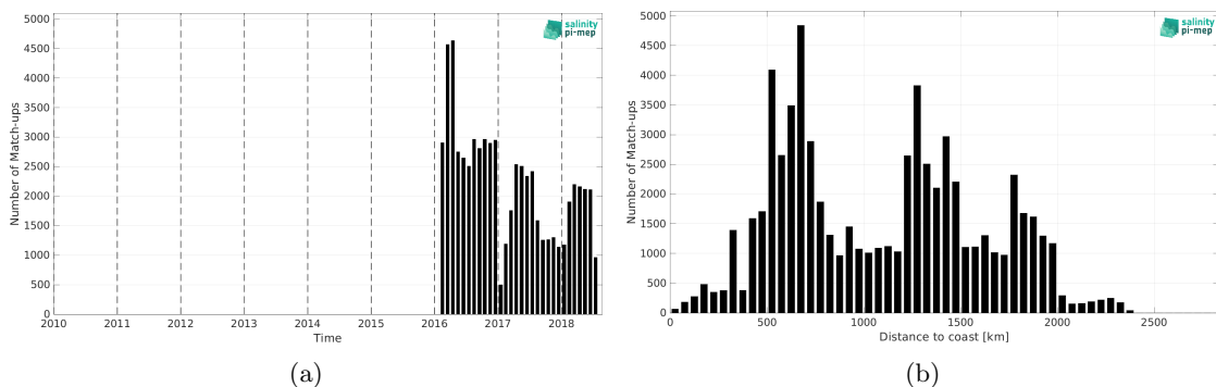
Figure 1: Number of match-ups between Surface drifters and SMAP SSS L4 OI v2 - Monthly (IPRC) SSS as a function of time (a) and as function of the distance to coast (b) over the Roaring Forties and Furious Fifties Pi-MEP region and for the full satellite product period.
