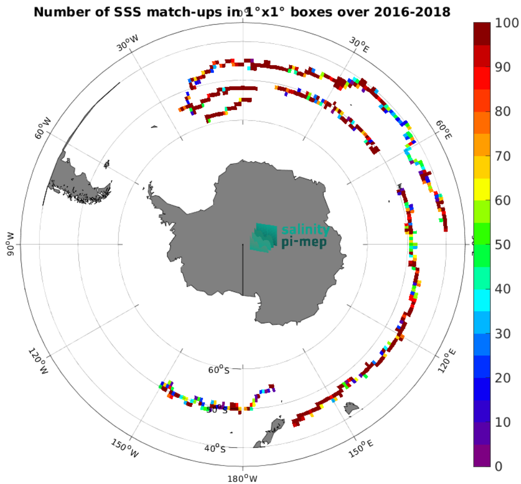
Figure 3: Number of SSS match-ups between Surface drifters SSS and the SMAP SSS L4 OI v2 - Monthly (IPRC) SSS product for the Roaring Forties and Furious Fifties Pi-MEP region over 1^\circ \times 1^\circ boxes and for the full satellite product period.
