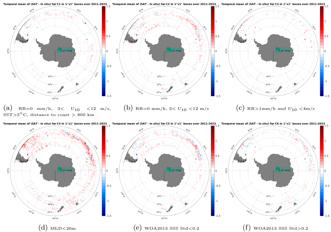
Figure 12: Temporal mean gridded over spatial boxes of size 1^{\circ}\times 1^{\circ} of \Delta\text{SSS} (SMAP SSS L4 OI v2 - Monthly (IPRC) - Argo) for 6 different subdatasets corresponding to:RR=0 mm/h, 3 < U_{10} < 12 m/s, SST > 5^{\circ}\text{C} , distance to coast > 800 km (a), RR=0 mm/h, 3 < U_{10} < 12 m/s (b), RR > 1\text{mm/h} and U_{10} < 4\text{m/s} (c),MLD < 20\text{m} (d),WOA2013 SSS Std < 0.2 (e),WOA2013 SSS Std > 0.2 (f).
