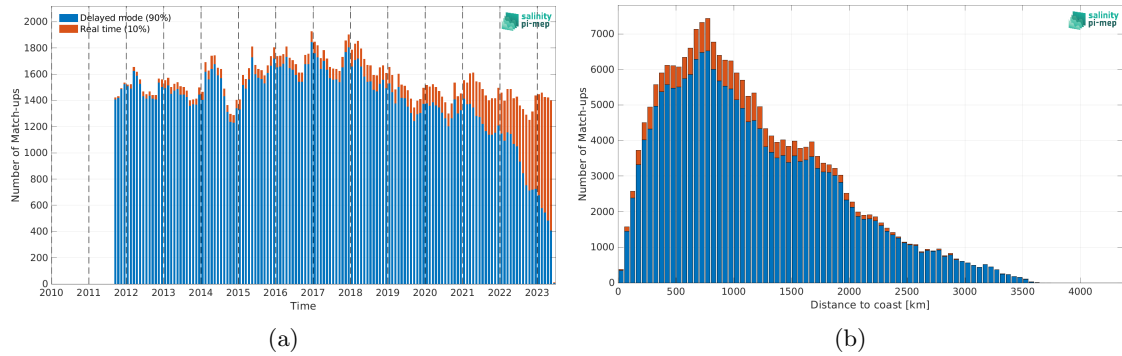
Figure 1: Number of match-ups between Argo and SMAP SSS L4 OI v2 - Monthly (IPRC) SSS as a function of time (a) and as function of the distance to coast (b) over the Roaring Forties and Furious Fifties Pi-MEP region and for the full satellite product period.
