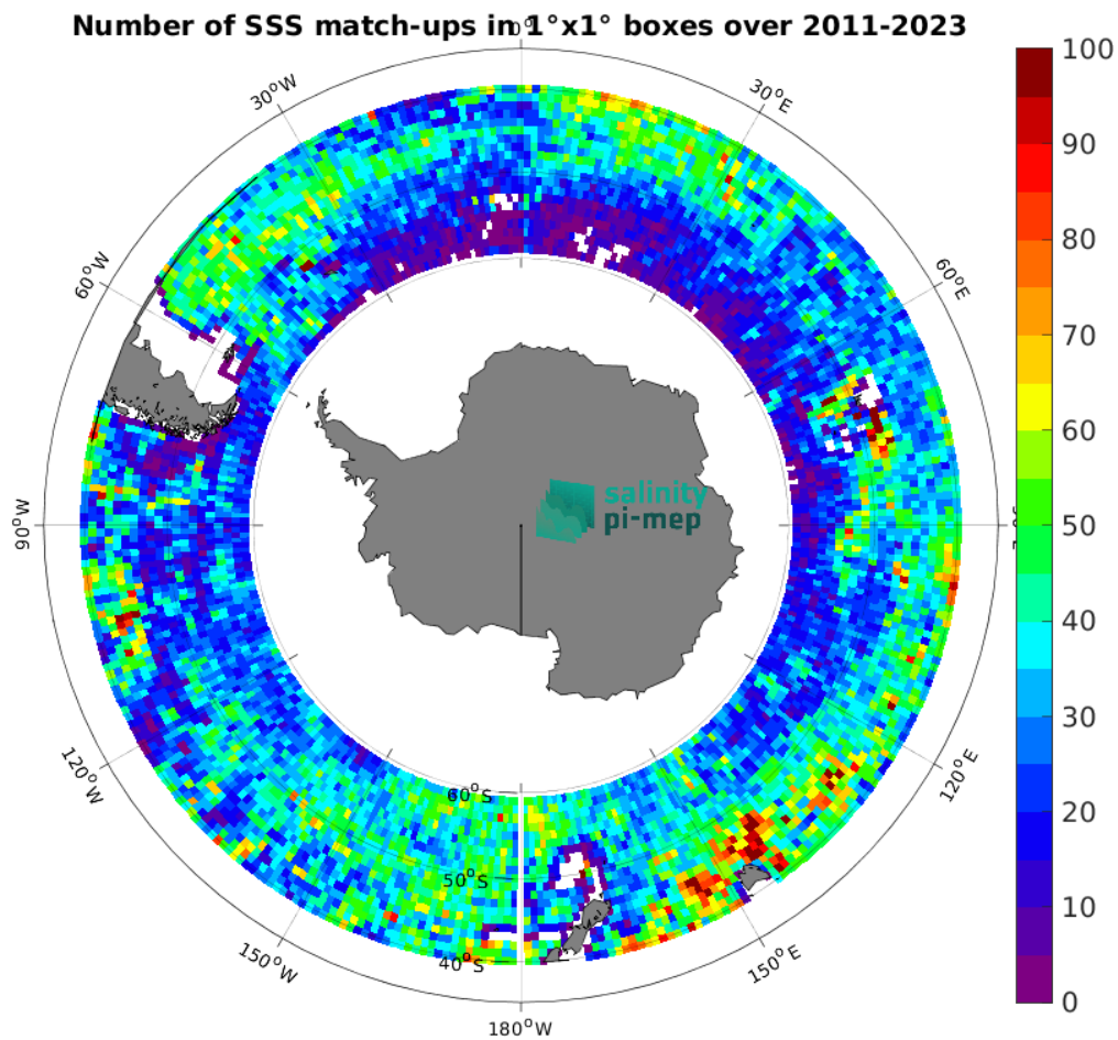
Figure 4: Number of SSS match-ups between Argo SSS and the SMAP SSS L4 OI v2 - Monthly (IPRC) SSS product for the Roaring Forties and Furious Fifties Pi-MEP region over 1^{\circ} \times 1^{\circ} boxes and for the full satellite product period.
