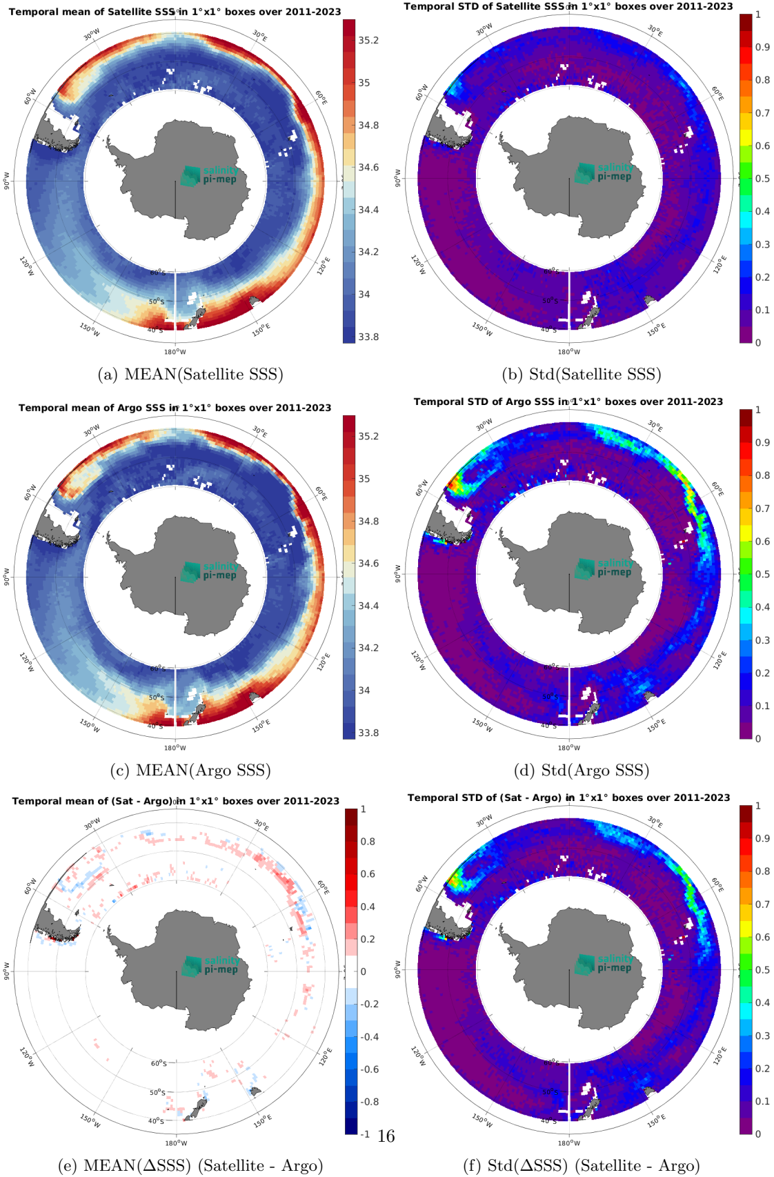
Figure 6: Temporal mean (left) and Std (right) of SSS from SMAP SSS L4 OI v2 - Monthly (IPRC) (top), Argo (middle), and of \Delta SSS (Satellite - Argo). Only match-up pairs are used to generate these maps.
