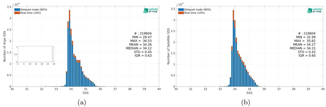
Figure 2: Histograms of SSS from Argo (a) and SMAP SSS L4 OI v2 - Monthly (IPRC) (b) considering all match-up pairs per bins of 0.1 over the Roaring Forties and Furious Fifties Pi-MEP region and for the full satellite product period.
