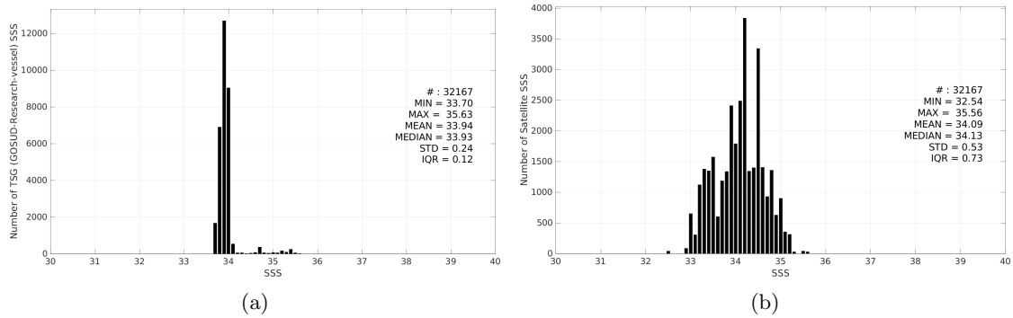
Figure 3: Histograms of SSS from TSG (GOSUD-Research-vessel) (a) and SMAP SSS L3 v6 - 8-Day running (RSS) (b) considering all match-up pairs per bins of 0.1 over the Roaring Forties and Furious Fifties Pi-MEP region and for the full satellite product period.
