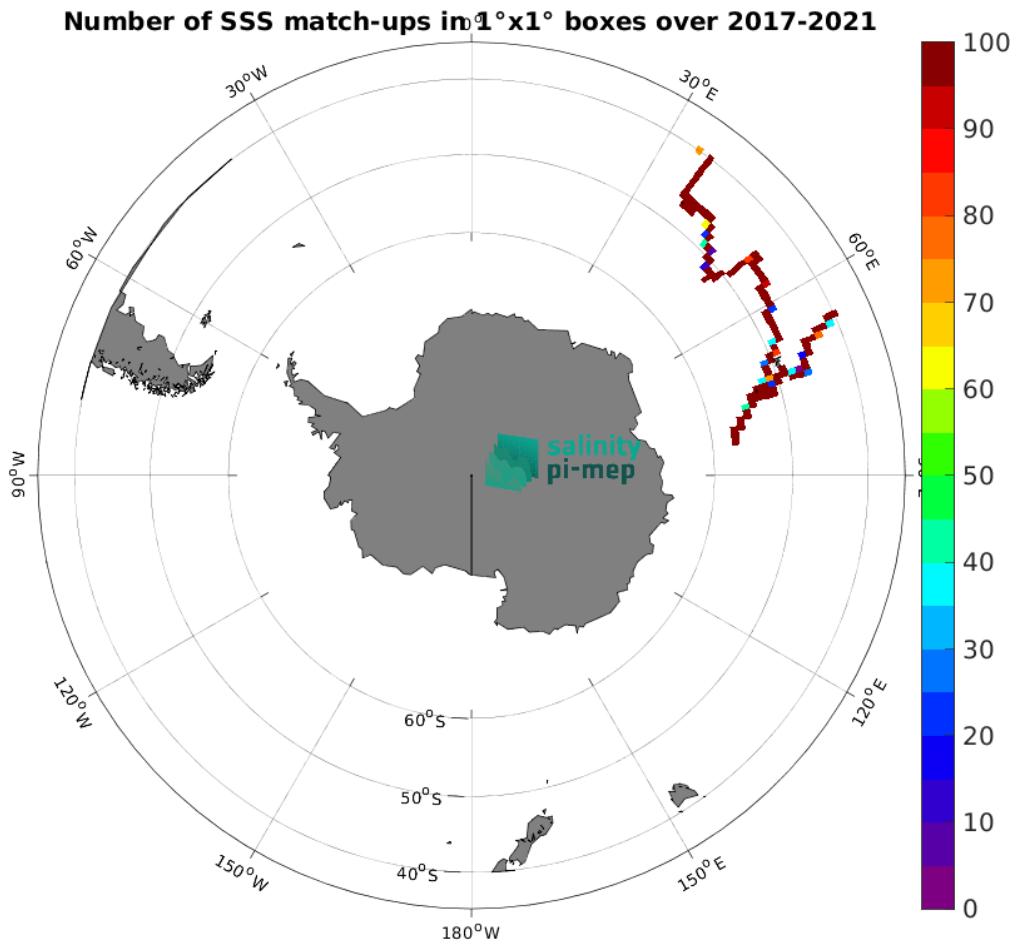
Figure 5: Number of SSS match-ups between TSG (GOSUD-Research-vessel) SSS and the SMAP SSS L3 v6 - 8-Day running (RSS) SSS product for the Roaring Forties and Furious Fifties Pi-MEP region over 1^\circ \times 1^\circ boxes and for the full satellite product period.
