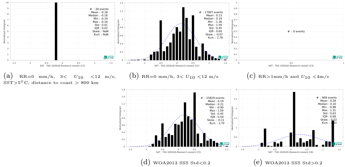
Figure 15: Normalized histogram of \Delta SSS (SMAP SSS L3 v6 - 8-Day running (RSS) - TSG (GOSUD-Research-vessel)) for 5 different subdatasets corresponding to: RR=0 mm/h, 3 < U_{10} < 12 m/s, SST > 5°C, distance to coast > 800 km (a), RR=0 mm/h, 3 < U_{10} < 12 m/s (b), RR > 1mm/h and U_{10} < 4 m/s (c), WOA2013 SSS Std < 0.2 (d), WOA2013 SSS Std > 0.2 (e).
