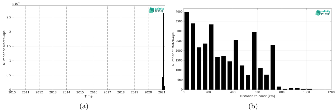
Figure 2: Number of match-ups between TSG (GOSUD-Research-vessel) and SMAP SSS L3 v6 - 8-Day running (RSS) SSS as a function of time (a) and as function of the distance to coast (b) over the Roaring Forties and Furious Fifties Pi-MEP region and for the full satellite product period.
