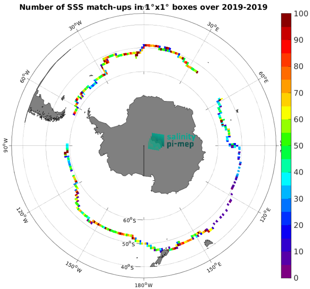
Figure 5: Number of SSS match-ups between Saildrone SSS and the SMAP SSS L3 v6 - Monthly (RSS) SSS product for the Roaring Forties and Furious Fifties Pi-MEP region over 1^{\circ} \times 1^{\circ} boxes and for the full satellite product period.
