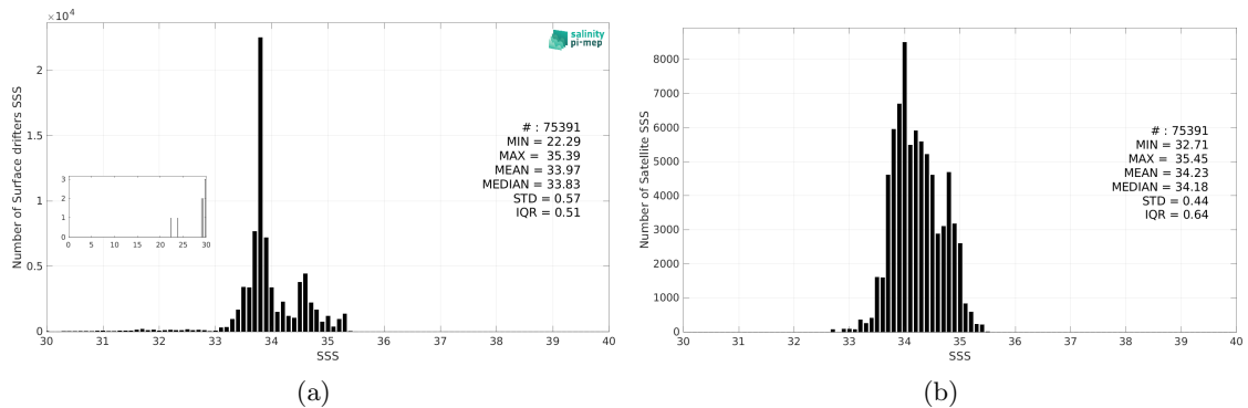
Figure 3: Histograms of SSS from Surface drifters (a) and SMAP SSS L3 v6 - Monthly (RSS) (b) considering all match-up pairs per bins of 0.1 over the Roaring Forties and Furious Fifties Pi-MEP region and for the full satellite product period.
