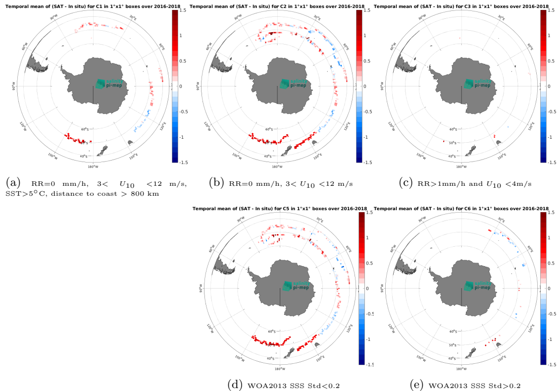
Figure 13: Temporal mean gridded over spatial boxes of size 1^\circ \times 1^\circ of \Delta\text{SSS} (SMAP SSS L3 v6 - Monthly (RSS) - Surface drifters) for 5 different subdatasets corresponding to:RR=0 mm/h, 3 < U_{10} < 12 m/s, SST > 5^\circ\text{C} , distance to coast > 800 km (a), RR=0 mm/h, 3 < U_{10} < 12 m/s (b), RR > 1 mm/h and U_{10} < 4 m/s (c), WOA2013 SSS Std < 0.2 (d), WOA2013 SSS Std > 0.2 (e).
