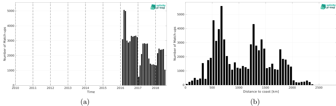
Figure 2: Number of match-ups between Surface drifters and SMAP SSS L3 v6 - Monthly (RSS) SSS as a function of time (a) and as function of the distance to coast (b) over the Roaring Forties and Furious Fifties Pi-MEP region and for the full satellite product period.
