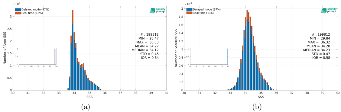
Figure 3: Histograms of SSS from Argo (a) and SMAP SSS L3 v6 - Monthly (RSS) (b) considering all match-up pairs per bins of 0.1 over the Roaring Forties and Furious Fifties Pi-MEP region and for the full satellite product period.
