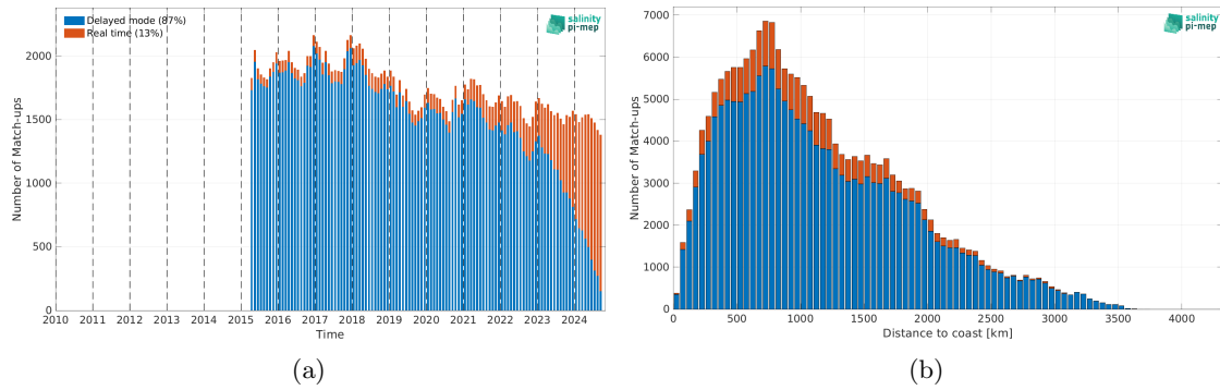
Figure 2: Number of match-ups between Argo and SMAP SSS L3 v6 - Monthly (RSS) SSS as a function of time (a) and as function of the distance to coast (b) over the Roaring Forties and Furious Fifties Pi-MEP region and for the full satellite product period.
