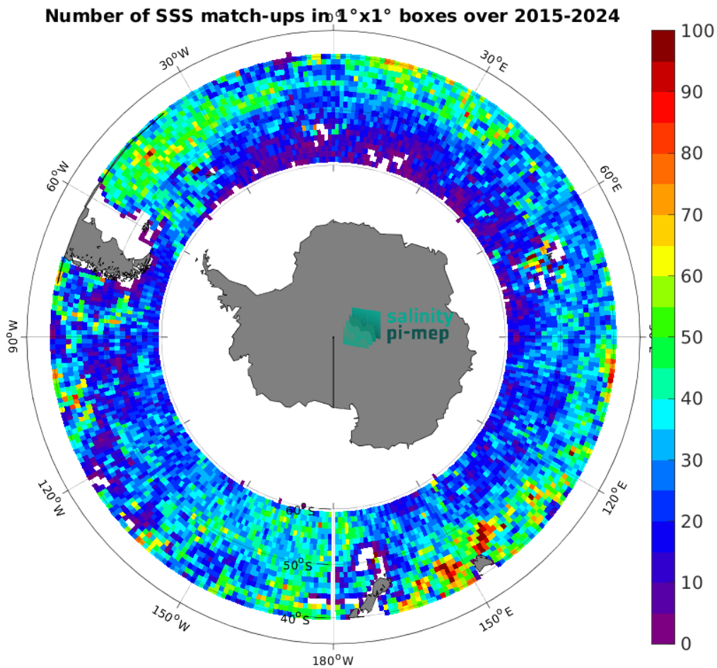
Figure 5: Number of SSS match-ups between Argo SSS and the SMAP SSS L3 v6 - Monthly (RSS) SSS product for the Roaring Forties and Furious Fifties Pi-MEP region over 1^\circ \times 1^\circ boxes and for the full satellite product period.
