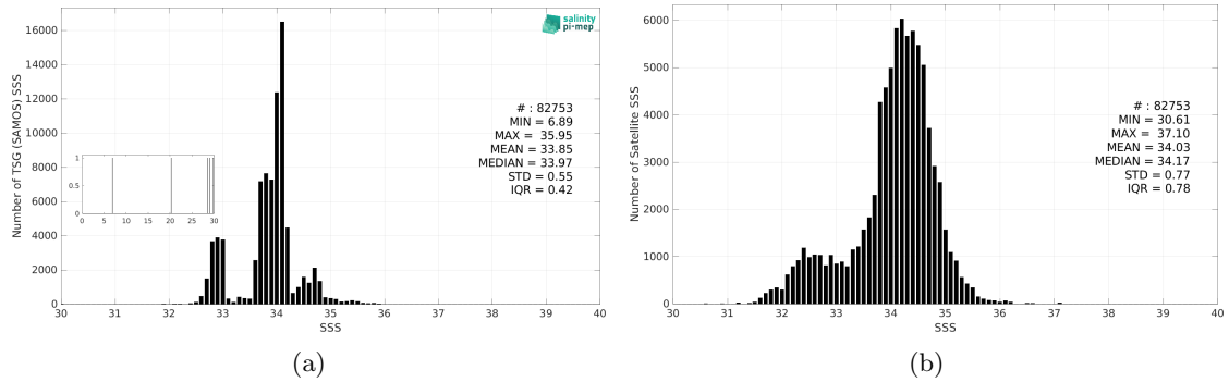
Figure 3: Histograms of SSS from TSG (SAMOS) (a) and SMAP SSS L3 v5.3 - 8-Day running (RSS) (b) considering all match-up pairs per bins of 0.1 over the Roaring Forties and Furious Fifties Pi-MEP region and for the full satellite product period.
