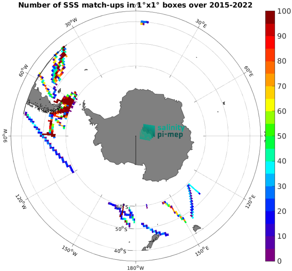
Figure 5: Number of SSS match-ups between TSG (SAMOS) SSS and the SMAP SSS L3 v5.3 - 8-Day running (RSS) SSS product for the Roaring Forties and Furious Fifties Pi-MEP region over 1^\circ \times 1^\circ boxes and for the full satellite product period.
