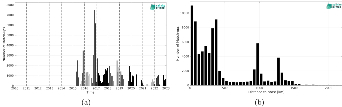
Figure 2: Number of match-ups between TSG (SAMOS) and SMAP SSS L3 v5.3 - 8-Day running (RSS) SSS as a function of time (a) and as function of the distance to coast (b) over the Roaring Forties and Furious Fifties Pi-MEP region and for the full satellite product period.
