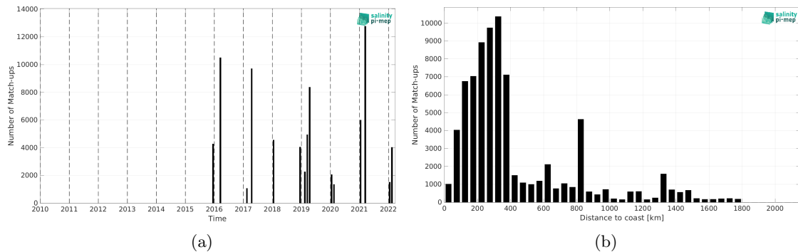
Figure 2: Number of match-ups between TSG (CSIC-UTM) and SMAP SSS L3 v5.3 - 8-Day running (RSS) SSS as a function of time (a) and as function of the distance to coast (b) over the Roaring Forties and Furious Fifties Pi-MEP region and for the full satellite product period.
