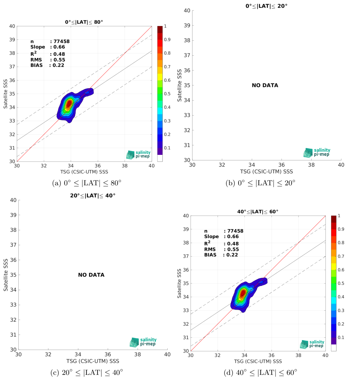
Figure 10: Contour maps of the concentration of SMAP SSS L3 v5.3 - 8-Day running (RSS) SSS (y-axis) versus TSG (CSIC-UTM) SSS (x-axis) at match-up pairs for different latitude bands. For each plot, the red line shows x=y . The black thin and dashed lines indicate a linear fit through the data cloud and the \pm 95\% confidence levels, respectively. The number match-up pairs n , the slope and R^2 coefficient of the linear fit, the root mean square (RMS) and the mean bias between satellite and in situ data are indicated for each latitude band in each plot.
