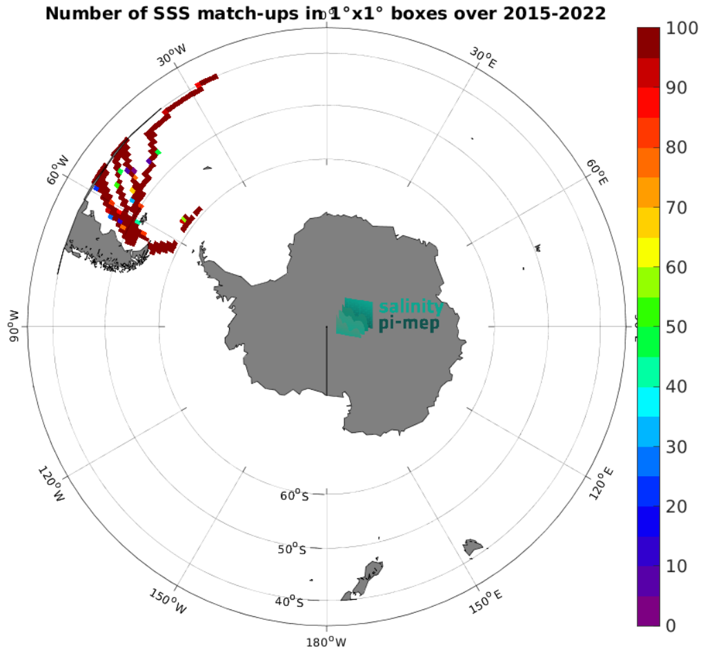
Figure 5: Number of SSS match-ups between TSG (CSIC-UTM) SSS and the SMAP SSS L3 v5.3 - 8-Day running (RSS) SSS product for the Roaring Forties and Furious Fifties Pi-MEP region over 1^\circ \times 1^\circ boxes and for the full satellite product period.
