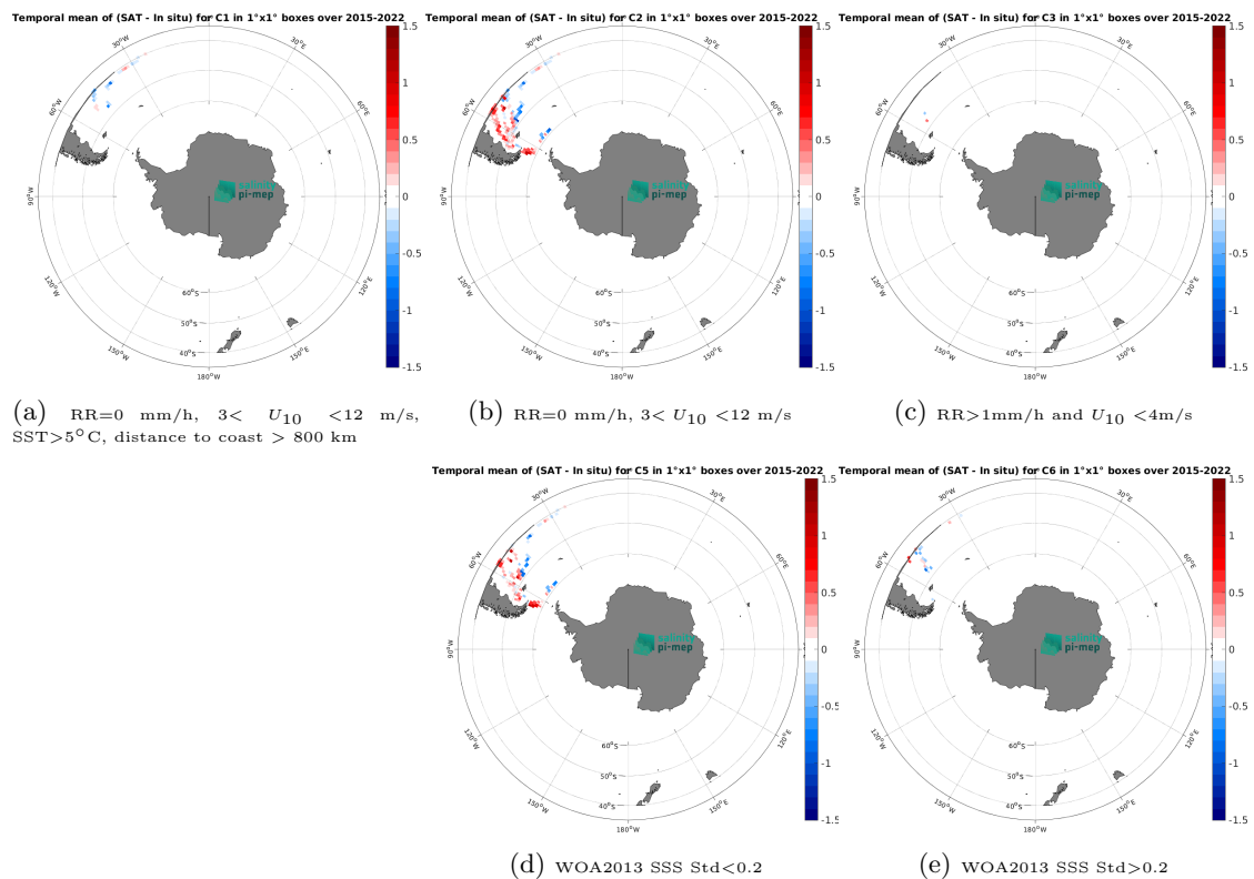
Figure 14: Temporal mean gridded over spatial boxes of size 1^\circ \times 1^\circ of \Delta SSS (SMAP SSS L3 v5.3 - 8-Day running (RSS) - TSG (CSIC-UTM)) for 5 different subdatasets corresponding to:RR=0 mm/h, 3 < U_{10} < 12 m/s, SST > 5^\circ\text{C} , distance to coast > 800 km (a), RR=0 mm/h, 3 < U_{10} < 12 m/s (b), RR > 1 mm/h and U_{10} < 4 m/s (c), WOA2013 SSS Std < 0.2 (d), WOA2013 SSS Std > 0.2 (e).
