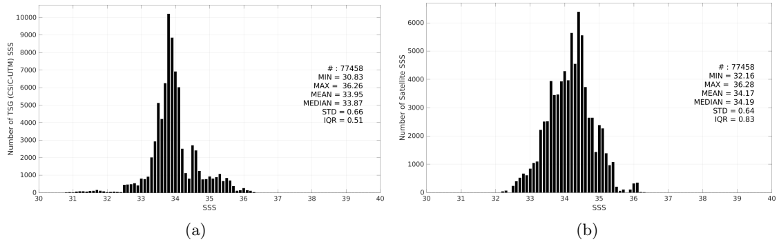
Figure 3: Histograms of SSS from TSG (CSIC-UTM) (a) and SMAP SSS L3 v5.3 - 8-Day running (RSS) (b) considering all match-up pairs per bins of 0.1 over the Roaring Forties and Furious Fifties Pi-MEP region and for the full satellite product period.
