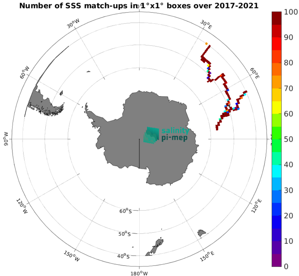
Figure 5: Number of SSS match-ups between TSG (GOSUD-Research-vessel) SSS and the SMAP SSS L3 v5.3 - Monthly (RSS) SSS product for the Roaring Forties and Furious Fifties Pi-MEP region over 1^\circ \times 1^\circ boxes and for the full satellite product period.
