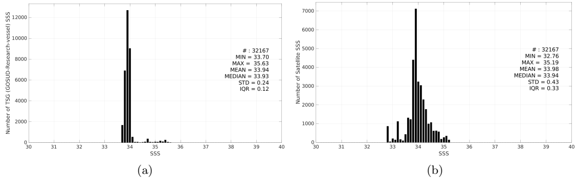
Figure 3: Histograms of SSS from TSG (GOSUD-Research-vessel) (a) and SMAP SSS L3 v5.3 - Monthly (RSS) (b) considering all match-up pairs per bins of 0.1 over the Roaring Forties and Furious Fifties Pi-MEP region and for the full satellite product period.
