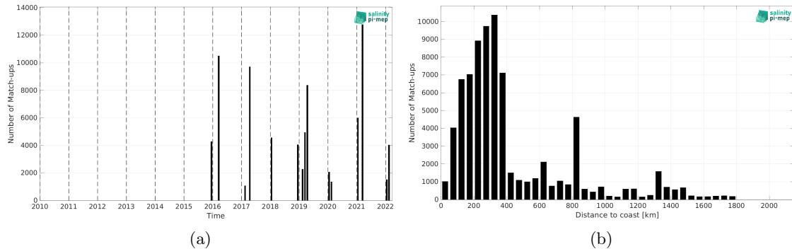
Figure 2: Number of match-ups between TSG (CSIC-UTM) and SMAP SSS L3 v5.3 - Monthly (RSS) SSS as a function of time (a) and as function of the distance to coast (b) over the Roaring Forties and Furious Fifties Pi-MEP region and for the full satellite product period.
