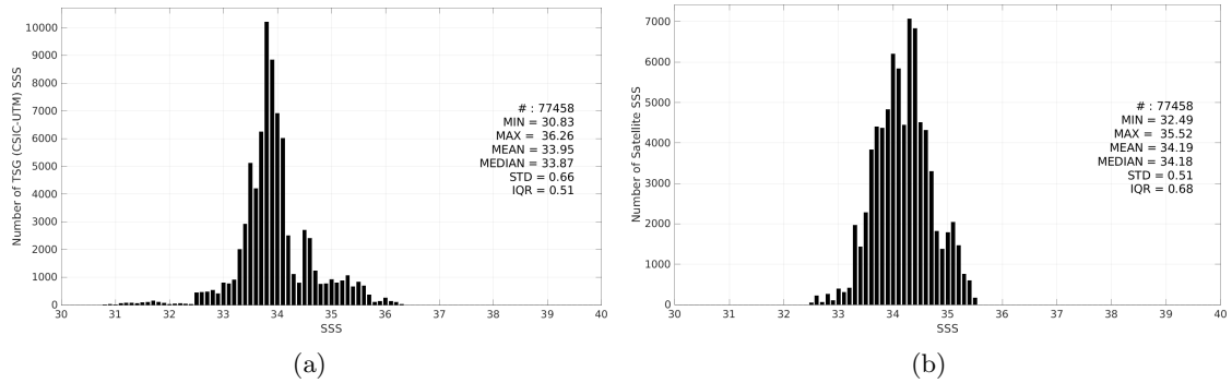
Figure 3: Histograms of SSS from TSG (CSIC-UTM) (a) and SMAP SSS L3 v5.3 - Monthly (RSS) (b) considering all match-up pairs per bins of 0.1 over the Roaring Forties and Furious Fifties Pi-MEP region and for the full satellite product period.
