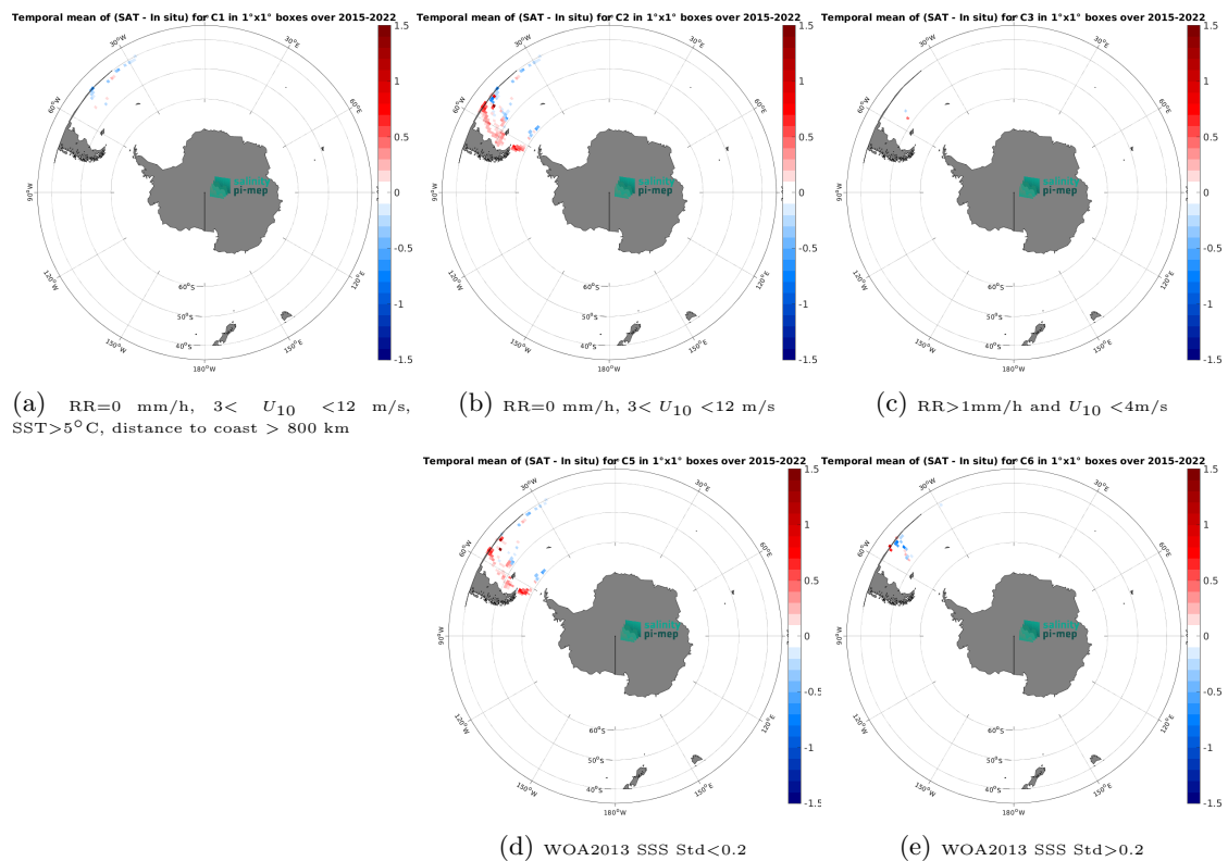
Figure 14: Temporal mean gridded over spatial boxes of size 1^\circ \times 1^\circ of \Delta SSS (SMAP SSS L3 v5.3 - Monthly (RSS) - TSG (CSIC-UTM)) for 5 different subdatasets corresponding to:RR=0 mm/h, 3 < U_{10} < 12 m/s, SST>5°C, distance to coast > 800 km (a), RR=0 mm/h, 3 < U_{10} < 12 m/s (b), RR>1mm/h and U_{10} < 4 m/s (c), WOA2013 SSS Std<0.2 (d), WOA2013 SSS Std>0.2 (e).
