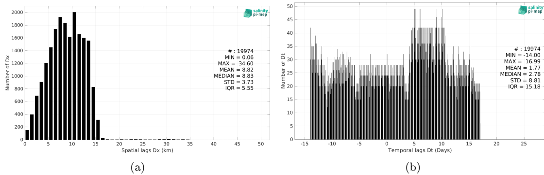
Figure 6: Histograms of the spatial (a) and temporal (b) lags between the location/time of the Saildrone measurement and the date of the corresponding SMAP SSS L3 v5.3 - Monthly (RSS) SSS pixel.
