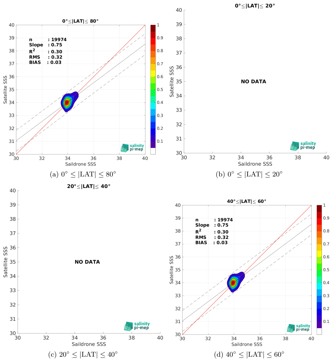
Figure 10: Contour maps of the concentration of SMAP SSS L3 v5.3 - Monthly (RSS) SSS (y-axis) versus Saildrone SSS (x-axis) at match-up pairs for different latitude bands. For each plot, the red line shows x=y . The black thin and dashed lines indicate a linear fit through the data cloud and the \pm 95\% confidence levels, respectively. The number match-up pairs n , the slope and R^2 coefficient of the linear fit, the root mean square (RMS) and the mean bias between satellite and in situ data are indicated for each latitude band in each plots.
