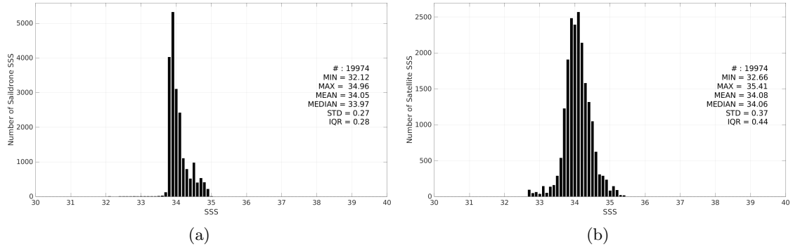
Figure 3: Histograms of SSS from Saildrone (a) and SMAP SSS L3 v5.3 - Monthly (RSS) (b) considering all match-up pairs per bins of 0.1 over the Roaring Forties and Furious Fifties Pi-MEP region and for the full satellite product period.
