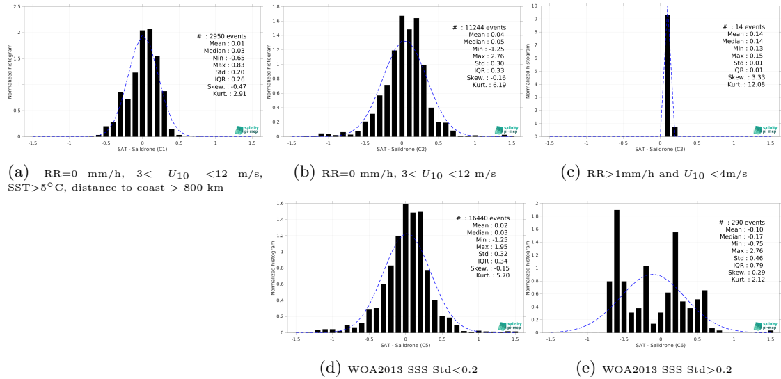
Figure 15: Normalized histogram of \Delta SSS (SMAP SSS L3 v5.3 - Monthly (RSS) - Saldrone) for 5 different subdatasets corresponding to: RR=0 mm/h, 3 < U_{10} < 12 m/s, SST>5°C, distance to coast > 800 km (a), RR=0 mm/h, 3 < U_{10} < 12 m/s (b), RR>1mm/h and U_{10} < 4 m/s (c), WOA2013 SSS Std<0.2 (d), WOA2013 SSS Std>0.2 (e).
