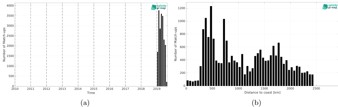
Figure 2: Number of match-ups between Saildrone and SMAP SSS L3 v5.3 - Monthly (RSS) SSS as a function of time (a) and as function of the distance to coast (b) over the Roaring Forties and Furious Fifties Pi-MEP region and for the full satellite product period.
