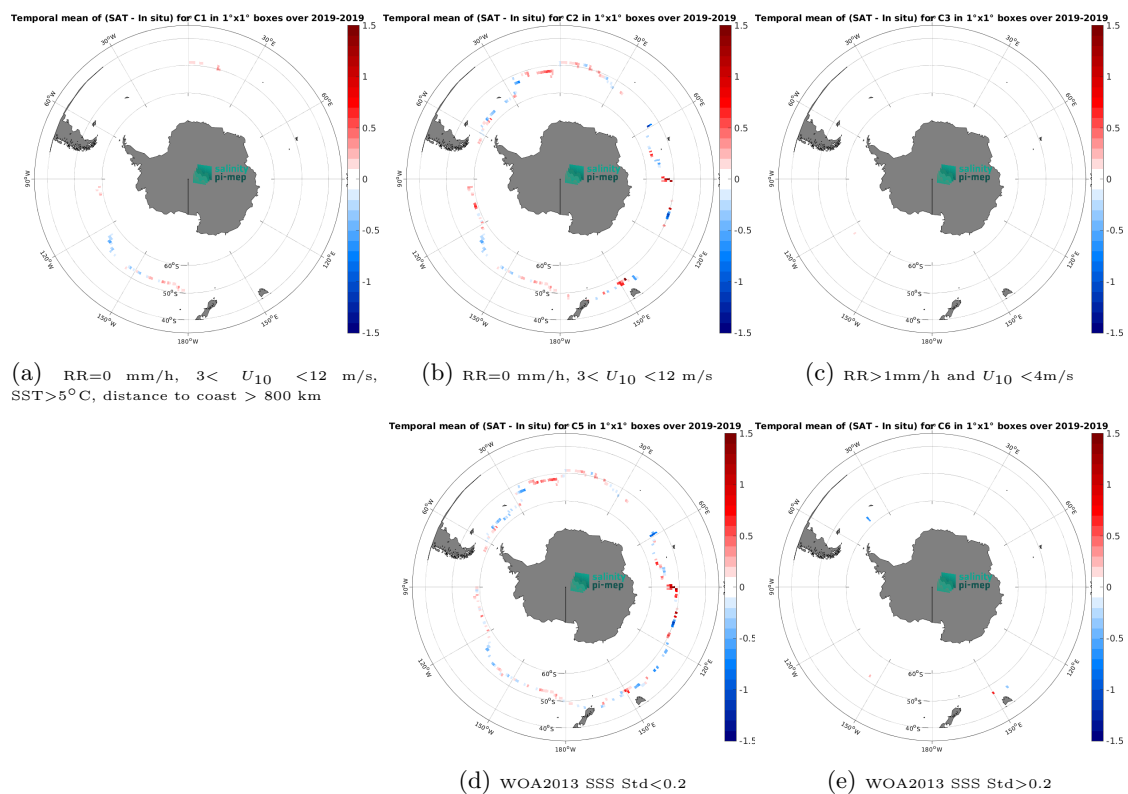
Figure 14: Temporal mean gridded over spatial boxes of size 1^\circ \times 1^\circ of \Delta\text{SSS} (SMAP SSS L3 v5.3 - Monthly (RSS) - Saildrone) for 5 different subdatasets corresponding to:RR=0 mm/h, 3 < U_{10} < 12 m/s, SST>5°C, distance to coast > 800 km (a), RR=0 mm/h, 3 < U_{10} < 12 m/s (b), RR>1mm/h and U_{10} < 4 m/s (c), WOA2013 SSS Std<0.2 (d), WOA2013 SSS Std>0.2 (e).
