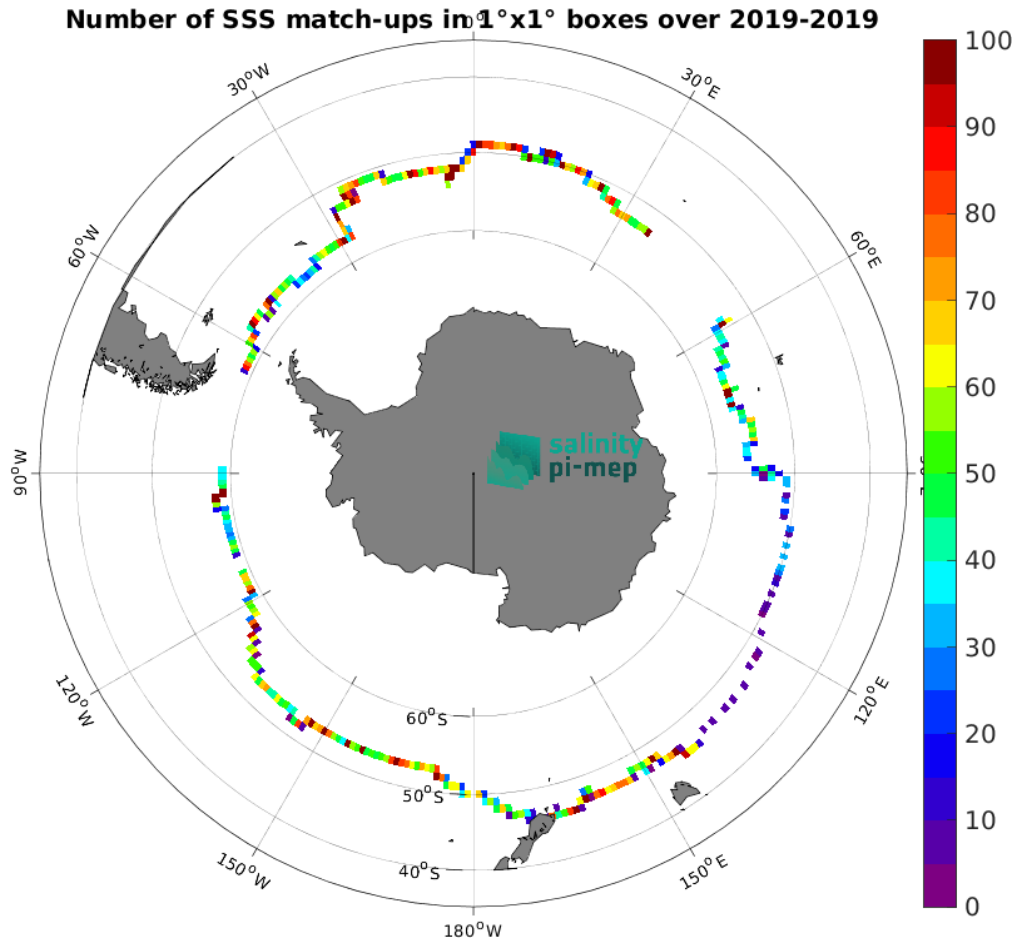
Figure 5: Number of SSS match-ups between Saildrone SSS and the SMAP SSS L3 v5.3 - Monthly (RSS) SSS product for the Roaring Forties and Furious Fifties Pi-MEP region over 1^\circ \times 1^\circ boxes and for the full satellite product period.
