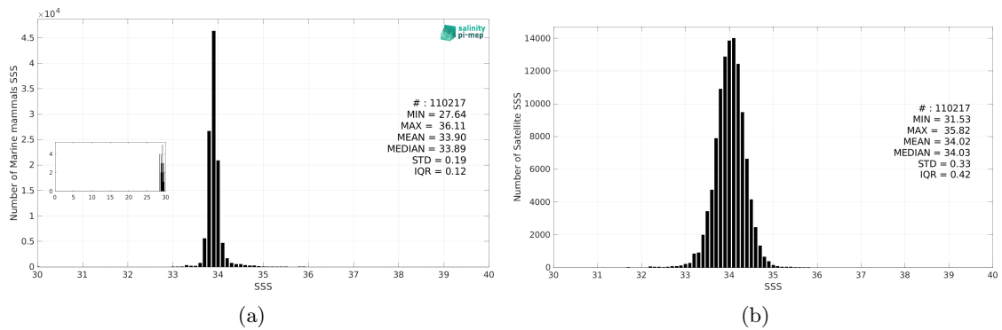
Figure 3: Histograms of SSS from Marine mammals (a) and SMAP SSS L3 v5.3 - Monthly (RSS) (b) considering all match-up pairs per bins of 0.1 over the Roaring Forties and Furious Fifties Pi-MEP region and for the full satellite product period.
