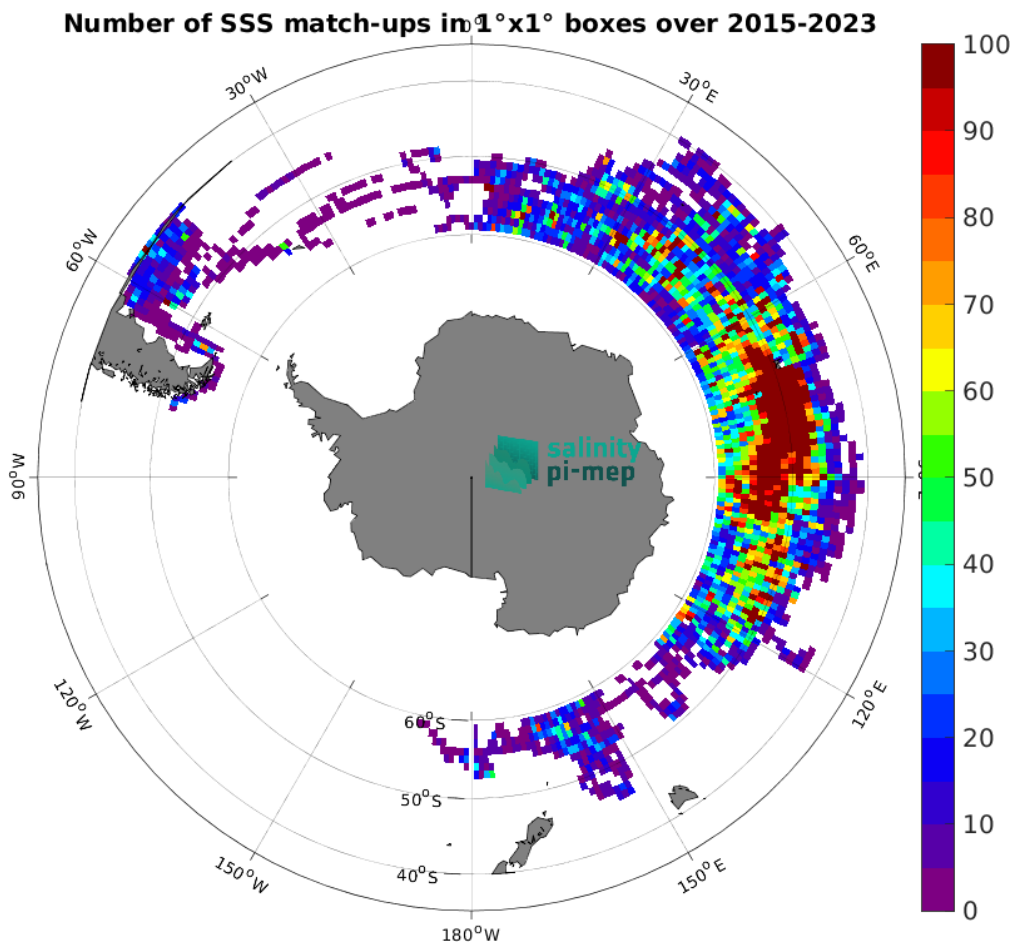
Figure 5: Number of SSS match-ups between Marine mammals SSS and the SMAP SSS L3 v5.3 - Monthly (RSS) SSS product for the Roaring Forties and Furious Fifties Pi-MEP region over 1^\circ \times 1^\circ boxes and for the full satellite product period.
