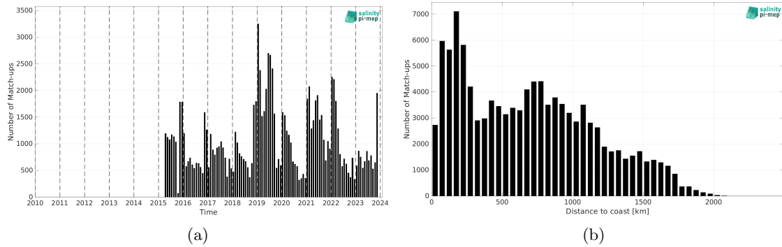
Figure 2: Number of match-ups between Marine mammals and SMAP SSS L3 v5.3 - Monthly (RSS) SSS as a function of time (a) and as function of the distance to coast (b) over the Roaring Forties and Furious Fifties Pi-MEP region and for the full satellite product period.
