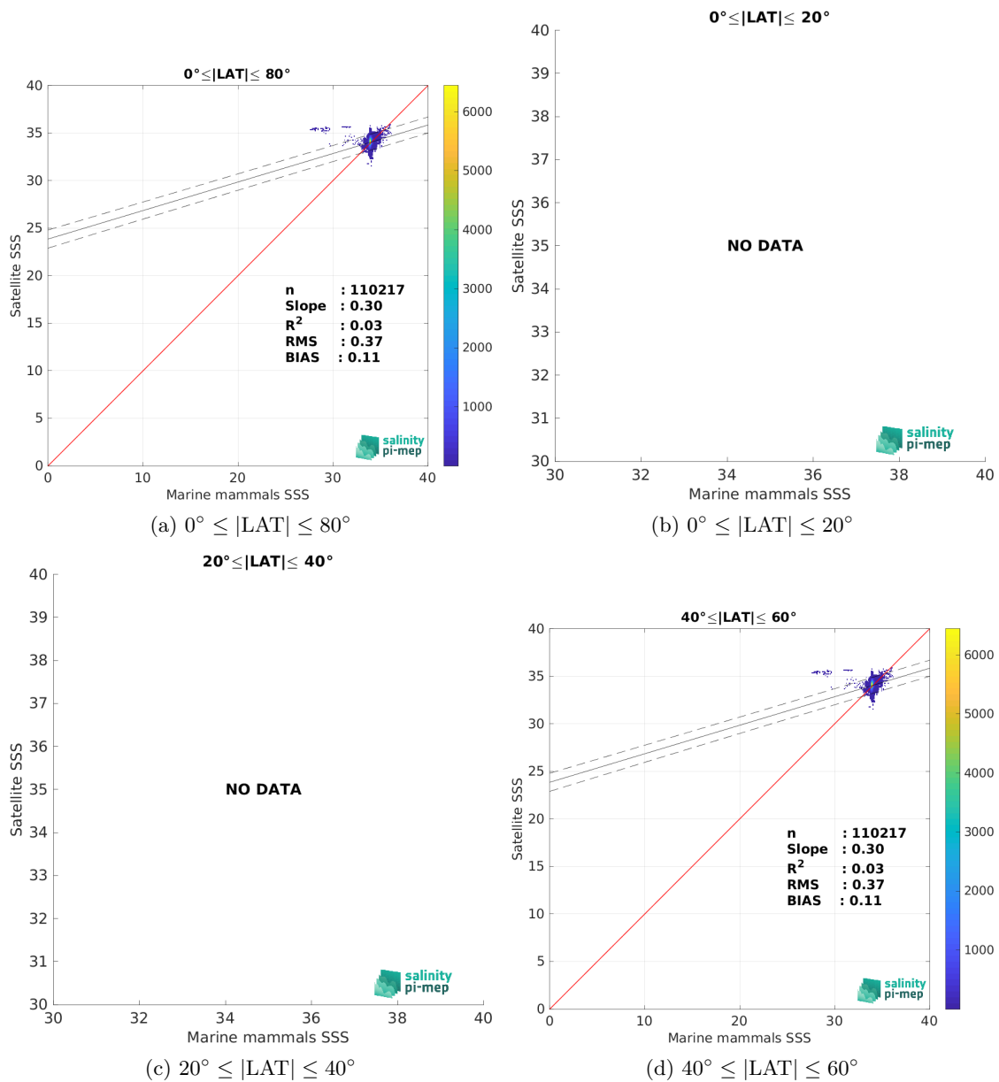
Figure 10: Contour maps of the concentration of SMAP SSS L3 v5.3 - Monthly (RSS) SSS (y-axis) versus Marine mammals SSS (x-axis) at match-up pairs for different latitude bands. For each plot, the red line shows x=y . The black thin and dashed lines indicate a linear fit through the data cloud and the \pm 95\% confidence levels, respectively. The number match-up pairs n , the slope and R^2 coefficient of the linear fit, the root mean square (RMS) and the mean bias between satellite and in situ data are indicated for each latitude band in each plots.
