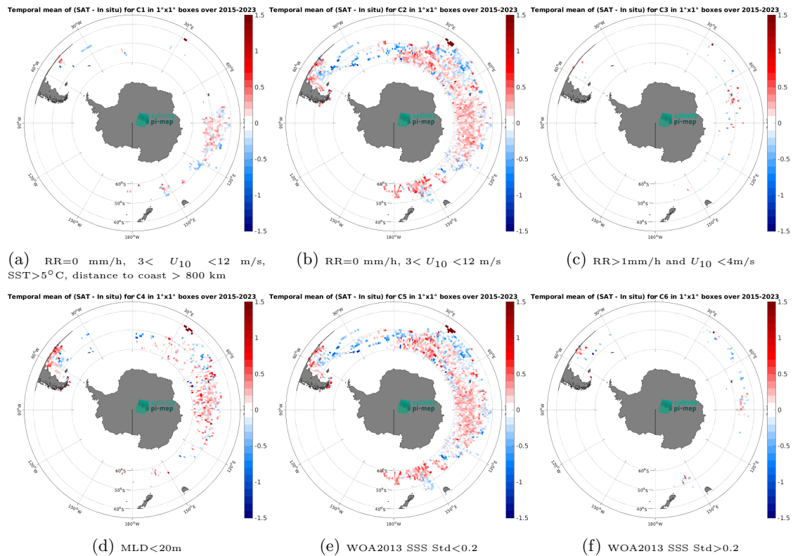
Figure 14: Temporal mean gridded over spatial boxes of size 1^\circ \times 1^\circ of \Delta SSS (SMAP SSS L3 v5.3 - Monthly (RSS) - Marine mammals) for 6 different subdatasets corresponding to:RR=0 mm/h, 3 < U_{10} < 12 m/s, SST>5°C, distance to coast > 800 km (a), RR=0 mm/h, 3 < U_{10} < 12 m/s (b), RR>1mm/h and U_{10} < 4 m/s (c),MLD<20m (d),WOA2013 SSS Std<0.2 (e),WOA2013 SSS Std>0.2 (f).
