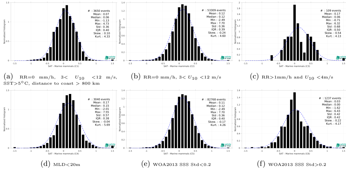
Figure 15: Normalized histogram of \Delta SSS (SMAP SSS L3 v5.3 - Monthly (RSS) - Marine mammals) for 6 different subdatasets corresponding to: RR=0 mm/h, 3 < U_{10} < 12 m/s, SST > 5°C, distance to coast > 800 km (a), RR=0 mm/h, 3 < U_{10} < 12 m/s (b), RR > 1mm/h and U_{10} < 4 m/s (c), MLD < 20m (d), WOA2013 SSS Std < 0.2 (e), WOA2013 SSS Std > 0.2 (f).
