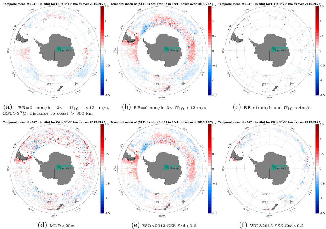
Figure 14: Temporal mean gridded over spatial boxes of size 1^\circ \times 1^\circ of \Delta SSS (SMAP SSS L3 v5.3 - Monthly (RSS) - Argo) for 6 different subdatasets corresponding to:RR=0 mm/h, 3 < U_{10} < 12 m/s, SST >5^\circ C, distance to coast > 800 km (a), RR=0 mm/h, 3 < U_{10} < 12 m/s (b), RR >1 mm/h and U_{10} < 4 m/s (c),MLD <20 m (d),WOA2013 SSS Std <0.2 (e),WOA2013 SSS Std >0.2 (f).
