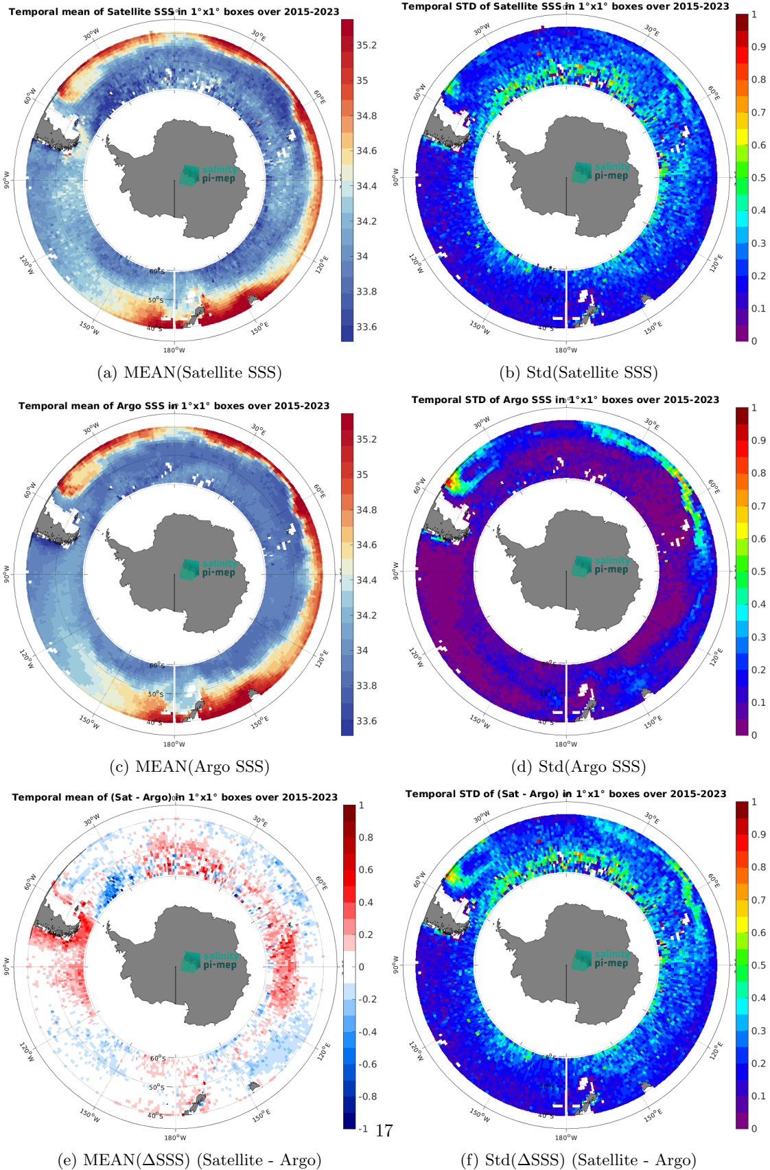
Figure 7: Temporal mean (left) and Std (right) of SSS from SMAP SSS L3 v5.3 - Monthly (RSS) (top), Argo (middle), and of \Delta SSS (Satellite - Argo). Only match-up pairs are used to generate these maps.
