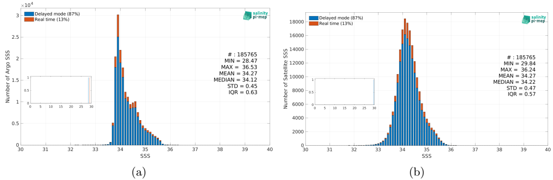
Figure 3: Histograms of SSS from Argo (a) and SMAP SSS L3 v5.3 - Monthly (RSS) (b) considering all match-up pairs per bins of 0.1 over the Roaring Forties and Furious Fifties Pi-MEP region and for the full satellite product period.
