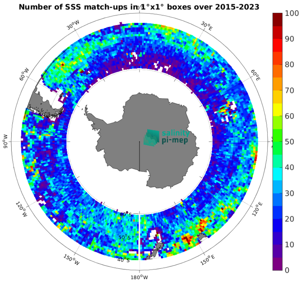
Figure 5: Number of SSS match-ups between Argo SSS and the SMAP SSS L3 v5.3 - Monthly (RSS) SSS product for the Roaring Forties and Furious Fifties Pi-MEP region over 1^\circ \times 1^\circ boxes and for the full satellite product period.
