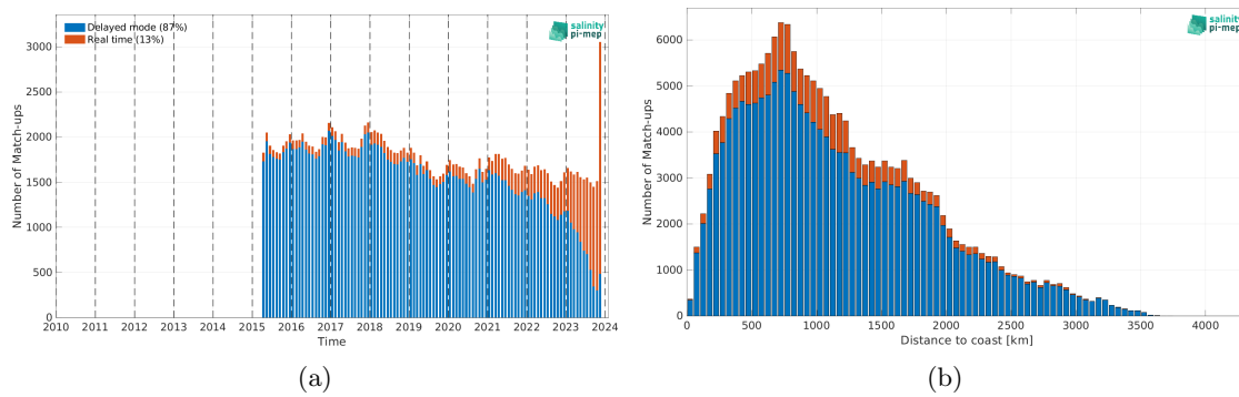
Figure 2: Number of match-ups between Argo and SMAP SSS L3 v5.3 - Monthly (RSS) SSS as a function of time (a) and as function of the distance to coast (b) over the Roaring Forties and Furious Fifties Pi-MEP region and for the full satellite product period.
