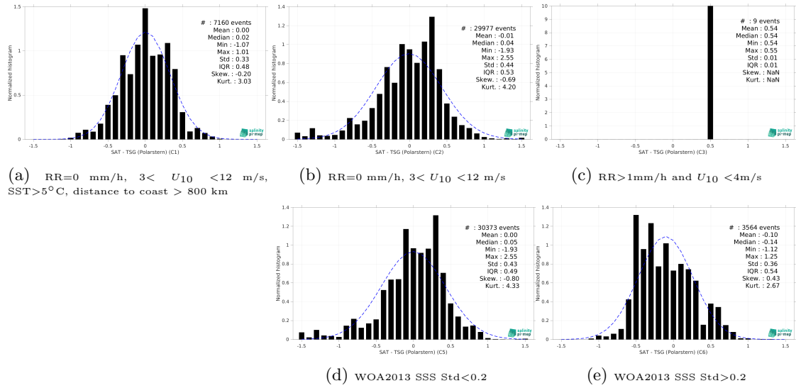
Figure 13: Normalized histogram of \Delta\text{SSS} (SMAP SSS L3 v5 - 8-Day running (RSS) - TSG (Polarstern)) for 5 different subdatasets corresponding to: RR=0 mm/h, 3 < U_{10} < 12 m/s, SST>5°C, distance to coast > 800 km (a), RR=0 mm/h, 3 < U_{10} < 12 m/s (b), RR>1mm/h and U_{10} < 4 m/s (c), WOA2013 SSS Std<0.2 (d), WOA2013 SSS Std>0.2 (e).
