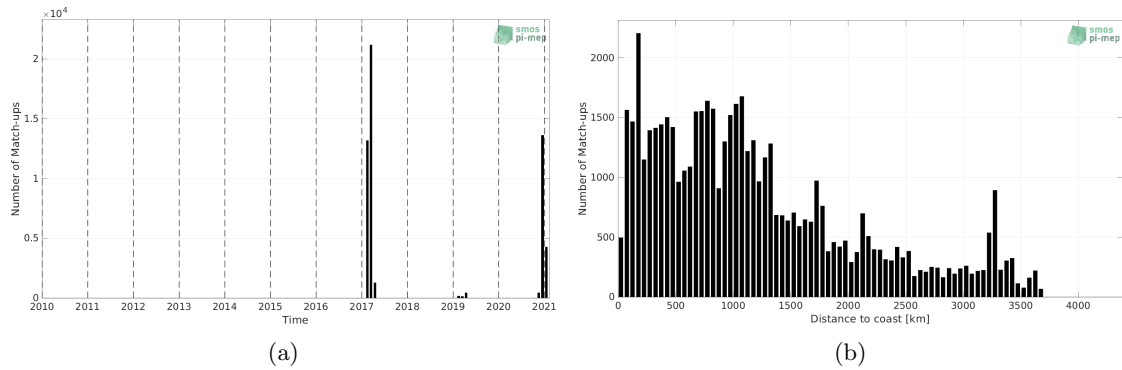
Figure 1: Number of match-ups between TSG (GOSUD-Sailing-ship) and SMAP SSS L3 v5 - 8-Day running (RSS) SSS as a function of time (a) and as function of the distance to coast (b) over the Roaring Forties and Furious Fifties Pi-MEP region and for the full satellite product period.
