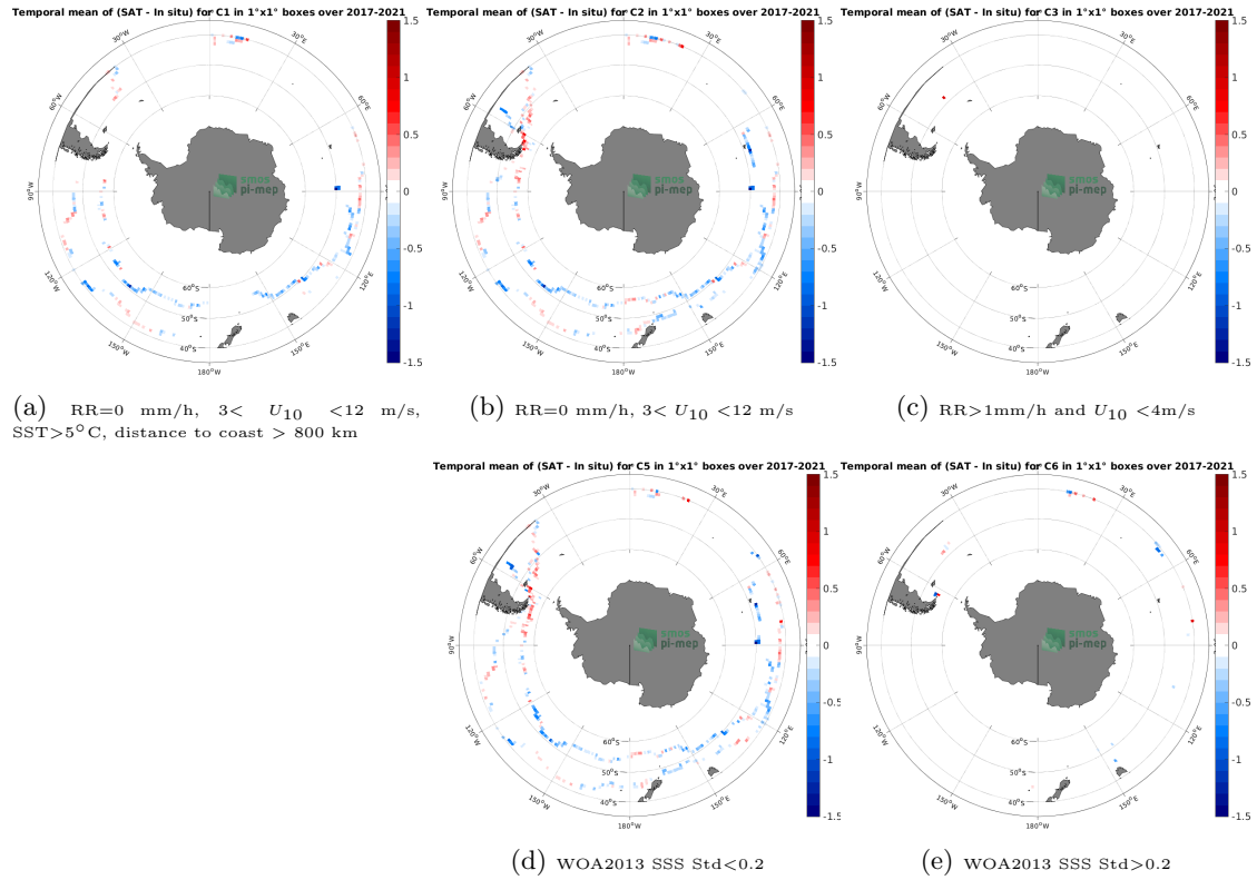
Figure 12: Temporal mean gridded over spatial boxes of size 1^\circ \times 1^\circ of \Delta\text{SSS} (SMAP SSS L3 v5 - 8-Day running (RSS) - TSG (GOSUD-Sailing-ship)) for 5 different subdatasets corresponding to: RR=0 mm/h, 3 < U_{10} < 12 m/s, SST > 5^\circ\text{C} , distance to coast > 800 km (a), RR=0 mm/h, 3 < U_{10} < 12 m/s (b), RR > 1 mm/h and U_{10} < 4 m/s (c), WOA2013 SSS Std < 0.2 (d), WOA2013 SSS Std > 0.2 (e).
