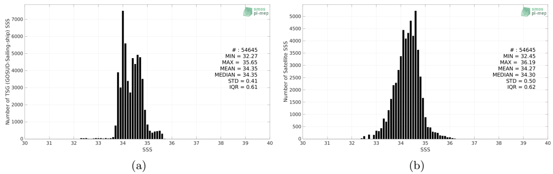
Figure 2: Histograms of SSS from TSG (GOSUD-Sailing-ship) (a) and SMAP SSS L3 v5 - 8-Day running (RSS) (b) considering all match-up pairs per bins of 0.1 over the Roaring Forties and Furious Fifties Pi-MEP region and for the full satellite product period.
