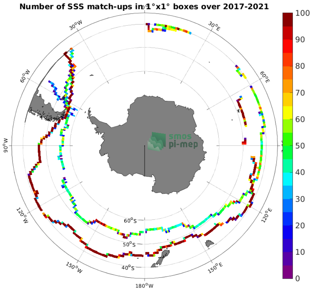
Figure 4: Number of SSS match-ups between TSG (GOSUD-Sailing-ship) SSS and the SMAP SSS L3 v5 - 8-Day running (RSS) SSS product for the Roaring Forties and Furious Fifties Pi-MEP region over 1^\circ \times 1^\circ boxes and for the full satellite product period.
