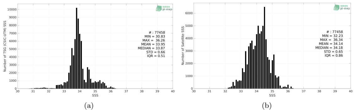
Figure 2: Histograms of SSS from TSG (CSIC-UTM) (a) and SMAP SSS L3 v5 - 8-Day running (RSS) (b) considering all match-up pairs per bins of 0.1 over the Roaring Forties and Furious Fifties Pi-MEP region and for the full satellite product period.
