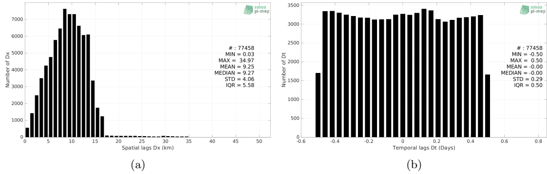
Figure 5: Histograms of the spatial (a) and temporal (b) lags between the location/time of the TSG (CSIC-UTM) measurement and the date of the corresponding SMAP SSS L3 v5 - 8-Day running (RSS) SSS pixel.
