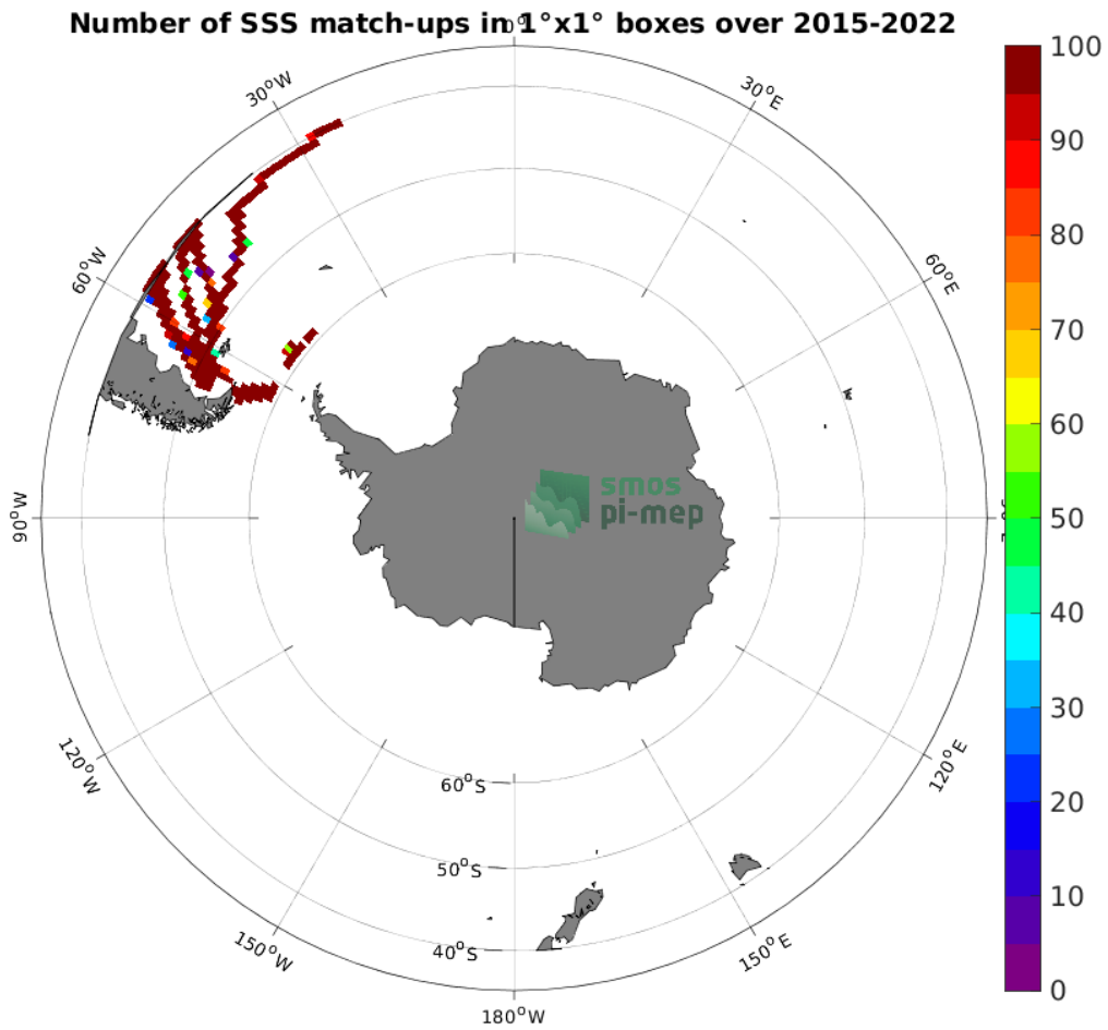
Figure 4: Number of SSS match-ups between TSG (CSIC-UTM) SSS and the SMAP SSS L3 v5 - 8-Day running (RSS) SSS product for the Roaring Forties and Furious Fifties Pi-MEP region over 1^\circ \times 1^\circ boxes and for the full satellite product period.
