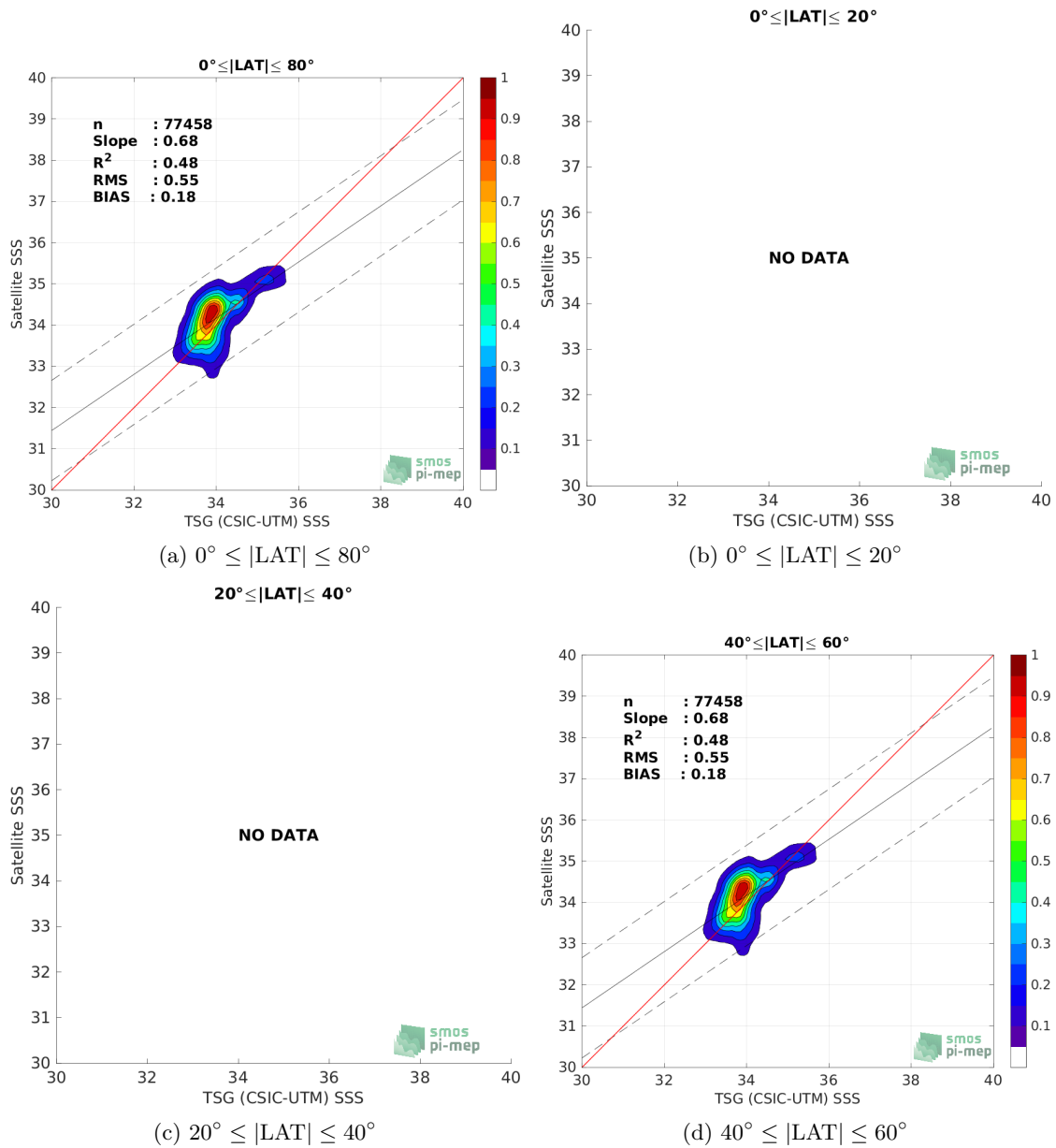
Figure 9: Contour maps of the concentration of SMAP SSS L3 v5 - 8-Day running (RSS) SSS (y-axis) versus TSG (CSIC-UTM) SSS (x-axis) at match-up pairs for different latitude bands. For each plot, the red line shows x=y . The black thin and dashed lines indicate a linear fit through the data cloud and the \pm 95\% confidence levels, respectively. The number match-up pairs n , the slope and R^2 coefficient of the linear fit, the root mean square (RMS) and the mean bias between satellite and in situ data are indicated for each latitude band in each plot.
