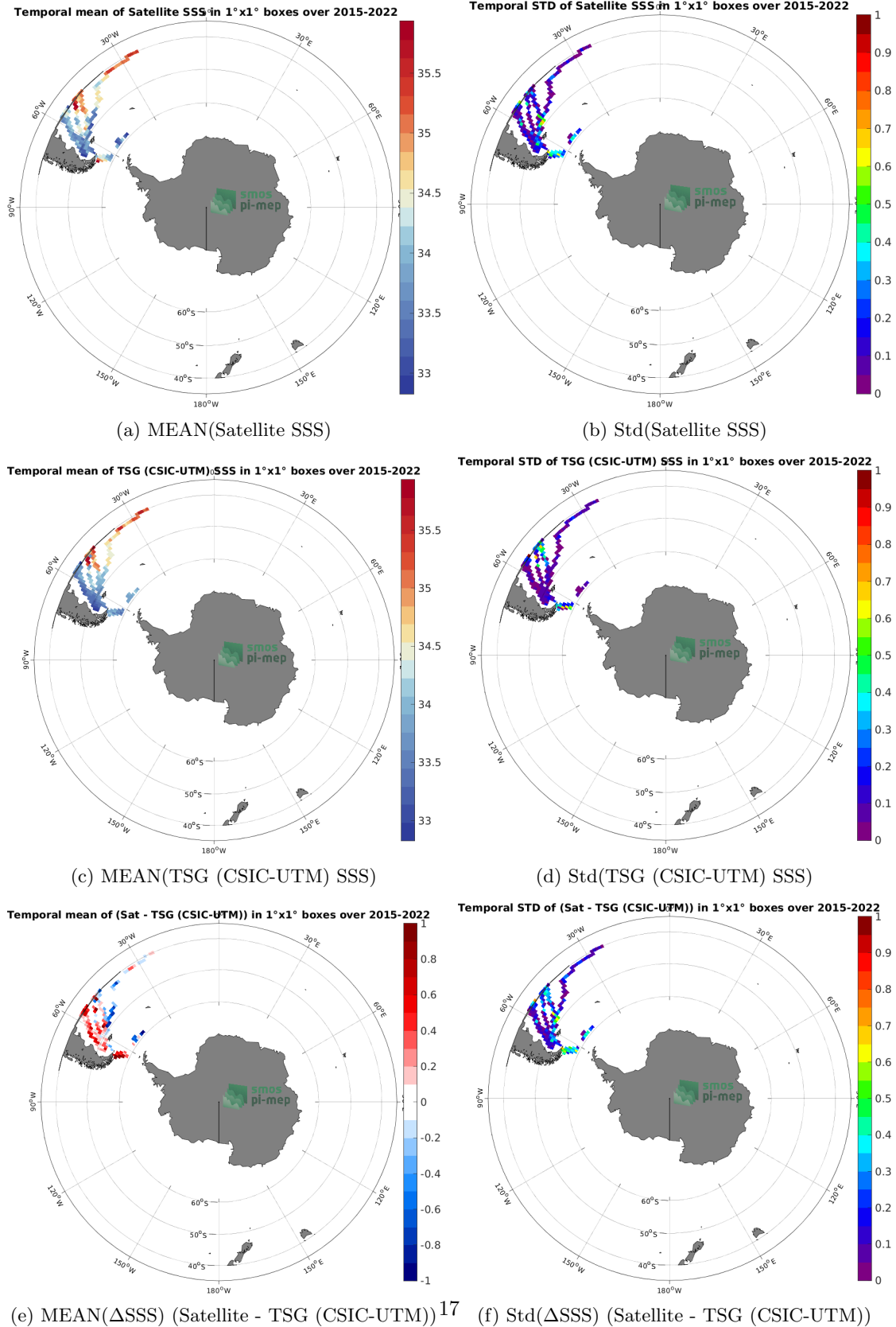
Figure 6: Temporal mean (left) and Std (right) of SSS from SMAP SSS L3 v5 - 8-Day running (RSS) (top), TSG (CSIC-UTM) (middle), and of \Delta SSS (Satellite - TSG (CSIC-UTM)). Only match-up pairs are used to generate these maps.
