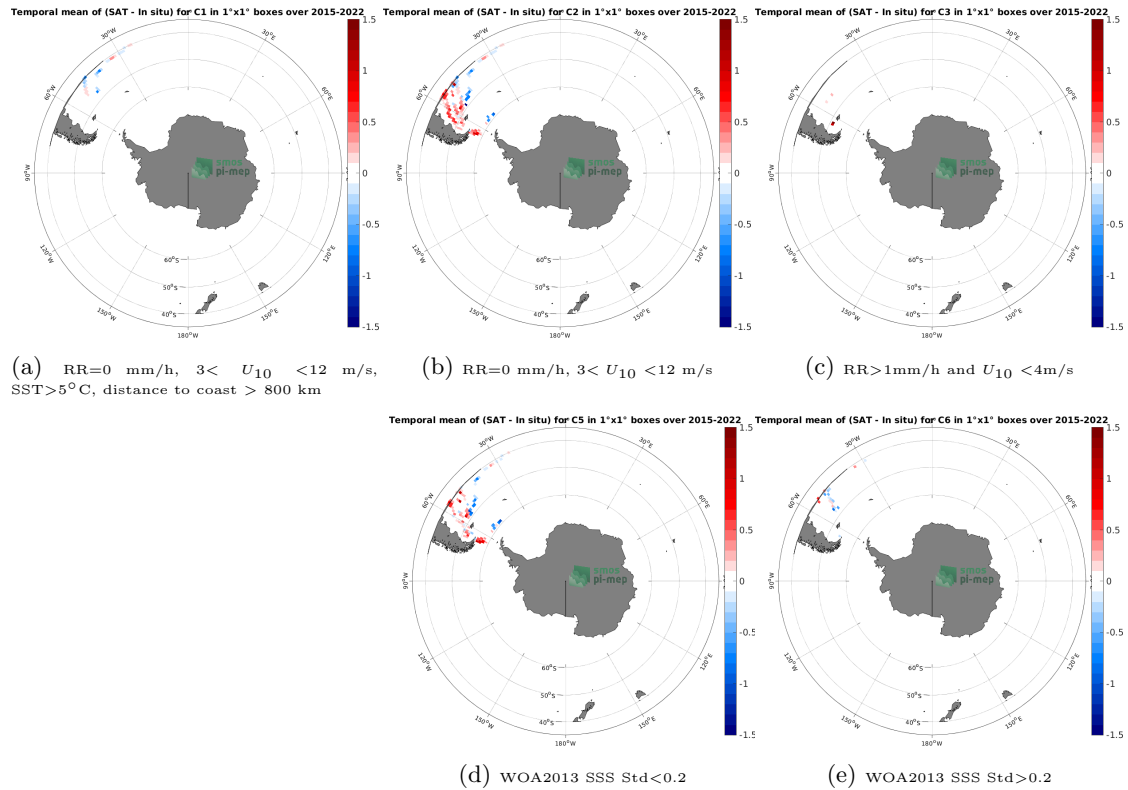
Figure 12: Temporal mean gridded over spatial boxes of size 1^{\circ}\times 1^{\circ} of \Delta\text{SSS} (SMAP SSS L3 v5 - 8-Day running (RSS) - TSG (CSIC-UTM)) for 5 different subdatasets corresponding to:RR=0 mm/h, 3 < U_{10} < 12 m/s, SST >5^{\circ}\text{C} , distance to coast > 800 km (a), RR=0 mm/h, 3 < U_{10} < 12 m/s (b), RR >1 mm/h and U_{10} < 4 m/s (c), WOA2013 SSS Std <0.2 (d), WOA2013 SSS Std >0.2 (e).
