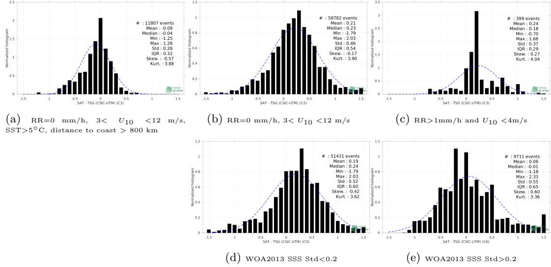
Figure 13: Normalized histogram of \Delta SSS (SMAP SSS L3 v5 - 8-Day running (RSS) - TSG (CSIC-UTM)) for 5 different subdatasets corresponding to: RR=0 mm/h, 3 < U_{10} < 12 m/s, SST>5°C, distance to coast > 800 km (a), RR=0 mm/h, 3 < U_{10} < 12 m/s (b), RR>1mm/h and U_{10} < 4 m/s (c), WOA2013 SSS Std<0.2 (d), WOA2013 SSS Std>0.2 (e).
