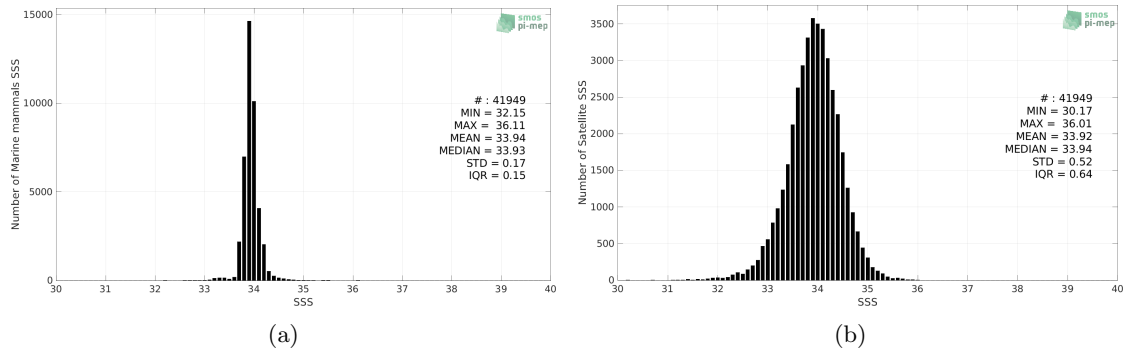
Figure 2: Histograms of SSS from Marine mammals (a) and SMAP SSS L3 v5 - 8-Day running (RSS) (b) considering all match-up pairs per bins of 0.1 over the Roaring Forties and Furious Fifties Pi-MEP region and for the full satellite product period.
