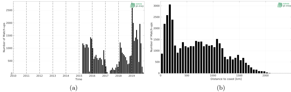
Figure 1: Number of match-ups between Marine mammals and SMAP SSS L3 v5 - 8-Day running (RSS) SSS as a function of time (a) and as function of the distance to coast (b) over the Roaring Forties and Furious Fifties Pi-MEP region and for the full satellite product period.
