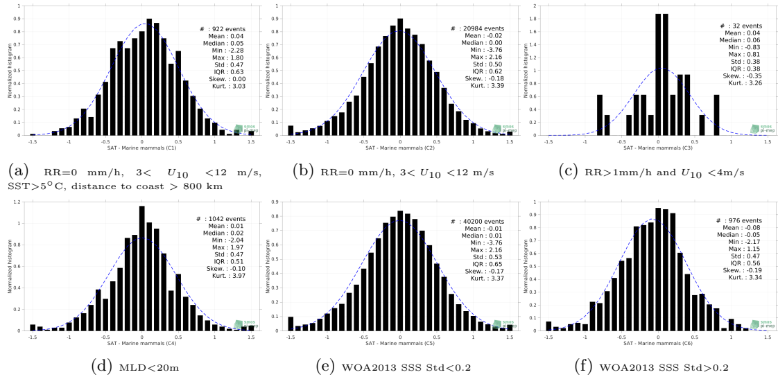
Figure 13: Normalized histogram of \Delta\text{SSS} (SMAP SSS L3 v5 - 8-Day running (RSS) - Marine mammals) for 6 different subdatasets corresponding to: RR=0 mm/h, 3 < U_{10} < 12 m/s, SST>5°C, distance to coast > 800 km (a), RR=0 mm/h, 3 < U_{10} < 12 m/s (b), RR>1mm/h and U_{10} < 4 m/s (c), MLD<20m (d), WOA2013 SSS Std<0.2 (e), WOA2013 SSS Std>0.2 (f).
