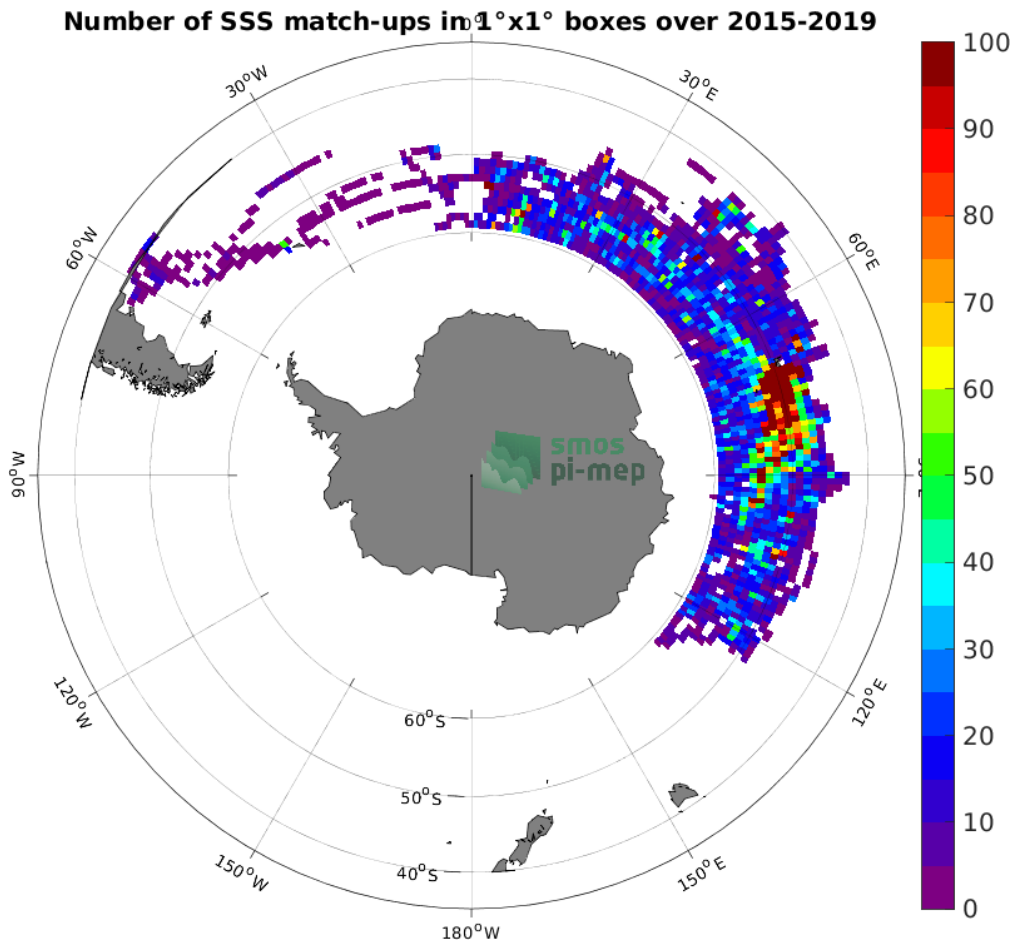
Figure 4: Number of SSS match-ups between Marine mammals SSS and the SMAP SSS L3 v5 - 8-Day running (RSS) SSS product for the Roaring Forties and Furious Fifties Pi-MEP region over 1^\circ \times 1^\circ boxes and for the full satellite product period.
